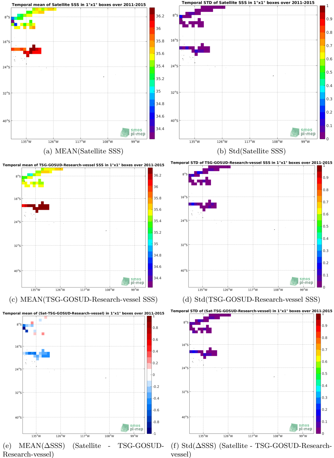
Figure 6: Temporal mean (left) and Std (right) of SSS from Aquarius-L3-OR-V5-7DAY-RUNNING-RAIN-MASK-1DEG (top), TSG-GOSUD-Research-vessel (middle), and of \Delta SSS (Satellite - TSG-GOSUD-Research-vessel). Only match-up pairs are used to generate these maps.
