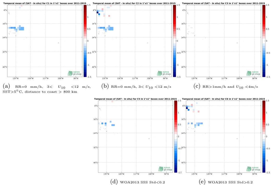
Figure 12: Temporal mean gridded over spatial boxes of size 1^\circ \times 1^\circ of \Delta SSS (Aquarius-L3-OR-V5-7DAY-RUNNING-RAIN-MASK-1DEG - TSG-GOSUD-Research-vessel) for 5 different subdatasets corresponding to:RR=0 mm/h, 3 < U_{10} < 12 m/s, SST >5^\circ C, distance to coast > 800 km (a), RR=0 mm/h, 3 < U_{10} < 12 m/s (b), RR >1 mm/h and U_{10} < 4 m/s (c), WOA2013 SSS Std <0.2 (d), WOA2013 SSS Std >0.2 (e).
