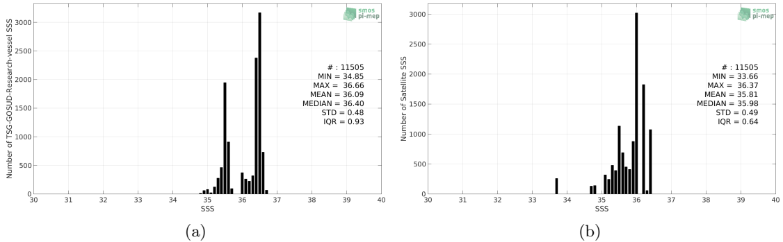
Figure 2: Histograms of SSS from TSG-GOSUD-Research-vessel (a) and Aquarius-L3-OR-V5-7DAY-RUNNING-RAIN-MASK-1DEG (b) considering all match-up pairs per bins of 0.1 over the OTT zone Pi-MEP region and for the full satellite product period.
