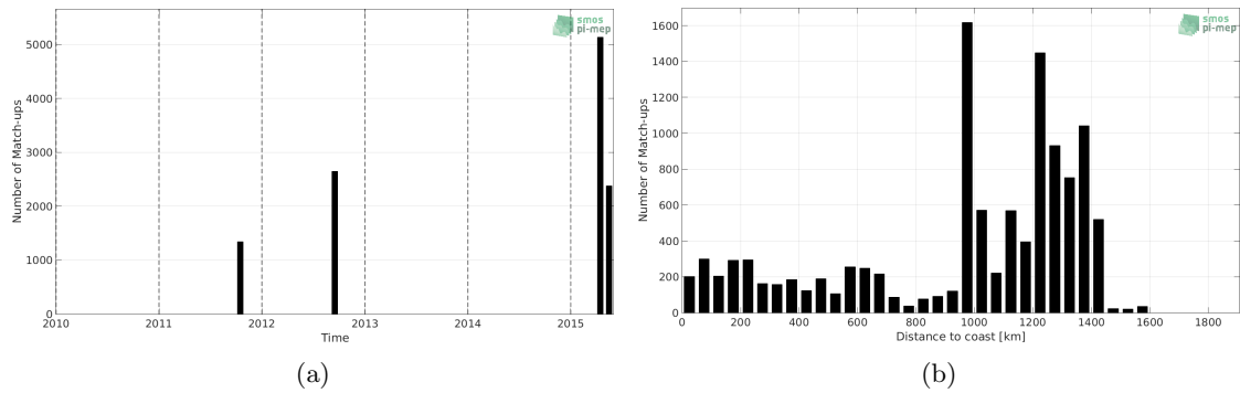
Figure 1: Number of match-ups between TSG-GOSUD-Research-vessel and Aquarius-L3-OR-V5-7DAY-RUNNING-RAIN-MASK-1DEG SSS as a function of time (a) and as function of the distance to coast (b) over the OTT zone Pi-MEP region and for the full satellite product period.
