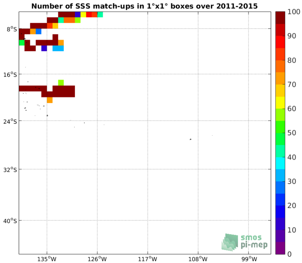
Figure 4: Number of SSS match-ups between TSG-GOSUD-Research-vessel SSS and the Aquarius-L3-OR-V5-7DAY-RUNNING-RAIN-MASK-1DEG SSS product for the OTT zone Pi-MEP region over 1°x1° boxes and for the full satellite product period.
