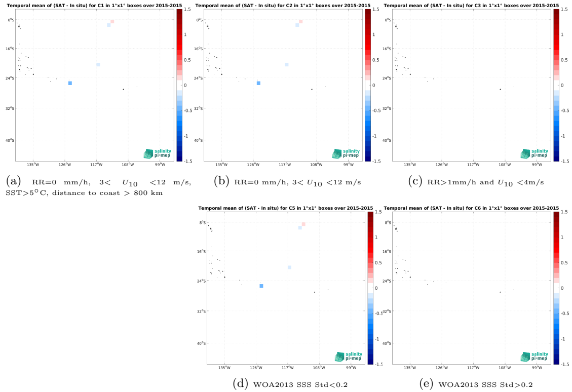
Figure 13: Temporal mean gridded over spatial boxes of size 1^\circ \times 1^\circ of \Delta SSS (Aquarius SSS L3 OR v5 - 7-Day running - Rain mask (NASA-GSFC) - Surface drifters) for 5 different subdatasets corresponding to:RR=0 mm/h, 3 < U_{10} < 12 m/s, SST >5^\circ C, distance to coast > 800 km (a), RR=0 mm/h, 3 < U_{10} < 12 m/s (b), RR >1 mm/h and U_{10} < 4 m/s (c), WOA2013 SSS Std <0.2 (d), WOA2013 SSS Std >0.2 (e).
