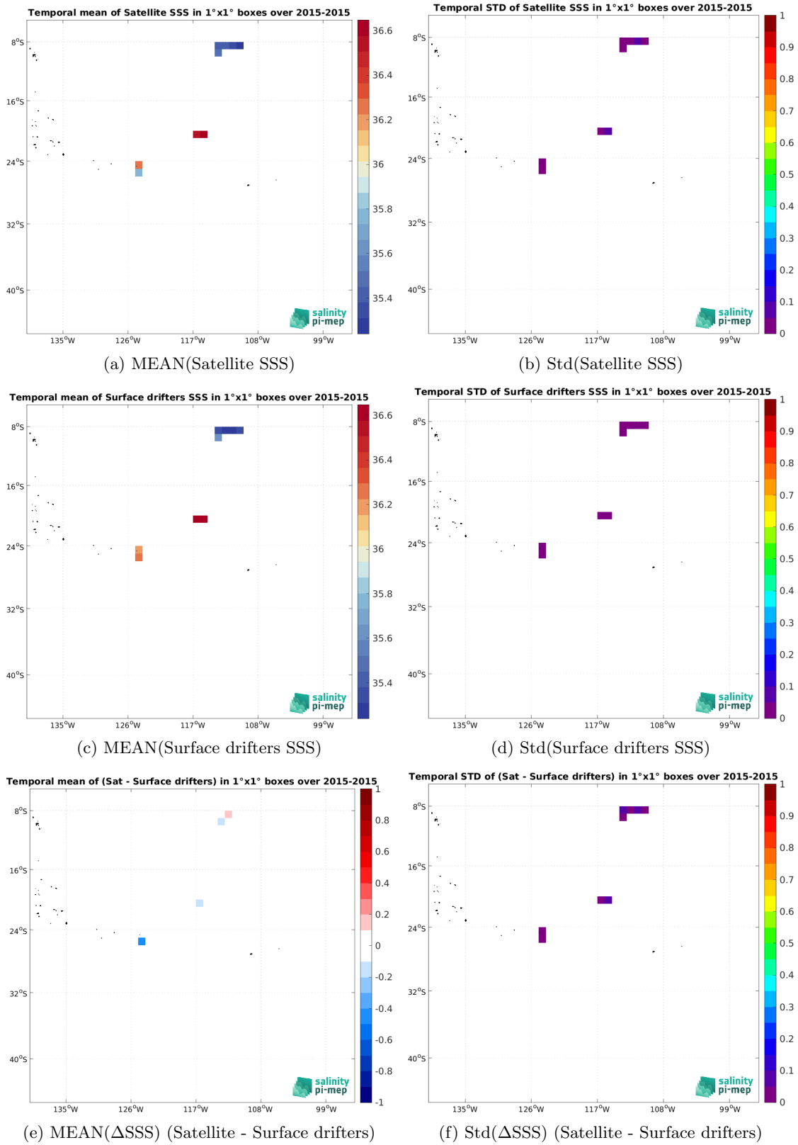
Figure 6: Temporal mean (left) and Std (right) of SSS from Aquarius SSS L3 OR v5 - 7-Day running - Rain mask (NASA-GSFC) (top), Surface drifters (middle), and of \Delta SSS (Satellite - Surface drifters). Only match-up pairs are used to generate these maps.
