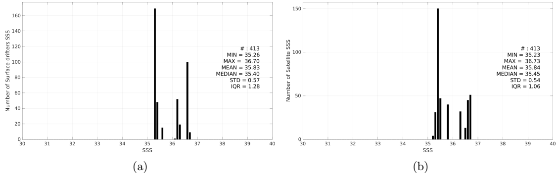
Figure 3: Histograms of SSS from Surface drifters (a) and Aquarius SSS L3 OR v5 - 7-Day running - Rain mask (NASA-GSFC) (b) considering all match-up pairs per bins of 0.1 over the OTT zone Pi-MEP region and for the full satellite product period.
