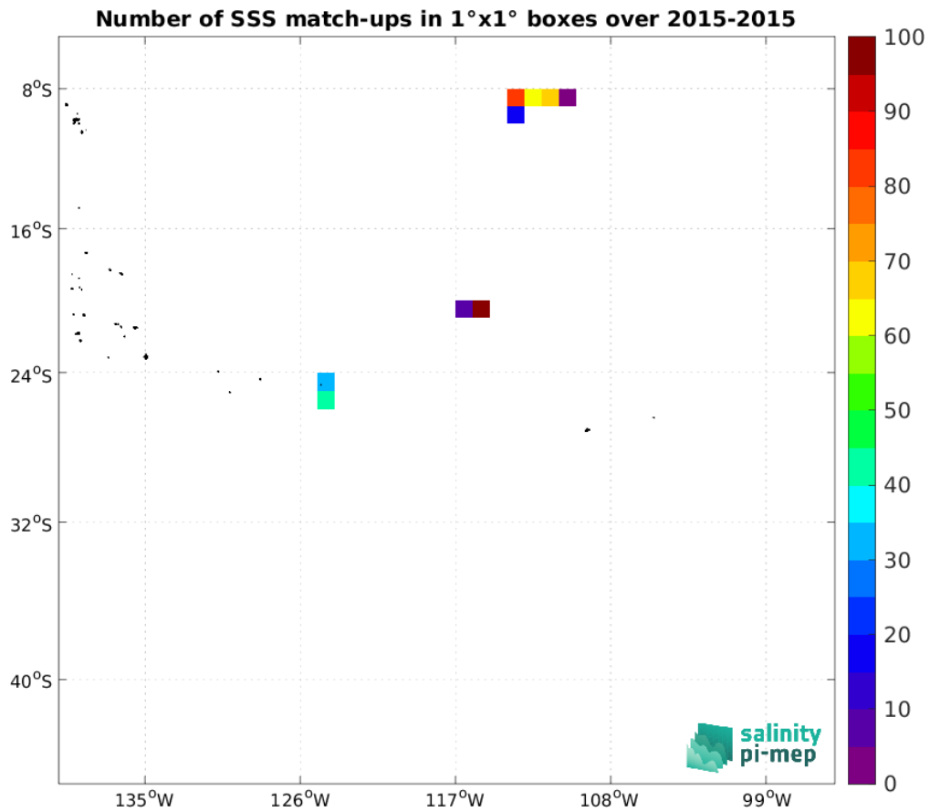
Figure 4: Number of SSS match-ups between Surface drifters SSS and the Aquarius SSS L3 OR v5 - 7-Day running - Rain mask (NASA-GSFC) SSS product for the OTT zone Pi-MEP region over 1°x1° boxes and for the full satellite product period.
