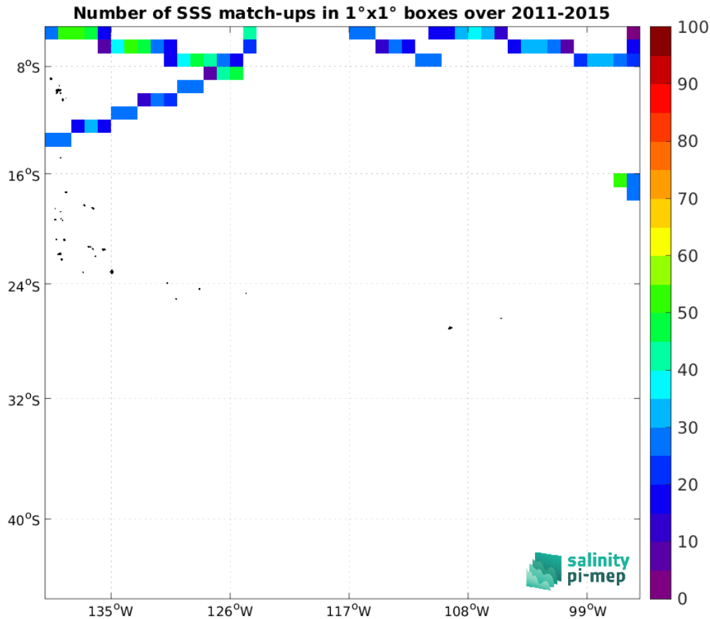
Figure 5: Number of SSS match-ups between TSG (SAMOS) SSS and the Aquarius SSS L3 OR v5 - Monthly (NASA-GSFC) SSS product for the OTT zone Pi-MEP region over 1^\circ \times 1^\circ boxes and for the full satellite product period.
