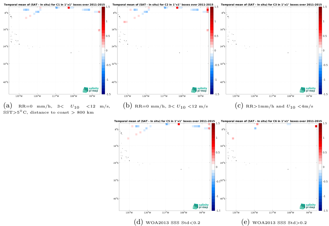
Figure 14: Temporal mean gridded over spatial boxes of size 1^\circ \times 1^\circ of \Delta SSS (Aquarius SSS L3 OR v5 - Monthly (NASA-GSFC) - TSG (SAMOS)) for 5 different subdatasets corresponding to:RR=0 mm/h, 3 < U_{10} < 12 m/s, SST>5°C, distance to coast > 800 km (a), RR=0 mm/h, 3 < U_{10} < 12 m/s (b), RR>1mm/h and U_{10} < 4 m/s (c), WOA2013 SSS Std<0.2 (d), WOA2013 SSS Std>0.2 (e).
