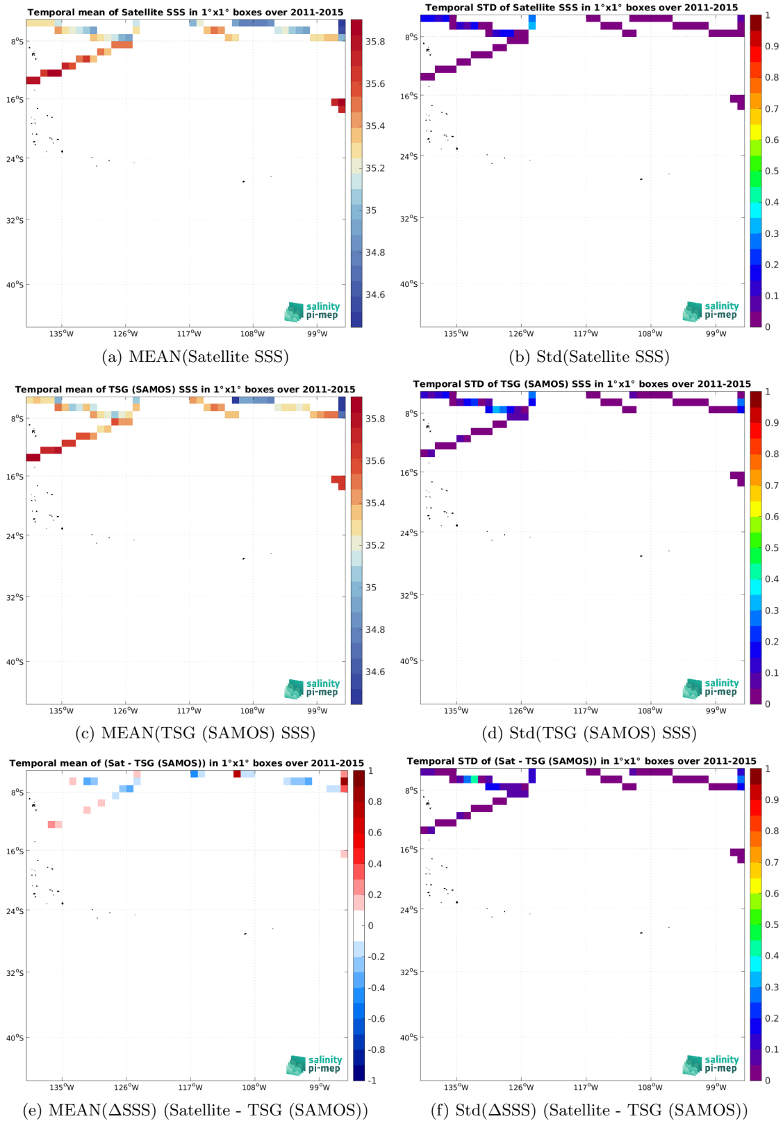
Figure 7: Temporal mean (left) and Std (right) of SSS from Aquarius SSS L3 OR v5 - Monthly (NASA-GSFC) (top), TSG (SAMOS) (middle), and of \Delta SSS (Satellite - TSG (SAMOS)). Only match-up pairs are used to generate these maps.
