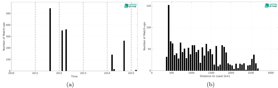
Figure 2: Number of match-ups between TSG (SAMOS) and Aquarius SSS L3 OR v5 - Monthly (NASA-GSFC) SSS as a function of time (a) and as function of the distance to coast (b) over the OTT zone Pi-MEP region and for the full satellite product period.
