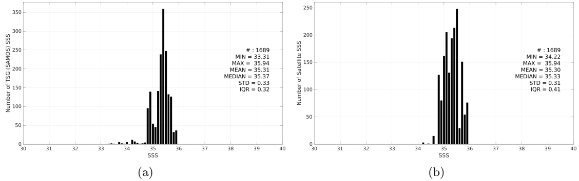
Figure 3: Histograms of SSS from TSG (SAMOS) (a) and Aquarius SSS L3 OR v5 - Monthly (NASA-GSFC) (b) considering all match-up pairs per bins of 0.1 over the OTT zone Pi-MEP region and for the full satellite product period.
