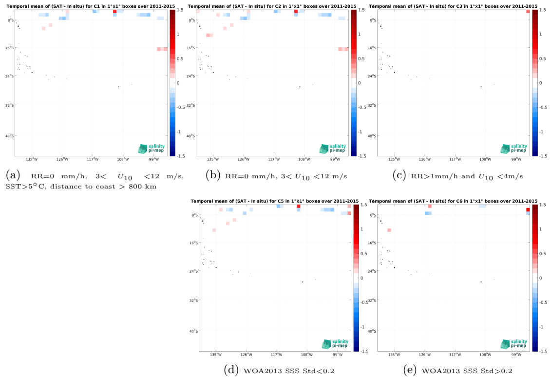
Figure 12: Temporal mean gridded over spatial boxes of size 1^\circ \times 1^\circ of \Delta\text{SSS} (Aquarius SSS L3 OR v5 - Monthly (NASA-GSFC) - TSG (SAMOS)) for 5 different subdatasets corresponding to: \text{RR}=0 mm/h, 3 < U_{10} < 12 m/s, \text{SST} > 5^\circ\text{C} , distance to coast > 800 km (a), \text{RR}=0 mm/h, 3 < U_{10} < 12 m/s (b), \text{RR} > 1 mm/h and U_{10} < 4 m/s (c), WOA2013 SSS Std < 0.2 (d), WOA2013 SSS Std > 0.2 (e).
