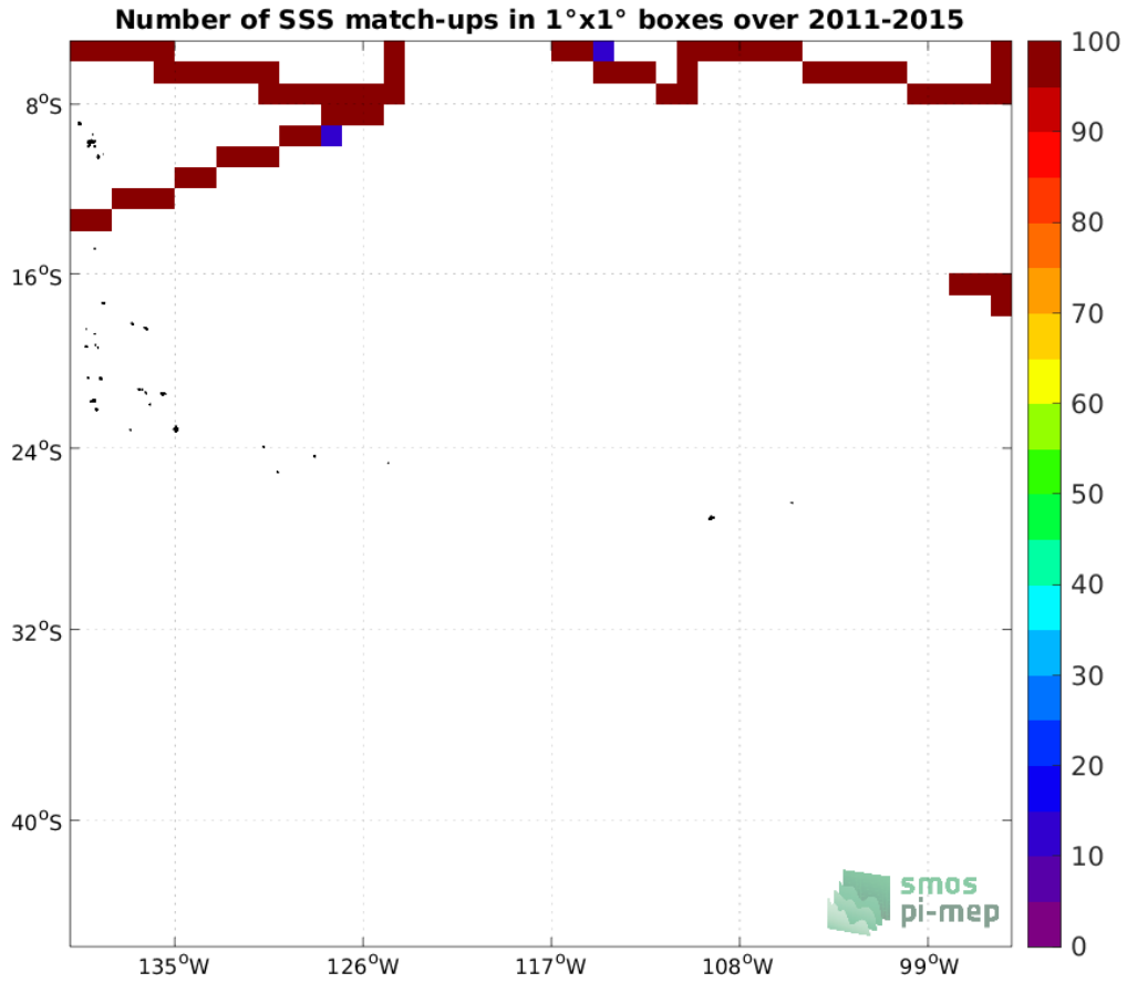
Figure 4: Number of SSS match-ups between TSG (SAMOS) SSS and the Aquarius SSS L3 OR v5 - Monthly (NASA-GSFC) SSS product for the OTT zone Pi-MEP region over 1^{\circ} \times 1^{\circ} boxes and for the full satellite product period.
