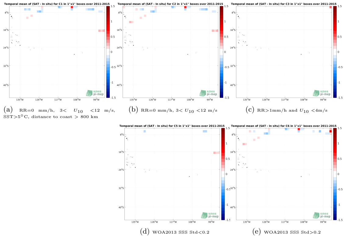
Figure 12: Temporal mean gridded over spatial boxes of size 1^\circ \times 1^\circ of \Delta SSS (Aquarius SSS L3 OR v5 - Monthly (NASA-GSFC) - TSG (SAMOS)) for 5 different subdatasets corresponding to: RR=0 mm/h, 3 < U_{10} < 12 m/s, SST > 5^\circ C , distance to coast > 800 km (a), RR=0 mm/h, 3 < U_{10} < 12 m/s (b), RR > 1 mm/h and U_{10} < 4 m/s (c), WOA2013 SSS Std < 0.2 (d), WOA2013 SSS Std > 0.2 (e).
