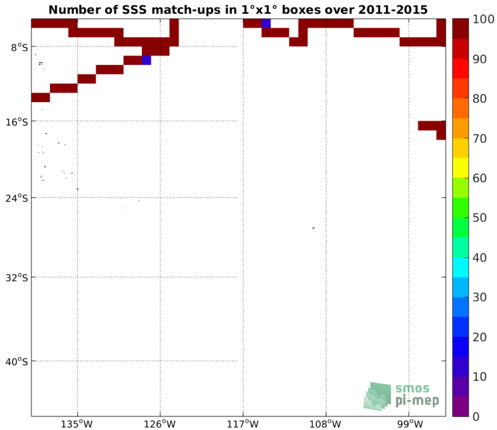
Figure 4: Number of SSS match-ups between TSG (SAMOS) SSS and the Aquarius SSS L3 OR v5 - Monthly (NASA-GSFC) SSS product for the OTT zone Pi-MEP region over 1°x1° boxes and for the full satellite product period.
