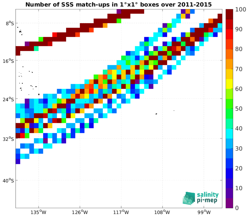
Figure 4: Number of SSS match-ups between TSG (LEGOS-DM) SSS and the Aquarius SSS L3 OR v5 - Monthly (NASA-GSFC) SSS product for the OTT zone Pi-MEP region over 1^\circ \times 1^\circ boxes and for the full satellite product period.
