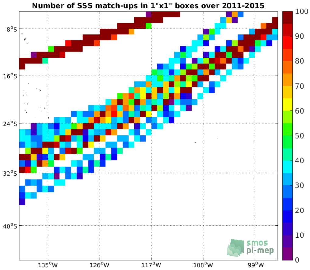
Figure 4: Number of SSS match-ups between TSG-LEGOS-DM SSS and the Aquarius-L3-OR-V5-MONTHLY-1DEG SSS product for the OTT zone Pi-MEP region over 1°x1° boxes and for the full satellite product period.
