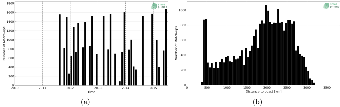
Figure 1: Number of match-ups between TSG-LEGOS-DM and Aquarius-L3-OR-V5-MONTHLY-1DEG SSS as a function of time (a) and as function of the distance to coast (b) over the OTT zone Pi-MEP region and for the full satellite product period.
