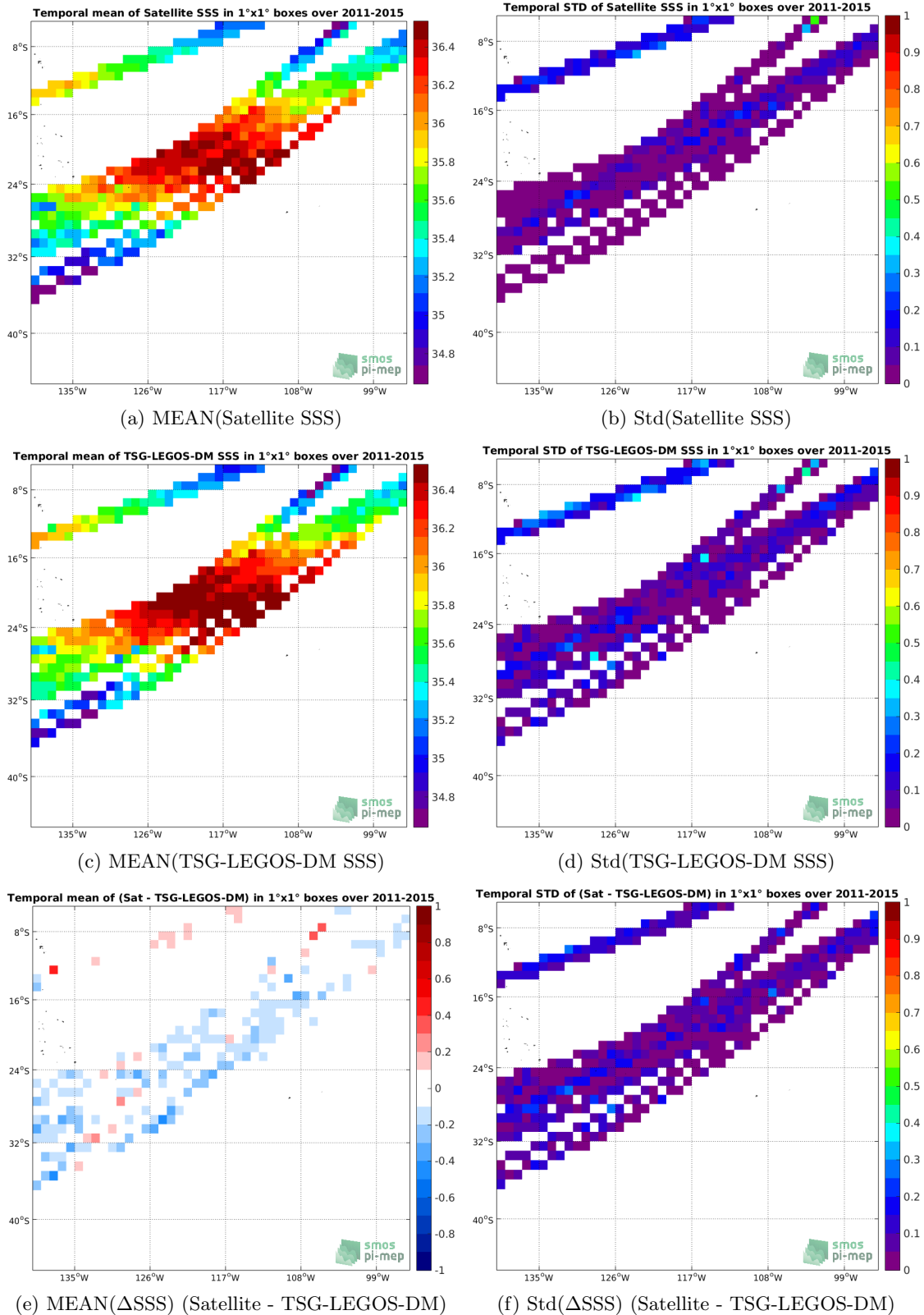
Figure 6: Temporal mean (left) and Std (right) of SSS from Aquarius-L3-OR-V5-MONTHLY-1DEG (top), TSG-LEGOS-DM (middle), and of \Delta SSS (Satellite - TSG-LEGOS-DM). Only match-up pairs are used to generate these maps.
