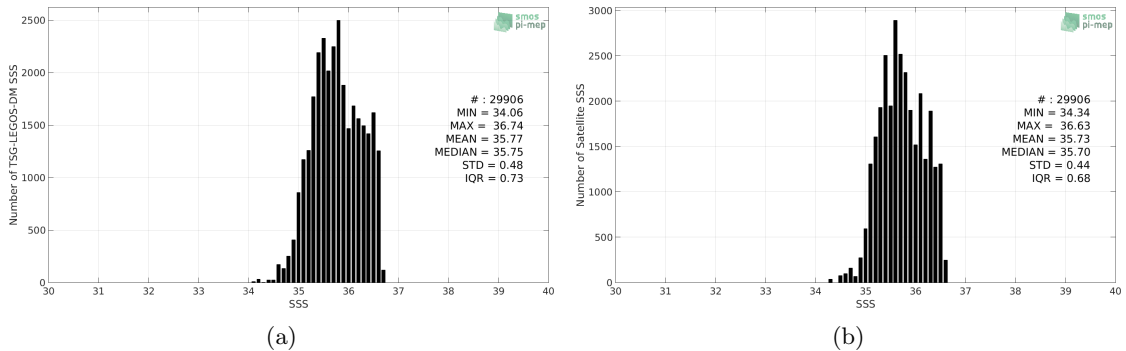
Figure 2: Histograms of SSS from TSG-LEGOS-DM (a) and Aquarius-L3-OR-V5-MONTHLY-1DEG (b) considering all match-up pairs per bins of 0.1 over the OTT zone Pi-MEP region and for the full satellite product period.
