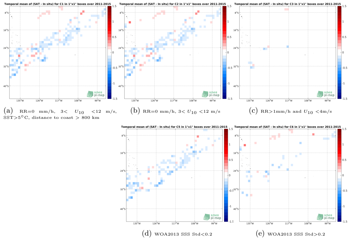
Figure 12: Temporal mean gridded over spatial boxes of size 1^\circ \times 1^\circ of \Delta SSS (Aquarius-L3-OR-V5-MONTHLY-1DEG - TSG-LEGOS-DM) for 5 different subdatasets corresponding to:RR=0 mm/h, 3 < U_{10} < 12 m/s, SST > 5^\circ\text{C} , distance to coast > 800 km (a), RR=0 mm/h, 3 < U_{10} < 12 m/s (b), RR > 1 mm/h and U_{10} < 4 m/s (c), WOA2013 SSS Std < 0.2 (d), WOA2013 SSS Std > 0.2 (e).
