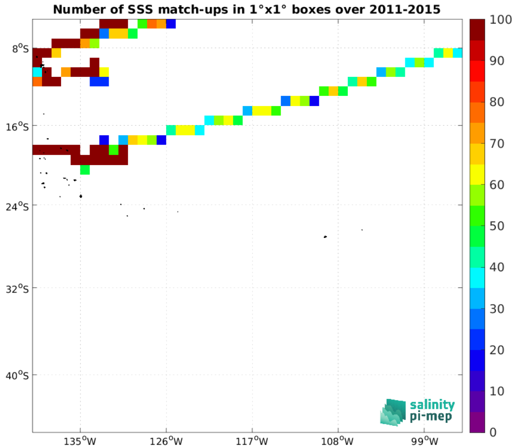
Figure 5: Number of SSS match-ups between TSG (GOSUD-Research-vessel) SSS and the Aquarius SSS L3 OR v5 - Monthly (NASA-GSFC) SSS product for the OTT zone Pi-MEP region over 1^\circ \times 1^\circ boxes and for the full satellite product period.
