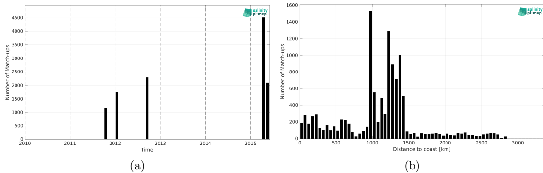
Figure 2: Number of match-ups between TSG (GOSUD-Research-vessel) and Aquarius SSS L3 OR v5 - Monthly (NASA-GSFC) SSS as a function of time (a) and as function of the distance to coast (b) over the OTT zone Pi-MEP region and for the full satellite product period.
