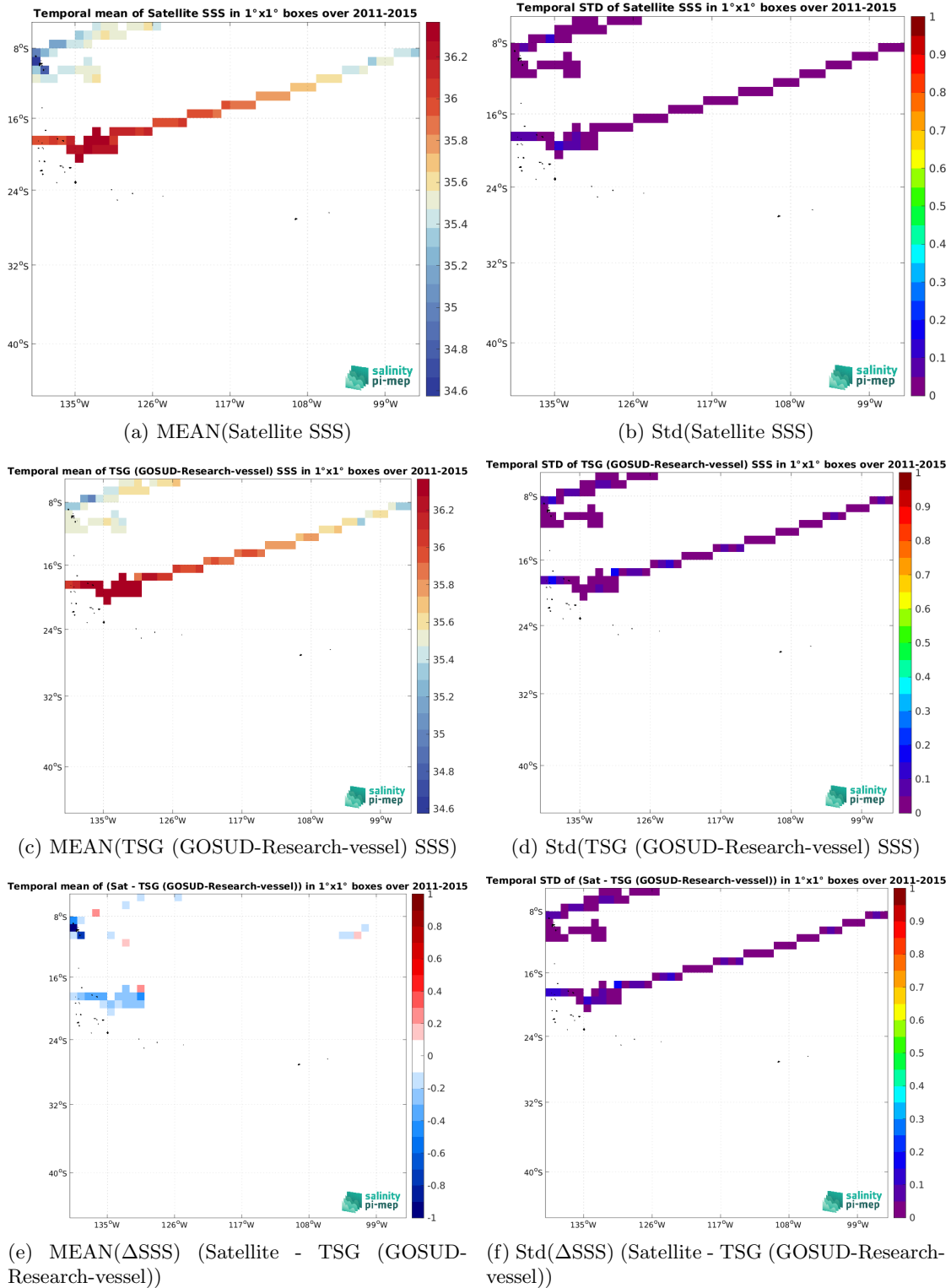
Figure 7: Temporal mean (left) and Std (right) of SSS from Aquarius SSS L3 OR v5 - Monthly (NASA-GSFC) (top), TSG (GOSUD-Research-vessel) (middle), and of \Delta SSS (Satellite - TSG (GOSUD-Research-vessel)). Only match-up pairs are used to generate these maps.
