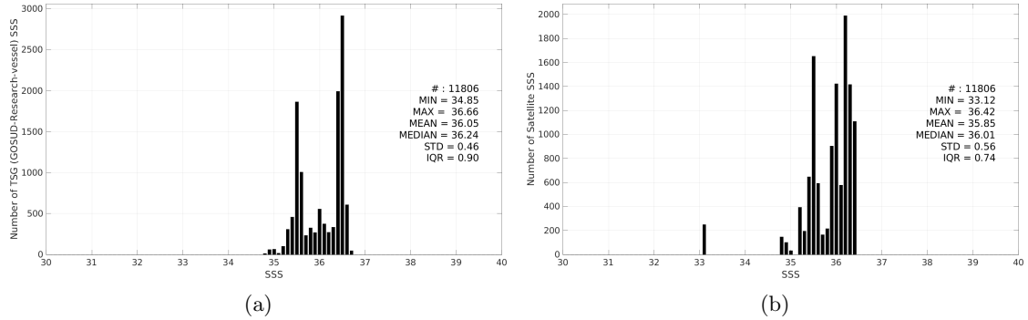
Figure 3: Histograms of SSS from TSG (GOSUD-Research-vessel) (a) and Aquarius SSS L3 OR v5 - Monthly (NASA-GSFC) (b) considering all match-up pairs per bins of 0.1 over the OTT zone Pi-MEP region and for the full satellite product period.
