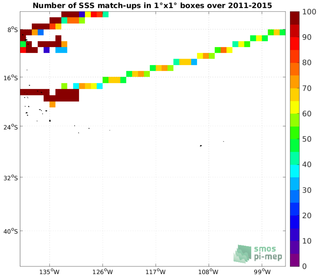
Figure 4: Number of SSS match-ups between TSG (GOSUD-Research-vessel) SSS and the Aquarius SSS L3 OR v5 - Monthly (NASA-GSFC) SSS product for the OTT zone Pi-MEP region over 1°x1° boxes and for the full satellite product period.
