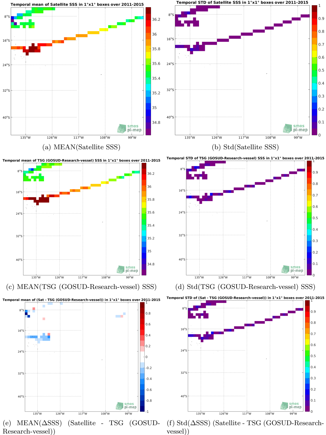
Figure 6: Temporal mean (left) and Std (right) of SSS from Aquarius SSS L3 OR v5 - Monthly (NASA-GSFC) (top), TSG (GOSUD-Research-vessel) (middle), and of \Delta SSS (Satellite - TSG (GOSUD-Research-vessel)). Only match-up pairs are used to generate these maps.
