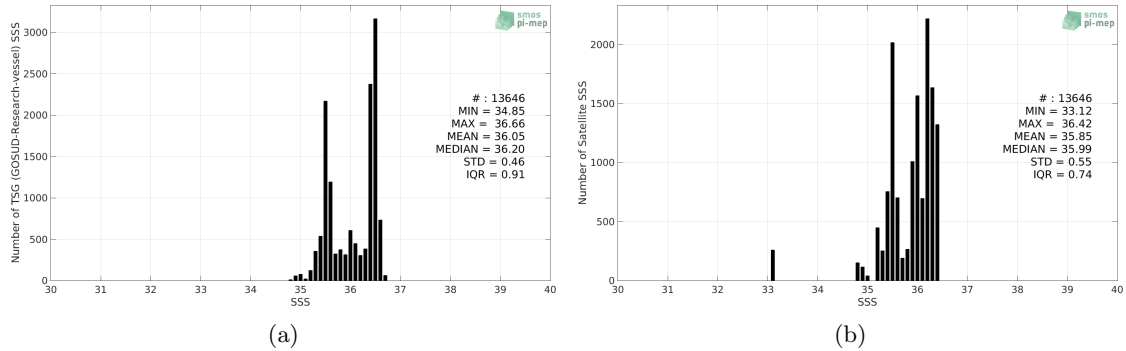
Figure 2: Histograms of SSS from TSG (GOSUD-Research-vessel) (a) and Aquarius SSS L3 OR v5 - Monthly (NASA-GSFC) (b) considering all match-up pairs per bins of 0.1 over the OTT zone Pi-MEP region and for the full satellite product period.
