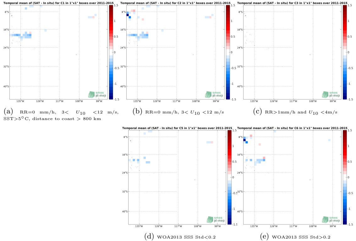
Figure 12: Temporal mean gridded over spatial boxes of size 1^\circ \times 1^\circ of \Delta SSS (Aquarius SSS L3 OR v5 - Monthly (NASA-GSFC) - TSG (GOSUD-Research-vessel)) for 5 different subdatasets corresponding to:RR=0 mm/h, 3 < U_{10} < 12 m/s, SST >5^\circ\text{C} , distance to coast > 800 km (a), RR=0 mm/h, 3 < U_{10} < 12 m/s (b), RR >1 mm/h and U_{10} < 4 m/s (c), WOA2013 SSS Std <0.2 (d), WOA2013 SSS Std >0.2 (e).
