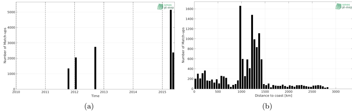
Figure 1: Number of match-ups between TSG (GOSUD-Research-vessel) and Aquarius SSS L3 OR v5 - Monthly (NASA-GSFC) SSS as a function of time (a) and as function of the distance to coast (b) over the OTT zone Pi-MEP region and for the full satellite product period.
