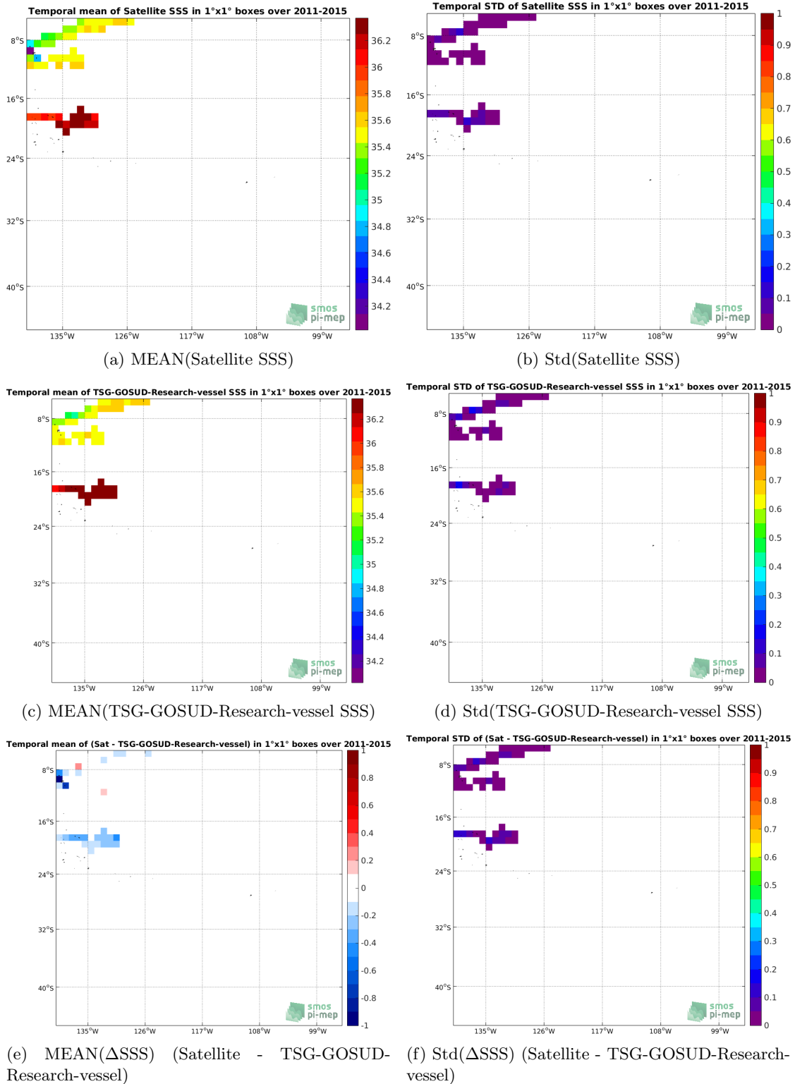
Figure 6: Temporal mean (left) and Std (right) of SSS from Aquarius-L3-OR-V5-MONTHLY-1DEG (top), TSG-GOSUD-Research-vessel (middle), and of \Delta SSS (Satellite - TSG-GOSUD-Research-vessel). Only match-up pairs are used to generate these maps.
