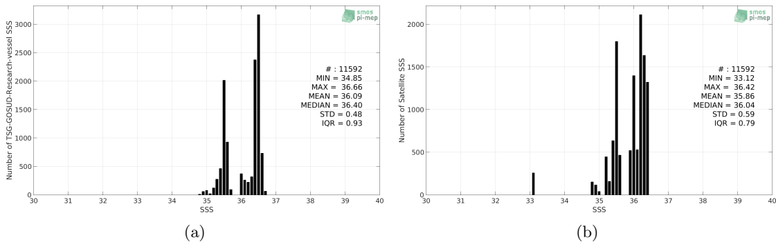
Figure 2: Histograms of SSS from TSG-GOSUD-Research-vessel (a) and Aquarius-L3-OR-V5-MONTHLY-1DEG (b) considering all match-up pairs per bins of 0.1 over the OTT zone Pi-MEP region and for the full satellite product period.
