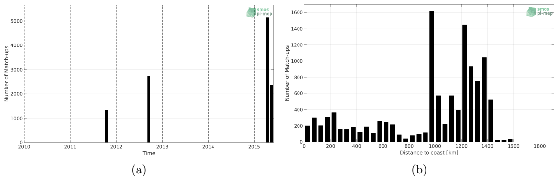
Figure 1: Number of match-ups between TSG-GOSUD-Research-vessel and Aquarius-L3-OR-V5-MONTHLY-1DEG SSS as a function of time (a) and as function of the distance to coast (b) over the OTT zone Pi-MEP region and for the full satellite product period.
