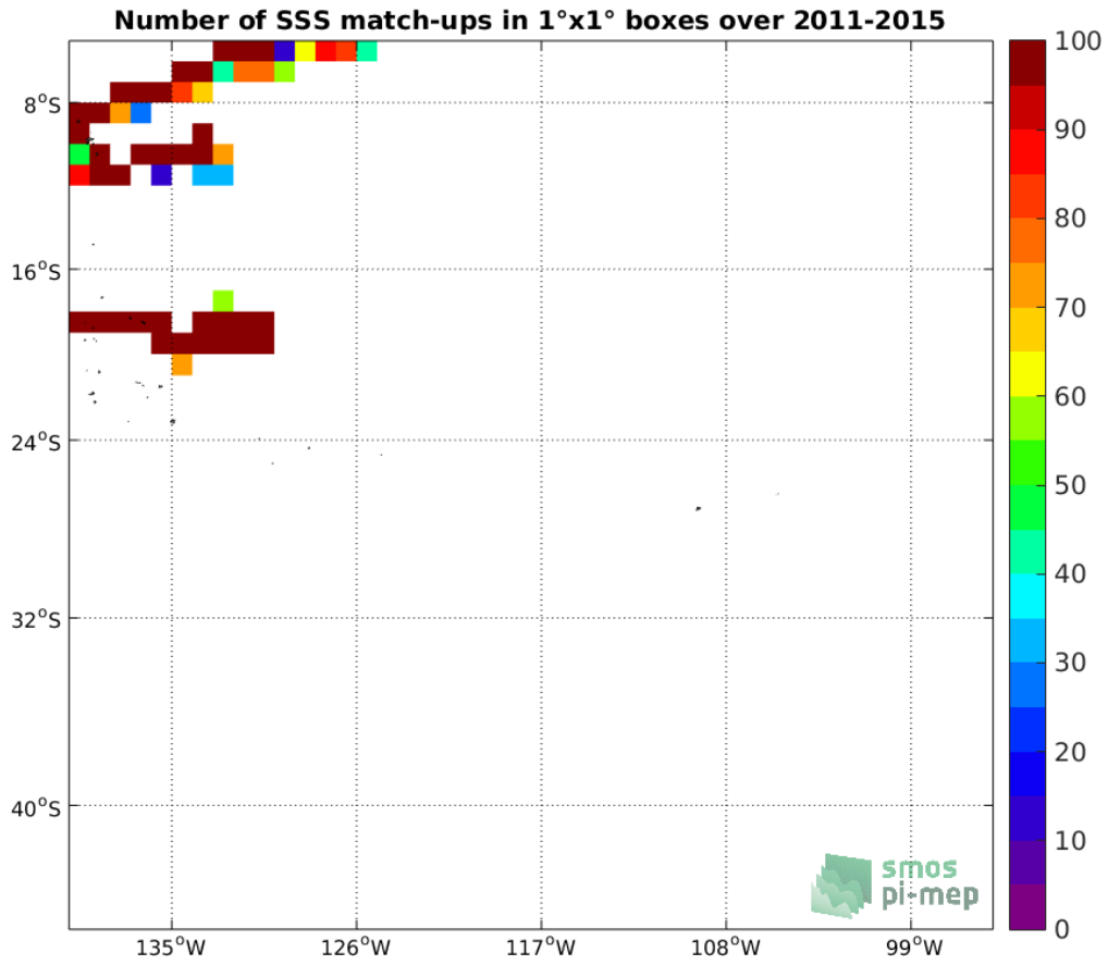
Figure 4: Number of SSS match-ups between TSG-GOSUD-Research-vessel SSS and the Aquarius-L3-OR-V5-MONTHLY-1DEG SSS product for the OTT zone Pi-MEP region over 1°x1° boxes and for the full satellite product period.
