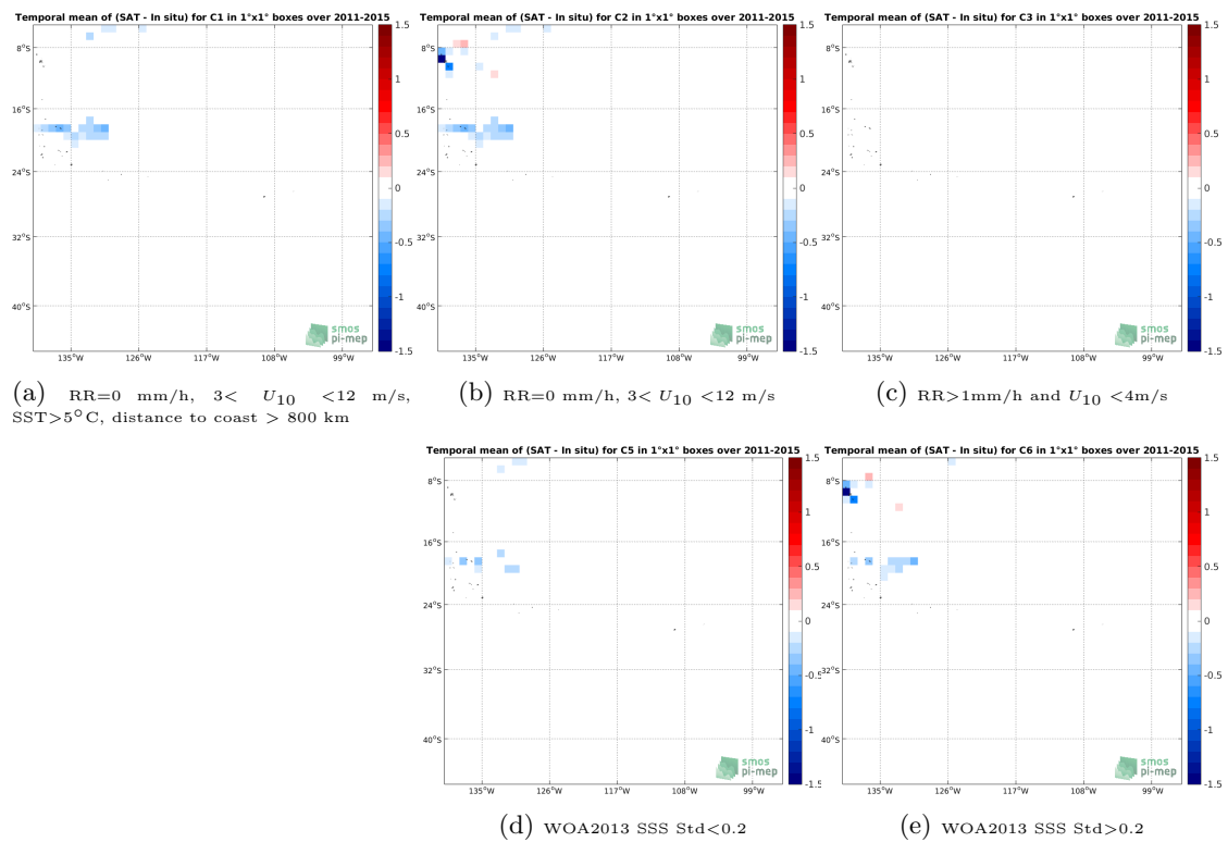
Figure 12: Temporal mean gridded over spatial boxes of size 1^\circ \times 1^\circ of \Delta SSS (Aquarius-L3-OR-V5-MONTHLY-1DEG - TSG-GOSUD-Research-vessel) for 5 different subdatasets corresponding to:RR=0 mm/h, 3 < U_{10} < 12 m/s, SST >5^\circ\text{C} , distance to coast > 800 km (a), RR=0 mm/h, 3 < U_{10} < 12 m/s (b), RR >1 mm/h and U_{10} < 4 m/s (c), WOA2013 SSS Std <0.2 (d), WOA2013 SSS Std >0.2 (e).
