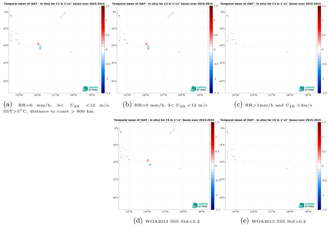
Figure 13: Temporal mean gridded over spatial boxes of size 1^\circ \times 1^\circ of \Delta SSS (Aquarius SSS L3 OR v5 - Monthly (NASA-GSFC) - Surface drifters) for 5 different subdatasets corresponding to: RR=0 mm/h, 3 < U_{10} < 12 m/s, SST > 5^\circ C , distance to coast > 800 km (a), RR=0 mm/h, 3 < U_{10} < 12 m/s (b), RR > 1 mm/h and U_{10} < 4 m/s (c), WOA2013 SSS Std < 0.2 (d), WOA2013 SSS Std > 0.2 (e).
