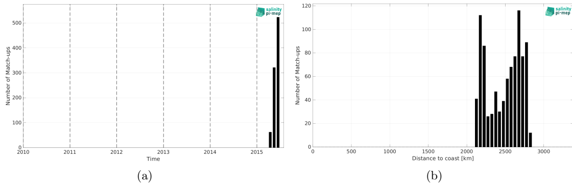
Figure 2: Number of match-ups between Surface drifters and Aquarius SSS L3 OR v5 - Monthly (NASA-GSFC) SSS as a function of time (a) and as function of the distance to coast (b) over the OTT zone Pi-MEP region and for the full satellite product period.
