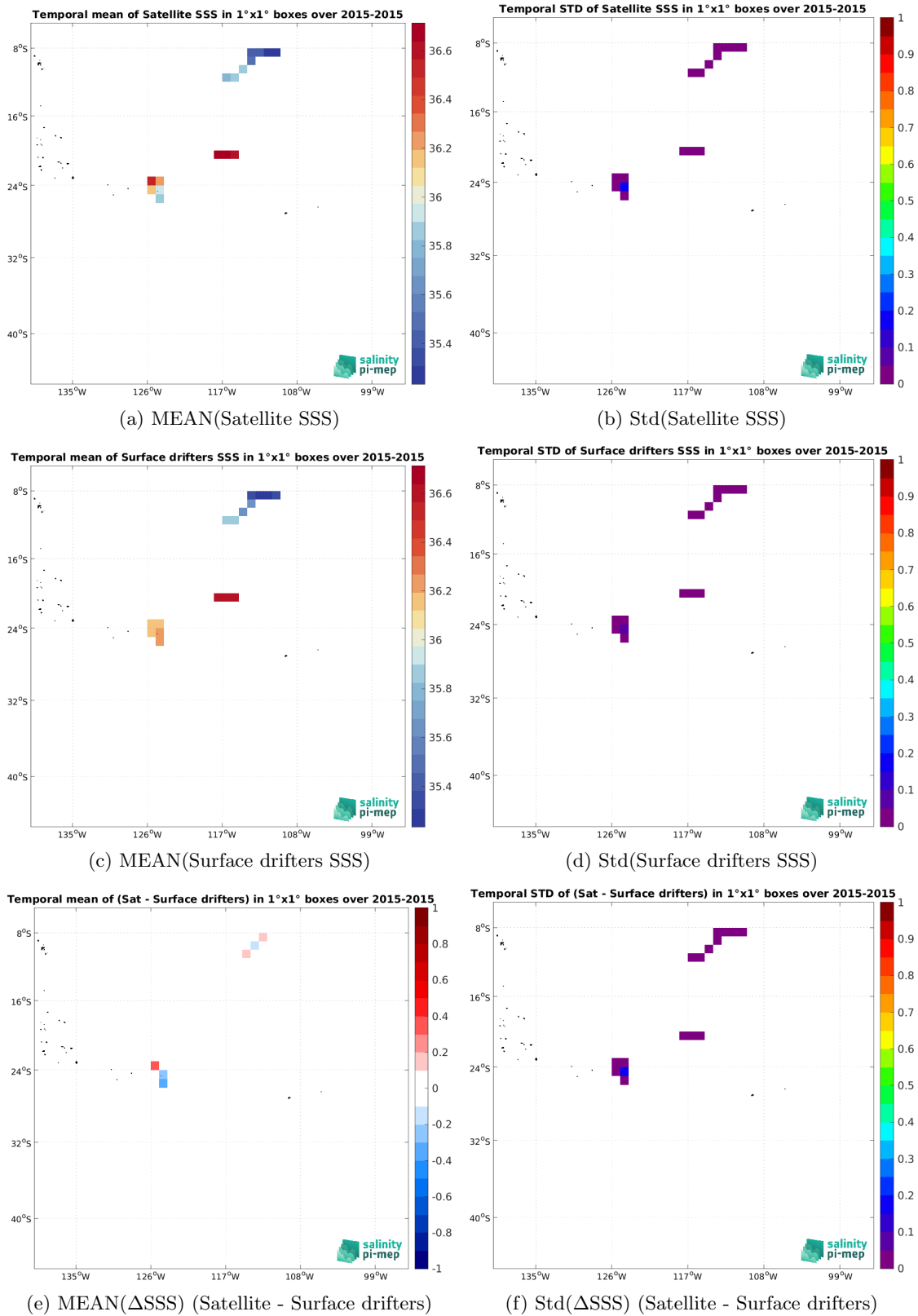
Figure 6: Temporal mean (left) and Std (right) of SSS from Aquarius SSS L3 OR v5 - Monthly (NASA-GSFC) (top), Surface drifters (middle), and of \Delta SSS (Satellite - Surface drifters). Only match-up pairs are used to generate these maps.
