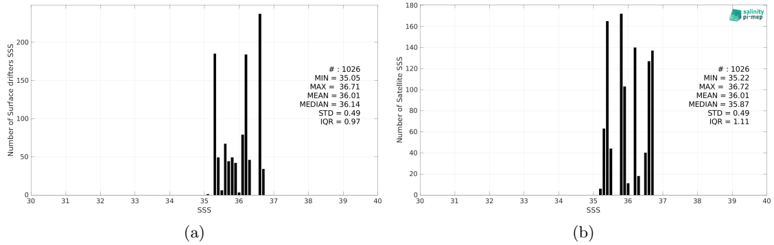
Figure 2: Histograms of SSS from Surface drifters (a) and Aquarius SSS L3 OR v5 - Monthly (NASA-GSFC) (b) considering all match-up pairs per bins of 0.1 over the OTT zone Pi-MEP region and for the full satellite product period.
