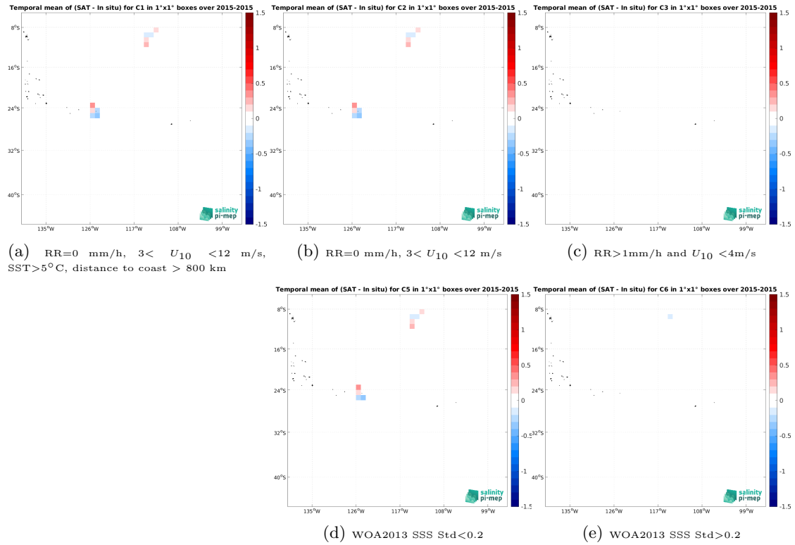
Figure 11: Temporal mean gridded over spatial boxes of size 1^\circ \times 1^\circ of \Delta\text{SSS} (Aquarius SSS L3 OR v5 - Monthly (NASA-GSFC) - Surface drifters) for 5 different subdatasets corresponding to:RR=0 mm/h, 3 < U_{10} < 12 m/s, SST >5^\circ\text{C} , distance to coast > 800 km (a), RR=0 mm/h, 3 < U_{10} < 12 m/s (b), RR >1 mm/h and U_{10} < 4 m/s (c), WOA2013 SSS Std <0.2 (d), WOA2013 SSS Std >0.2 (e).
