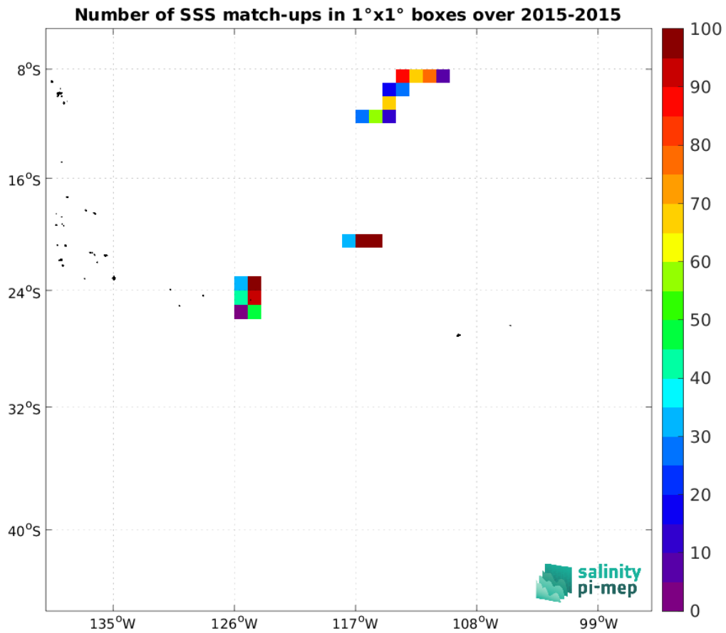
Figure 3: Number of SSS match-ups between Surface drifters SSS and the Aquarius SSS L3 OR v5 - Monthly (NASA-GSFC) SSS product for the OTT zone Pi-MEP region over 1°x1° boxes and for the full satellite product period.
