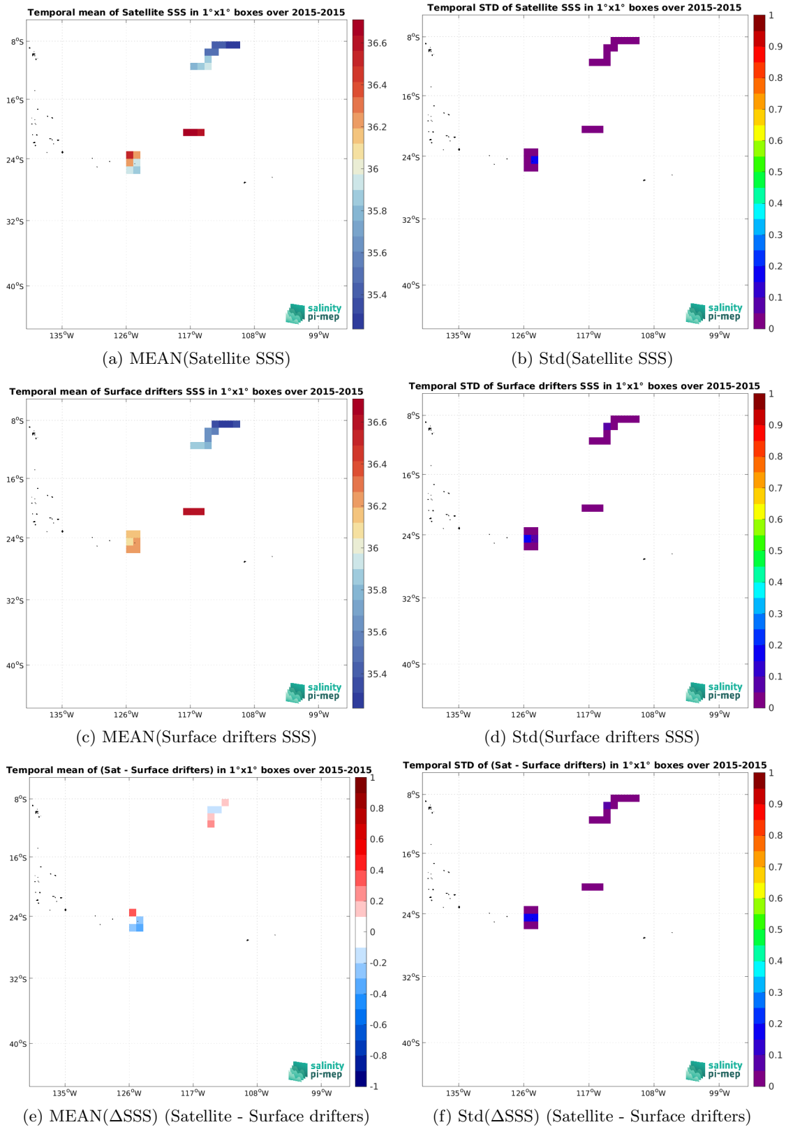
Figure 5: Temporal mean (left) and Std (right) of SSS from Aquarius SSS L3 OR v5 - Monthly (NASA-GSFC) (top), Surface drifters (middle), and of \Delta SSS (Satellite - Surface drifters). Only match-up pairs are used to generate these maps.
