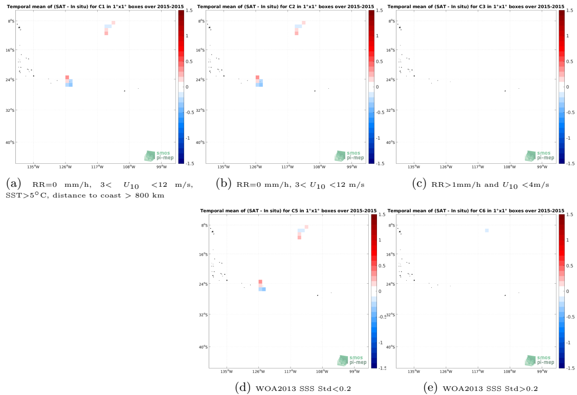
Figure 11: Temporal mean gridded over spatial boxes of size 1^\circ \times 1^\circ of \Delta SSS (Aquarius SSS L3 OR v5 - Monthly (NASA-GSFC) - Surface drifters) for 5 different subdatasets corresponding to: RR=0 mm/h, 3 < U_{10} < 12 m/s, SST > 5^\circ\text{C} , distance to coast > 800 km (a), RR=0 mm/h, 3 < U_{10} < 12 m/s (b), RR > 1 mm/h and U_{10} < 4 m/s (c), WOA2013 SSS Std < 0.2 (d), WOA2013 SSS Std > 0.2 (e).
