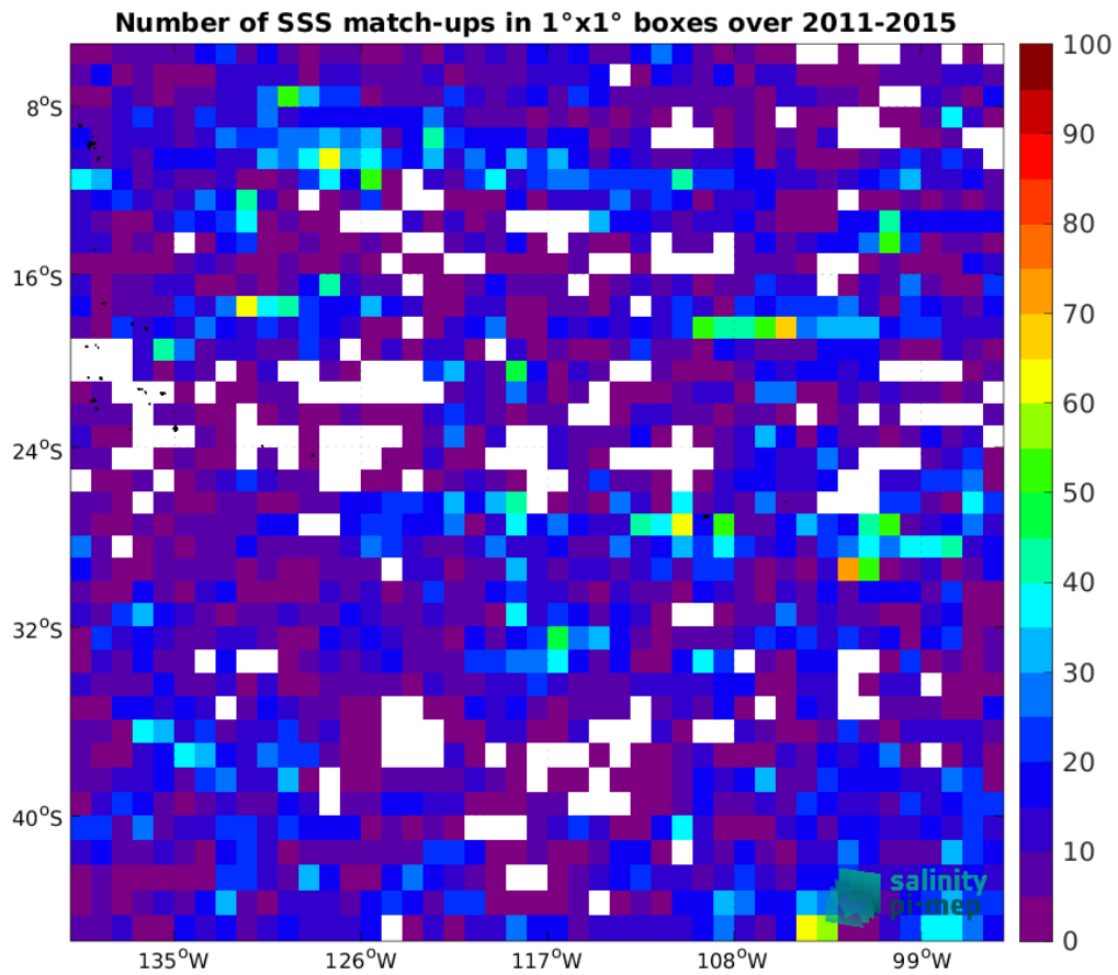
Figure 5: Number of SSS match-ups between Argo SSS and the Aquarius SSS L3 OR v5 - Monthly (NASA-GSFC) SSS product for the OTT zone Pi-MEP region over 1°x1° boxes and for the full satellite product period.
