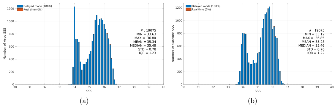
Figure 3: Histograms of SSS from Argo (a) and Aquarius SSS L3 OR v5 - Monthly (NASA-GSFC) (b) considering all match-up pairs per bins of 0.1 over the OTT zone Pi-MEP region and for the full satellite product period.
