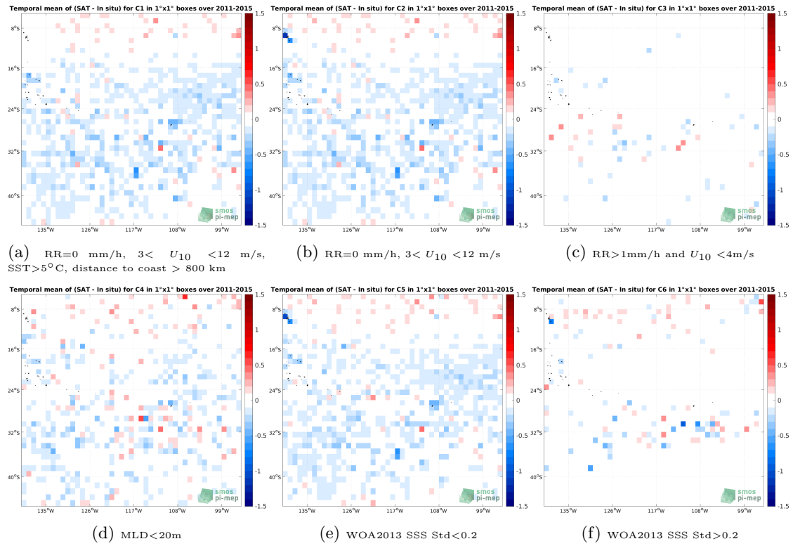
Figure 12: Temporal mean gridded over spatial boxes of size 1^\circ \times 1^\circ of \Delta SSS (Aquarius SSS L3 OR v5 - Monthly (NASA-GSFC) - Argo) for 6 different subdatasets corresponding to:RR=0 mm/h, 3 < U_{10} < 12 m/s, SST >5^\circ C, distance to coast > 800 km (a), RR=0 mm/h, 3 < U_{10} < 12 m/s (b), RR >1 mm/h and U_{10} < 4 m/s (c),MLD <20 m (d),WOA2013 SSS Std <0.2 (e),WOA2013 SSS Std >0.2 (f).
