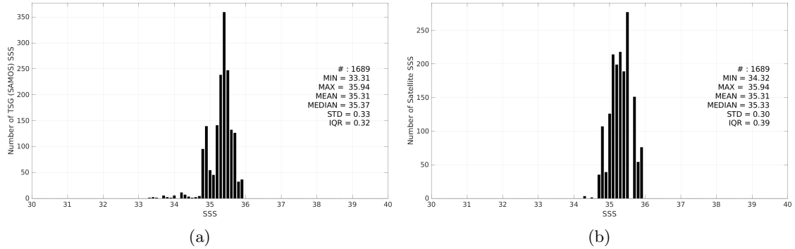
Figure 3: Histograms of SSS from TSG (SAMOS) (a) and Aquarius SSS L3 OR v5 - Monthly - Rain mask (NASA-GSFC) (b) considering all match-up pairs per bins of 0.1 over the OTT zone Pi-MEP region and for the full satellite product period.
