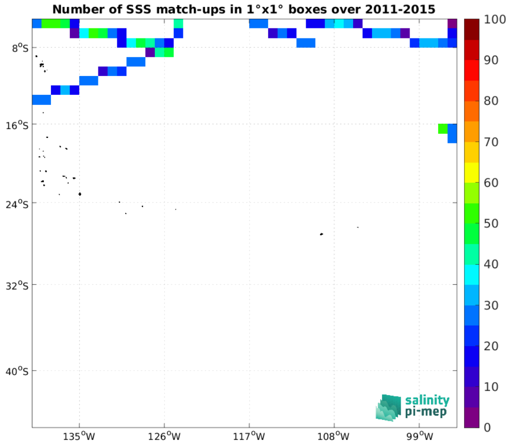
Figure 5: Number of SSS match-ups between TSG (SAMOS) SSS and the Aquarius SSS L3 OR v5 - Monthly - Rain mask (NASA-GSFC) SSS product for the OTT zone Pi-MEP region over 1^\circ \times 1^\circ boxes and for the full satellite product period.
