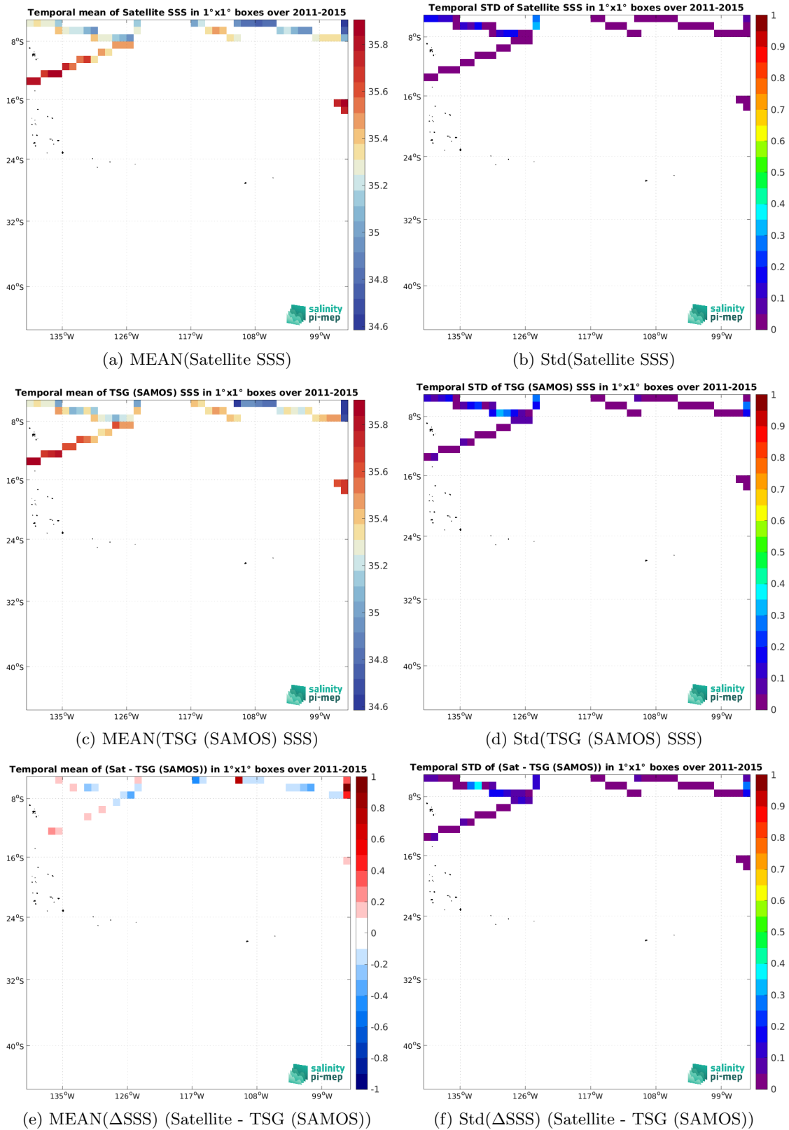
Figure 7: Temporal mean (left) and Std (right) of SSS from Aquarius SSS L3 OR v5 - Monthly - Rain mask (NASA-GSFC) (top), TSG (SAMOS) (middle), and of \Delta SSS (Satellite - TSG (SAMOS)). Only match-up pairs are used to generate these maps.
