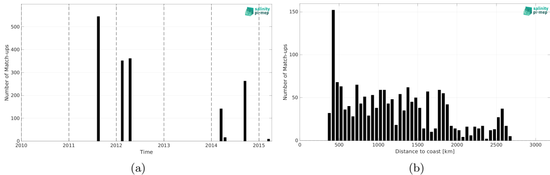
Figure 2: Number of match-ups between TSG (SAMOS) and Aquarius SSS L3 OR v5 - Monthly - Rain mask (NASA-GSFC) SSS as a function of time (a) and as function of the distance to coast (b) over the OTT zone Pi-MEP region and for the full satellite product period.
