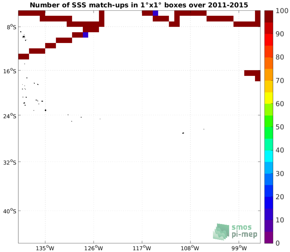
Figure 4: Number of SSS match-ups between TSG (SAMOS) SSS and the Aquarius SSS L3 OR v5 - Monthly - Rain mask (NASA-GSFC) SSS product for the OTT zone Pi-MEP region over 1^\circ \times 1^\circ boxes and for the full satellite product period.
