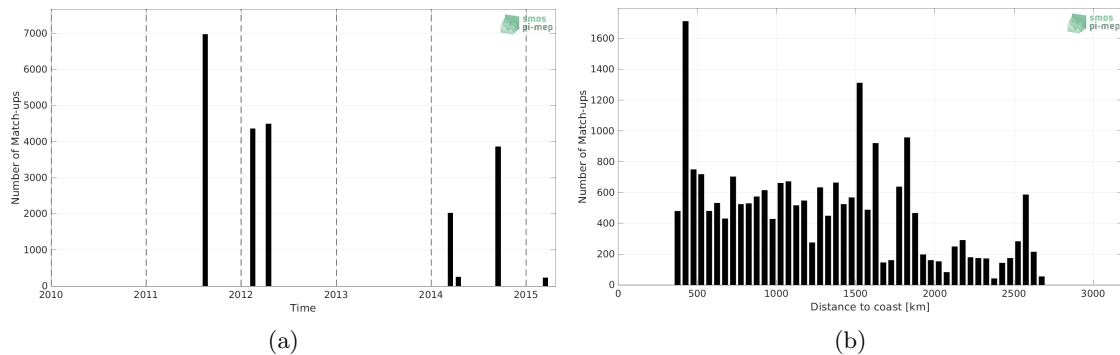
Figure 1: Number of match-ups between TSG (SAMOS) and Aquarius SSS L3 OR v5 - Monthly - Rain mask (NASA-GSFC) SSS as a function of time (a) and as function of the distance to coast (b) over the OTT zone Pi-MEP region and for the full satellite product period.
