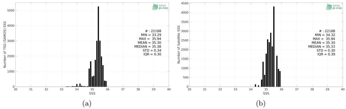
Figure 2: Histograms of SSS from TSG (SAMOS) (a) and Aquarius SSS L3 OR v5 - Monthly - Rain mask (NASA-GSFC) (b) considering all match-up pairs per bins of 0.1 over the OTT zone Pi-MEP region and for the full satellite product period.
