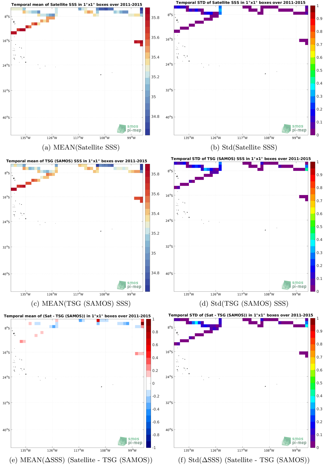
Figure 6: Temporal mean (left) and Std (right), of SSS from Aquarius SSS L3 OR v5 - Monthly - Rain mask (NASA-GSFC) (top), TSG (SAMOS) (middle), and of \Delta SSS (Satellite - TSG (SAMOS)). Only match-up pairs are used to generate these maps.
