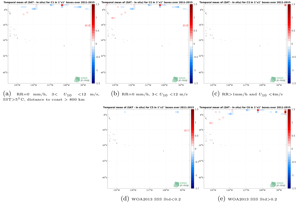
Figure 12: Temporal mean gridded over spatial boxes of size 1^{\circ}\times 1^{\circ} of \Delta\text{SSS} (Aquarius SSS L3 OR v5 - Monthly - Rain mask (NASA-GSFC) - TSG (SAMOS)) for 5 different subdatasets corresponding to:RR=0 mm/h, 3 < U_{10} < 12 m/s, SST >5^{\circ}\text{C} , distance to coast > 800 km (a), RR=0 mm/h, 3 < U_{10} < 12 m/s (b), RR >1\text{mm/h} and U_{10} < 4\text{m/s} (c), WOA2013 SSS Std <0.2 (d), WOA2013 SSS Std >0.2 (e).
