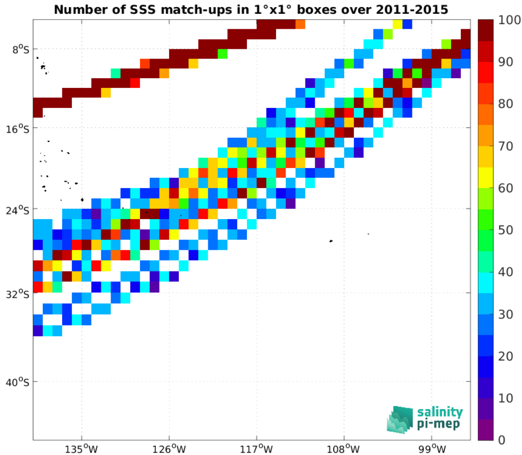
Figure 5: Number of SSS match-ups between TSG (LEGOS-DM) SSS and the Aquarius SSS L3 OR v5 - Monthly - Rain mask (NASA-GSFC) SSS product for the OTT zone Pi-MEP region over 1^\circ \times 1^\circ boxes and for the full satellite product period.
