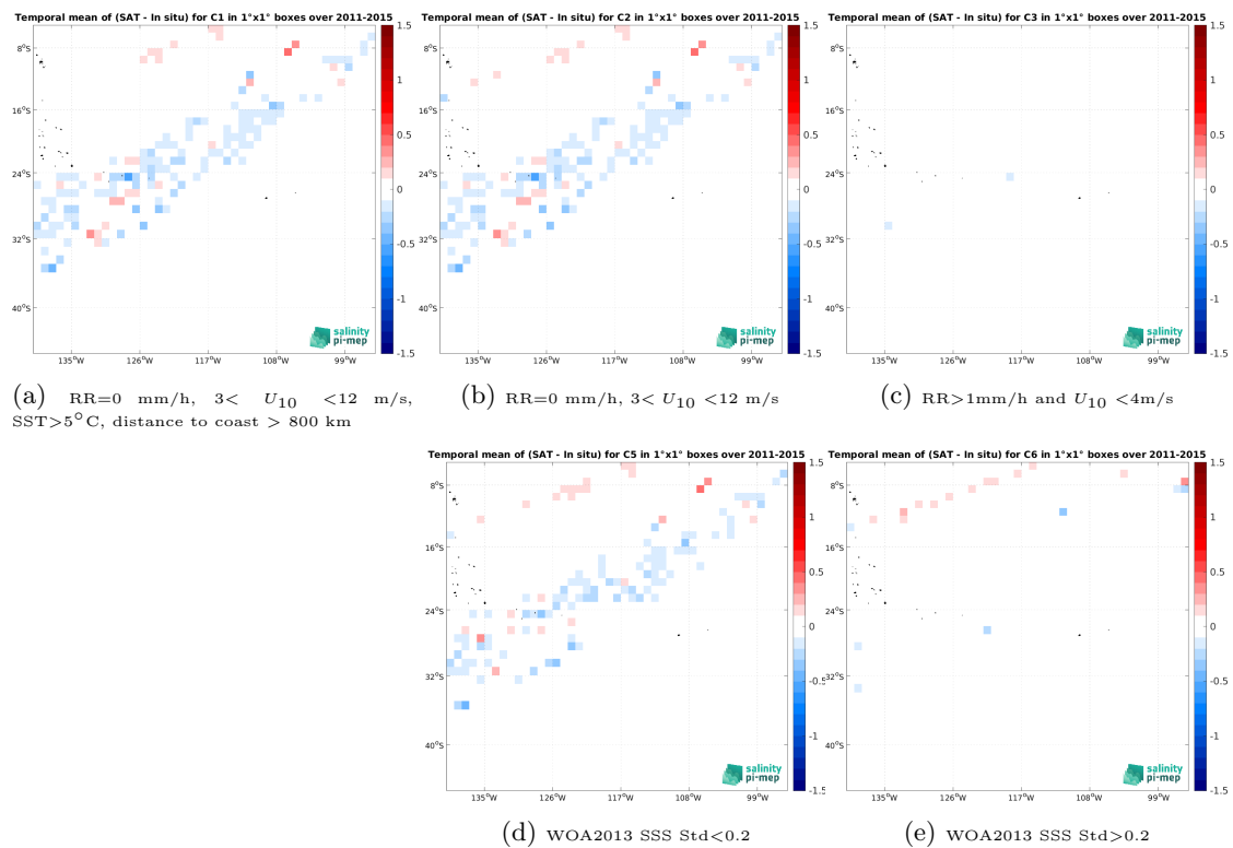
Figure 14: Temporal mean gridded over spatial boxes of size 1^\circ \times 1^\circ of \Delta SSS (Aquarius SSS L3 OR v5 - Monthly - Rain mask (NASA-GSFC) - TSG (LEGOS-DM)) for 5 different subdatasets corresponding to: RR=0 mm/h, 3 < U_{10} < 12 m/s, SST > 5^\circ\text{C} , distance to coast > 800 km (a), RR=0 mm/h, 3 < U_{10} < 12 m/s (b), RR > 1 mm/h and U_{10} < 4 m/s (c), WOA2013 SSS Std < 0.2 (d), WOA2013 SSS Std > 0.2 (e).
