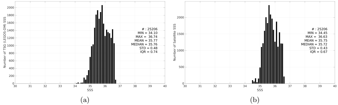
Figure 3: Histograms of SSS from TSG (LEGOS-DM) (a) and Aquarius SSS L3 OR v5 - Monthly - Rain mask (NASA-GSFC) (b) considering all match-up pairs per bins of 0.1 over the OTT zone Pi-MEP region and for the full satellite product period.
