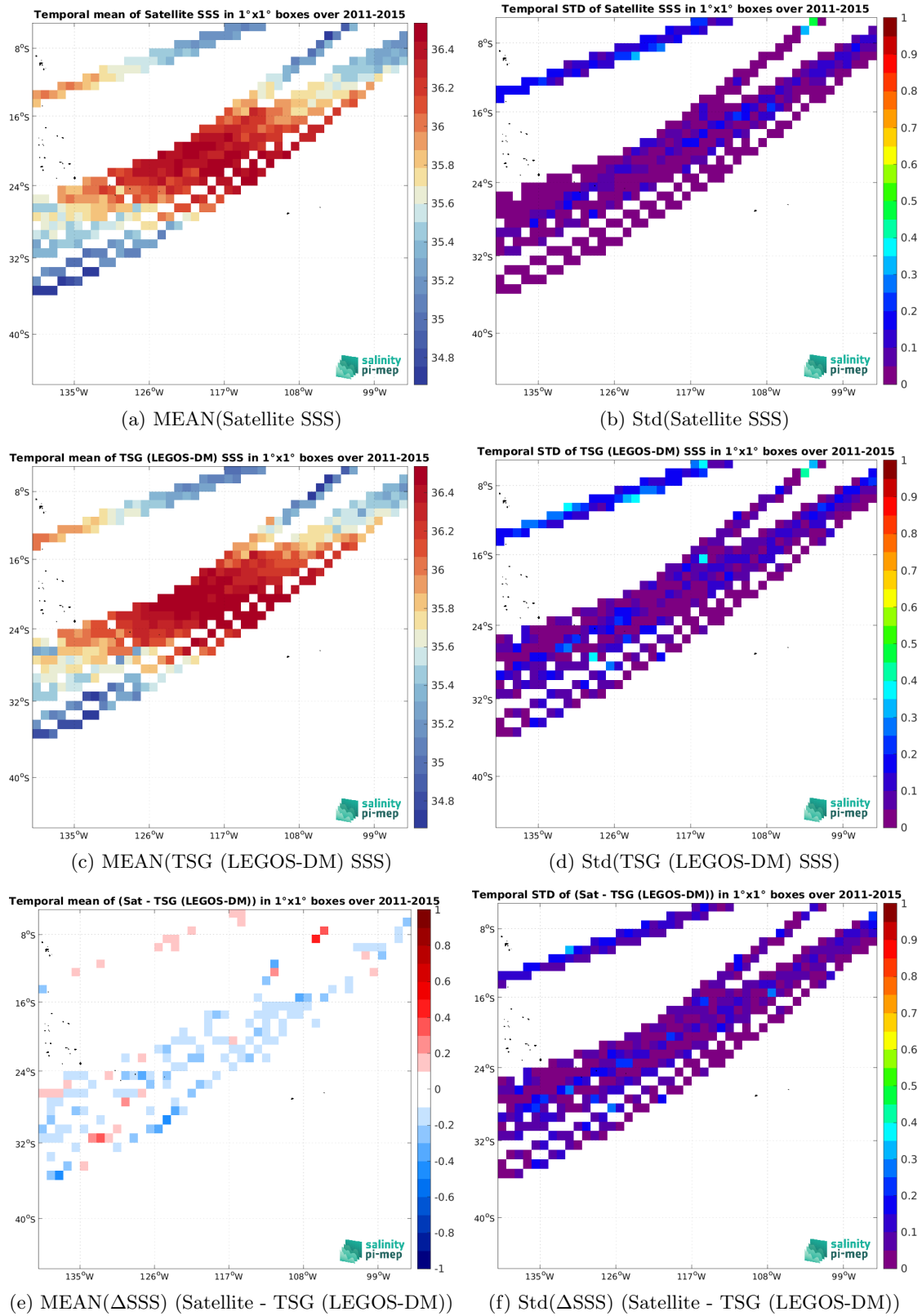
Figure 7: Temporal mean (left) and Std (right) of SSS from Aquarius SSS L3 OR v5 - Monthly - Rain mask (NASA-GSFC) (top), TSG (LEGOS-DM) (middle), and of \Delta SSS (Satellite - TSG (LEGOS-DM)). Only match-up pairs are used to generate these maps.
