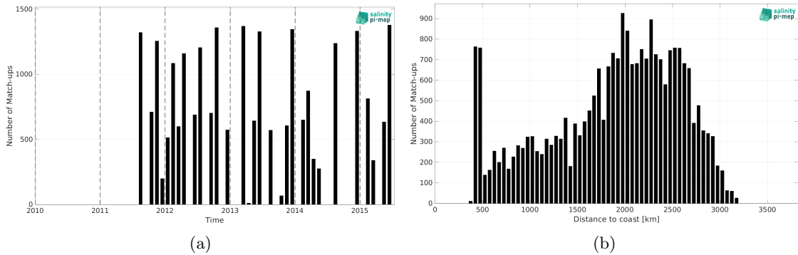
Figure 2: Number of match-ups between TSG (LEGOS-DM) and Aquarius SSS L3 OR v5 - Monthly - Rain mask (NASA-GSFC) SSS as a function of time (a) and as function of the distance to coast (b) over the OTT zone Pi-MEP region and for the full satellite product period.
