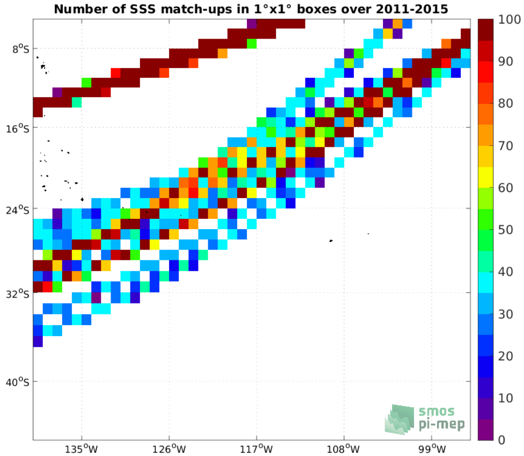
Figure 4: Number of SSS match-ups between TSG (LEGOS-DM) SSS and the Aquarius SSS L3 OR v5 - Monthly - Rain mask (NASA-GSFC) SSS product for the OTT zone Pi-MEP region over 1°x1° boxes and for the full satellite product period.
