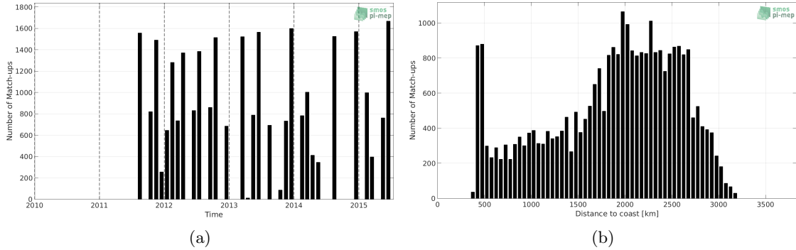
Figure 1: Number of match-ups between TSG-LEGOS-DM and Aquarius-L3-OR-V5-MONTHLY-RAIN-MASK-1DEG SSS as a function of time (a) and as function of the distance to coast (b) over the OTT zone Pi-MEP region and for the full satellite product period.
