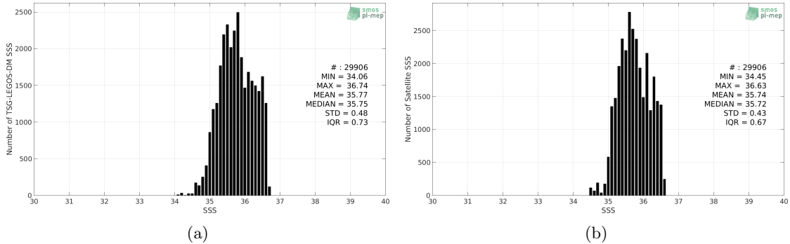
Figure 2: Histograms of SSS from TSG-LEGOS-DM (a) and Aquarius-L3-OR-V5-MONTHLY-RAIN-MASK-1DEG (b) considering all match-up pairs per bins of 0.1 over the OTT zone Pi-MEP region and for the full satellite product period.
