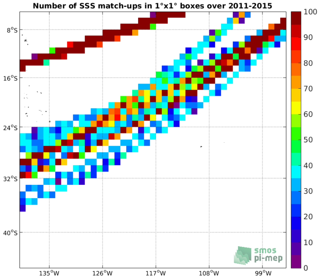
Figure 4: Number of SSS match-ups between TSG-LEGOS-DM SSS and the Aquarius-L3-OR-V5-MONTHLY-RAIN-MASK-1DEG SSS product for the OTT zone Pi-MEP region over 1°x1° boxes and for the full satellite product period.
