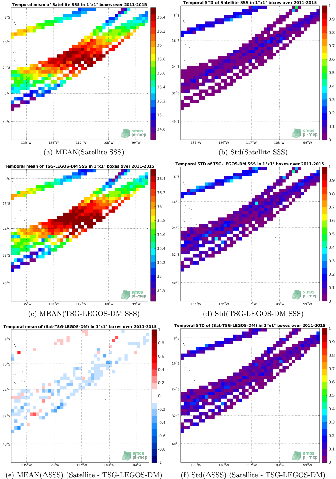
Figure 6: Temporal mean (left) and Std (right) of SSS from Aquarius-L3-OR-V5-MONTHLY-RAIN-MASK-1DEG (top), TSG-LEGOS-DM (middle), and of \Delta SSS (Satellite - TSG-LEGOS-DM). Only match-up pairs are used to generate these maps.
