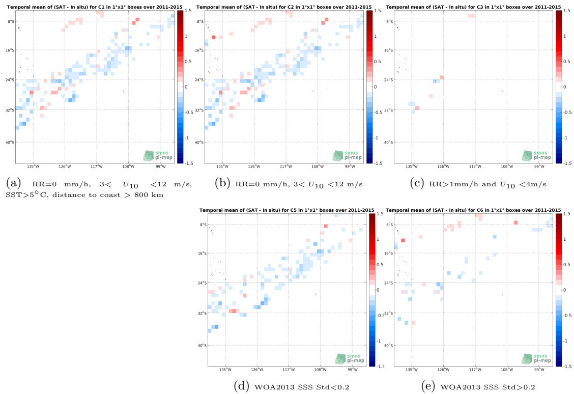
Figure 12: Temporal mean gridded over spatial boxes of size 1^\circ \times 1^\circ of \Delta SSS (Aquarius-L3-OR-V5-MONTHLY-RAIN-MASK-1DEG - TSG-LEGOS-DM) for 5 different subdatasets corresponding to:RR=0 mm/h, 3 < U_{10} < 12 m/s, SST >5^\circ C, distance to coast > 800 km (a), RR=0 mm/h, 3 < U_{10} < 12 m/s (b), RR >1 mm/h and U_{10} < 4 m/s (c), WOA2013 SSS Std <0.2 (d), WOA2013 SSS Std >0.2 (e).
