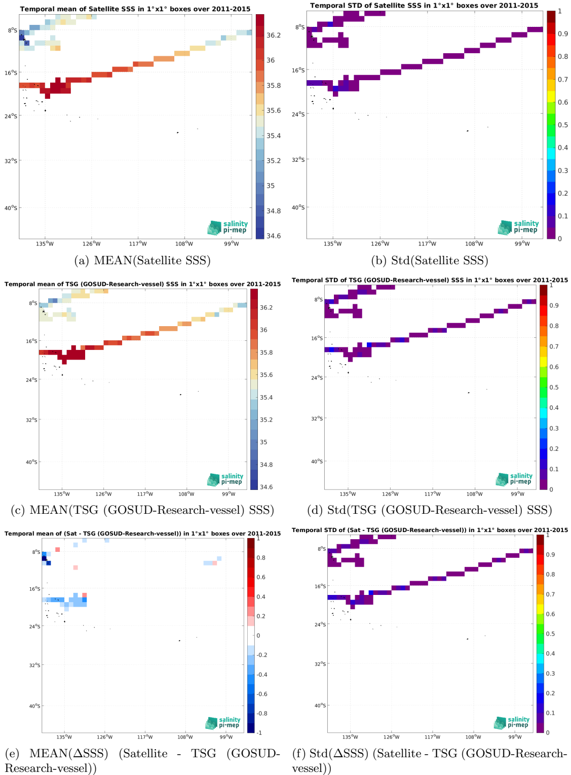
Figure 7: Temporal mean (left) and Std (right) of SSS from Aquarius SSS L3 OR v5 - Monthly - Rain mask (NASA-GSFC) (top), TSG (GOSUD-Research-vessel) (middle), and of \Delta SSS (Satellite - TSG (GOSUD-Research-vessel)). Only match-up pairs are used to generate these maps.
