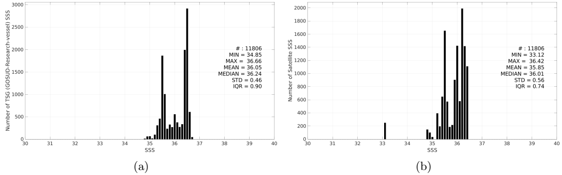
Figure 3: Histograms of SSS from TSG (GOSUD-Research-vessel) (a) and Aquarius SSS L3 OR v5 - Monthly - Rain mask (NASA-GSFC) (b) considering all match-up pairs per bins of 0.1 over the OTT zone Pi-MEP region and for the full satellite product period.
