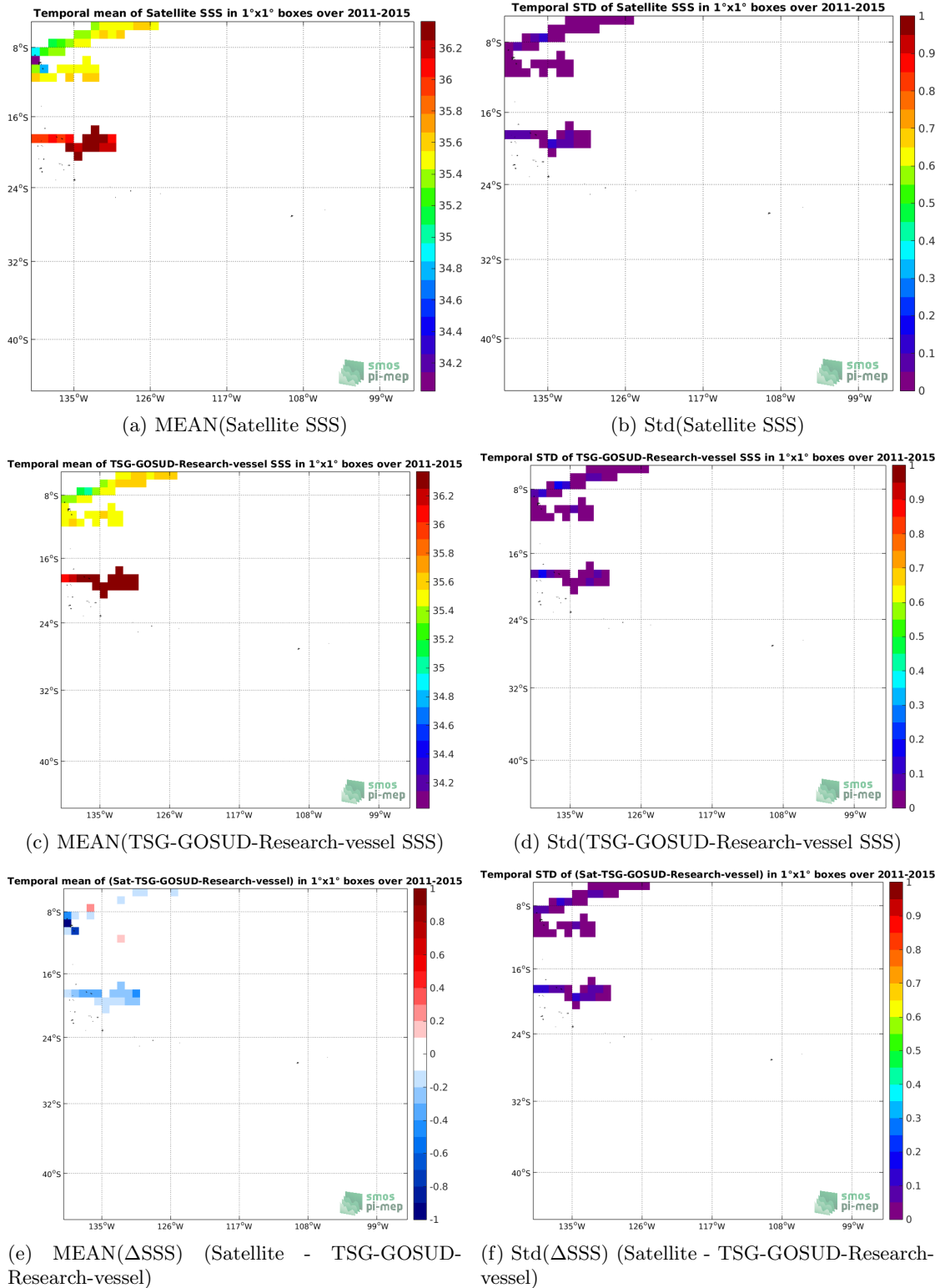
Figure 6: Temporal mean (left) and Std (right) of SSS from Aquarius-L3-OR-V5-MONTHLY-RAIN-MASK-1DEG (top), TSG-GOSUD-Research-vessel (middle), and of \Delta SSS (Satellite - TSG-GOSUD-Research-vessel). Only match-up pairs are used to generate these maps.
