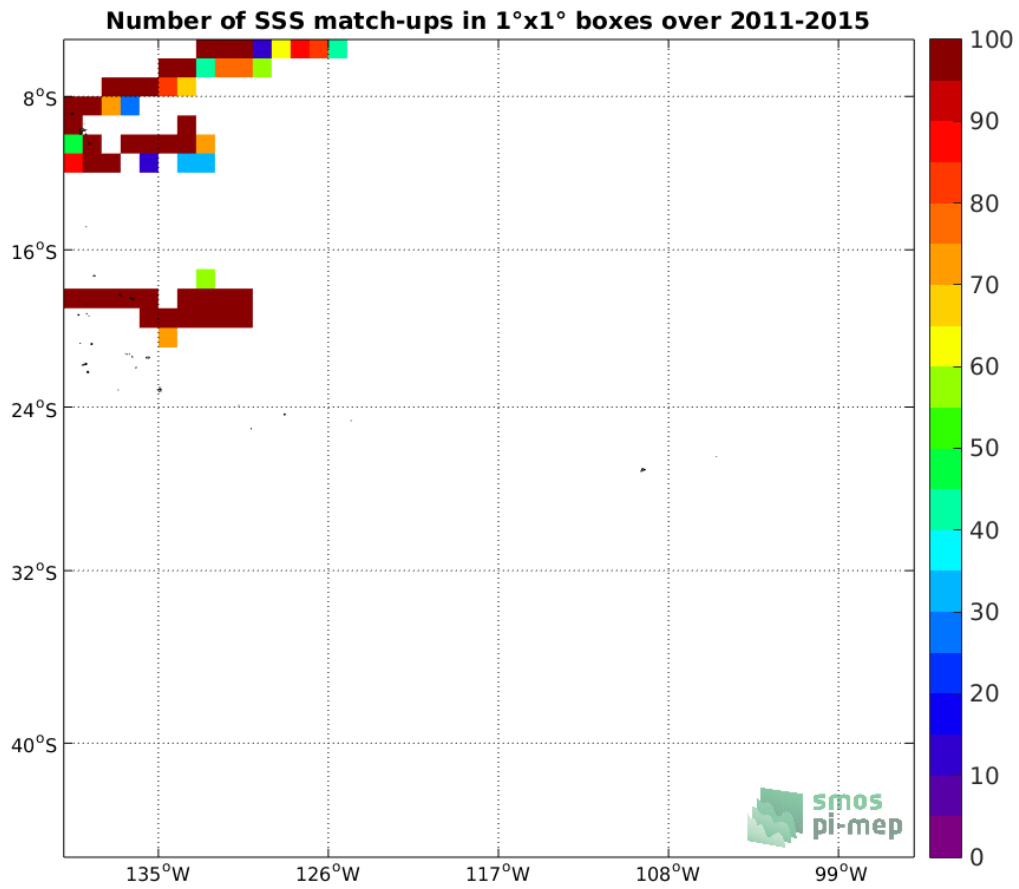
Figure 4: Number of SSS match-ups between TSG-GOSUD-Research-vessel SSS and the Aquarius-L3-OR-V5-MONTHLY-RAIN-MASK-1DEG SSS product for the OTT zone Pi-MEP region over 1°x1° boxes and for the full satellite product period.
