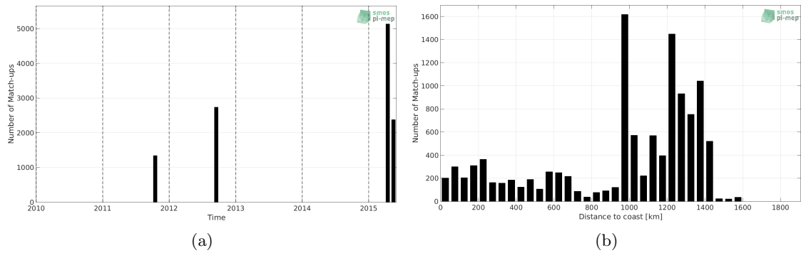
Figure 1: Number of match-ups between TSG-GOSUD-Research-vessel and Aquarius-L3-OR-V5-MONTHLY-RAIN-MASK-1DEG SSS as a function of time (a) and as function of the distance to coast (b) over the OTT zone Pi-MEP region and for the full satellite product period.
