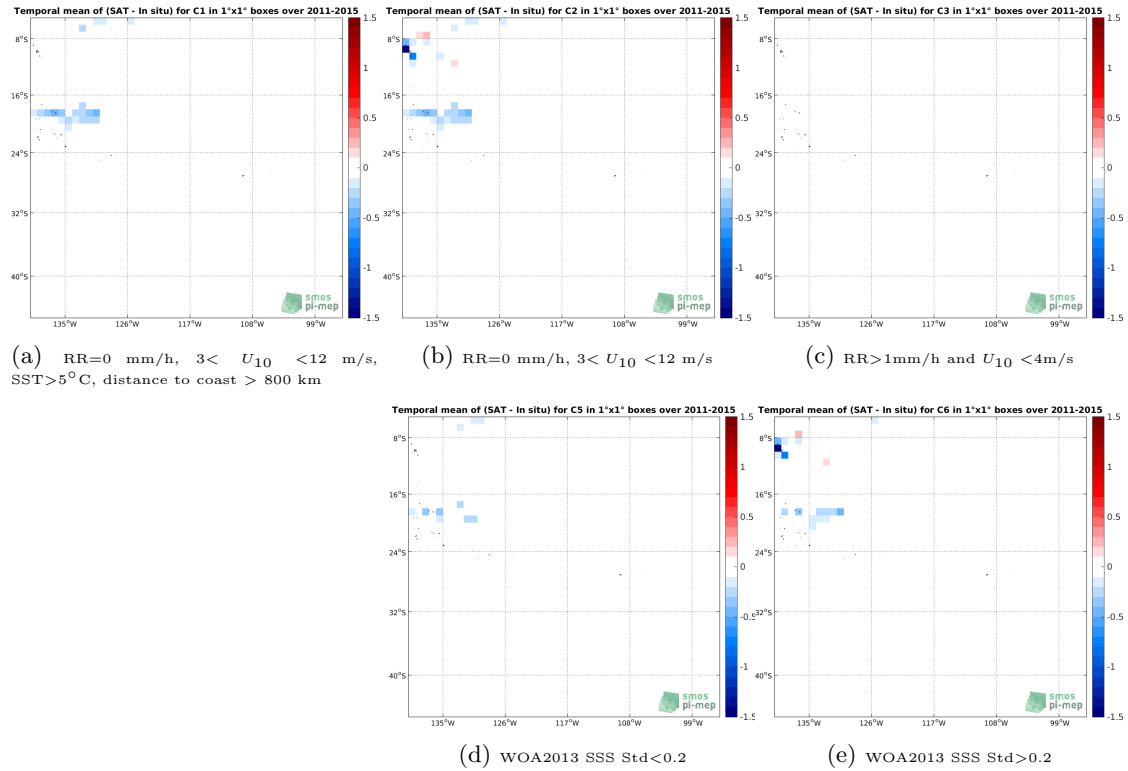
Figure 12: Temporal mean gridded over spatial boxes of size 1^\circ \times 1^\circ of \Delta SSS (Aquarius-L3-OR-V5-MONTHLY-RAIN-MASK-1DEG - TSG-GOSUD-Research-vessel) for 5 different subdatasets corresponding to:RR=0 mm/h, 3 < U_{10} < 12 m/s, SST >5^\circ C, distance to coast > 800 km (a), RR=0 mm/h, 3 < U_{10} < 12 m/s (b), RR >1 mm/h and U_{10} < 4 m/s (c), WOA2013 SSS Std <0.2 (d), WOA2013 SSS Std >0.2 (e).
