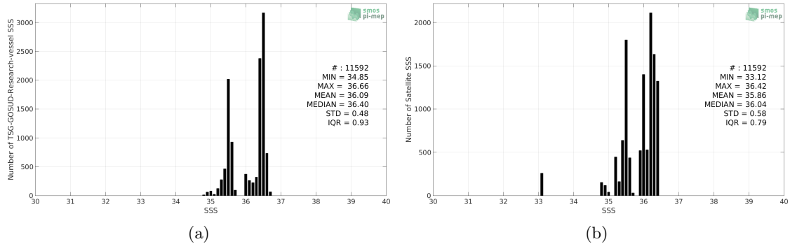
Figure 2: Histograms of SSS from TSG-GOSUD-Research-vessel (a) and Aquarius-L3-OR-V5-MONTHLY-RAIN-MASK-1DEG (b) considering all match-up pairs per bins of 0.1 over the OTT zone Pi-MEP region and for the full satellite product period.
