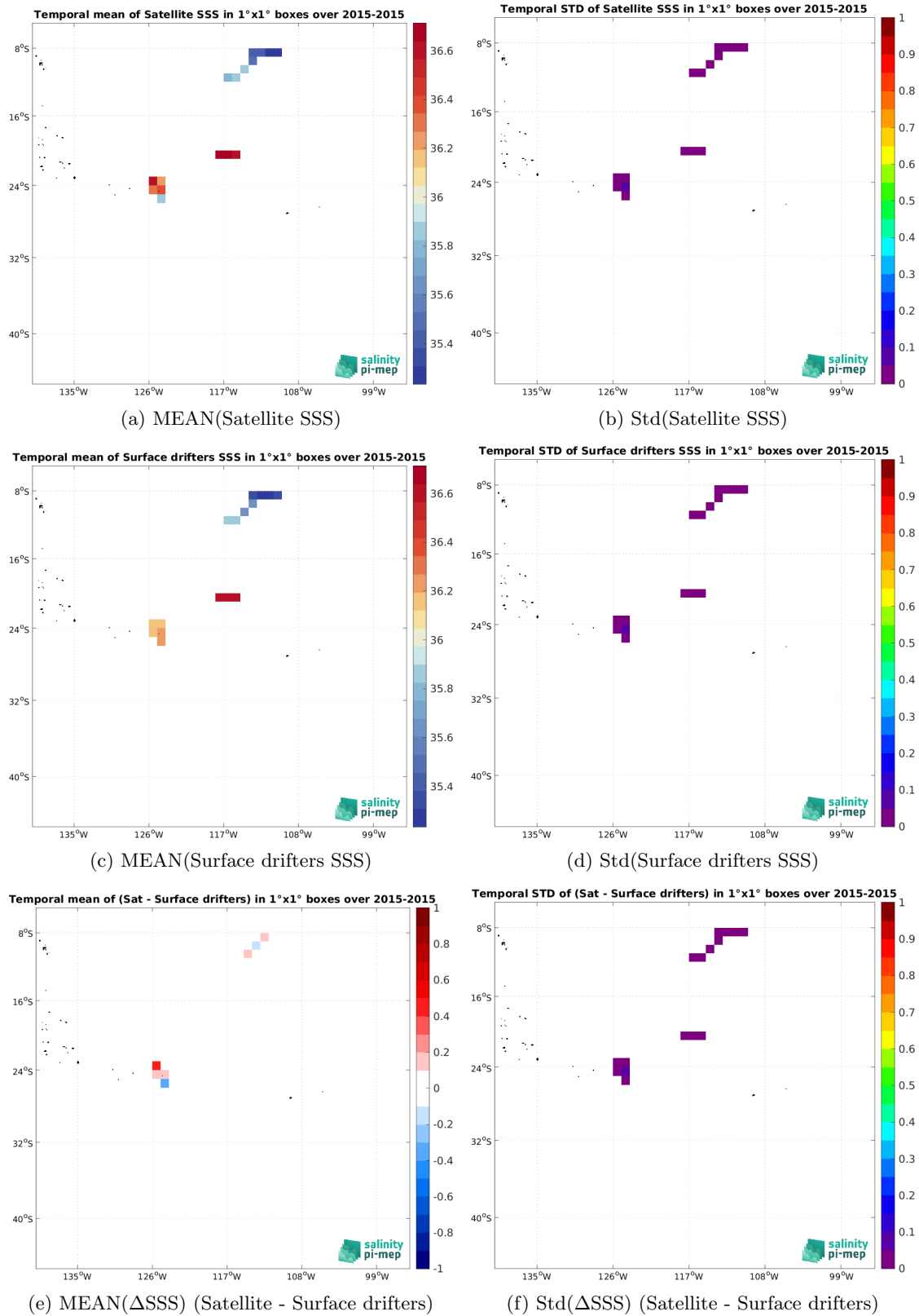
Figure 6: Temporal mean (left) and Std (right) of SSS from Aquarius SSS L3 OR v5 - Monthly - Rain mask (NASA-GSFC) (top), Surface drifters (middle), and of \Delta SSS (Satellite - Surface drifters). Only match-up pairs are used to generate these maps.
