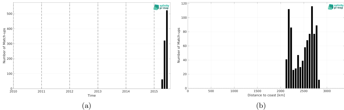
Figure 2: Number of match-ups between Surface drifters and Aquarius SSS L3 OR v5 - Monthly - Rain mask (NASA-GSFC) SSS as a function of time (a) and as function of the distance to coast (b) over the OTT zone Pi-MEP region and for the full satellite product period.
