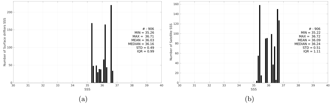
Figure 3: Histograms of SSS from Surface drifters (a) and Aquarius SSS L3 OR v5 - Monthly - Rain mask (NASA-GSFC) (b) considering all match-up pairs per bins of 0.1 over the OTT zone Pi-MEP region and for the full satellite product period.
