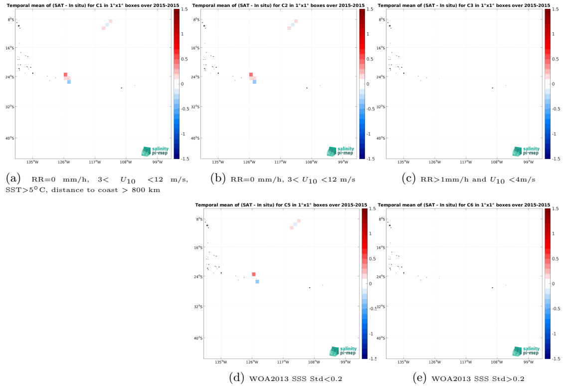
Figure 13: Temporal mean gridded over spatial boxes of size 1^\circ \times 1^\circ of \Delta\text{SSS} (Aquarius SSS L3 OR v5 - Monthly - Rain mask (NASA-GSFC) - Surface drifters) for 5 different subdatasets corresponding to:RR=0 mm/h, 3 < U_{10} < 12 m/s, SST >5^\circ\text{C} , distance to coast > 800 km (a), RR=0 mm/h, 3 < U_{10} < 12 m/s (b), RR >1 mm/h and U_{10} < 4 m/s (c), WOA2013 SSS Std <0.2 (d), WOA2013 SSS Std >0.2 (e).
