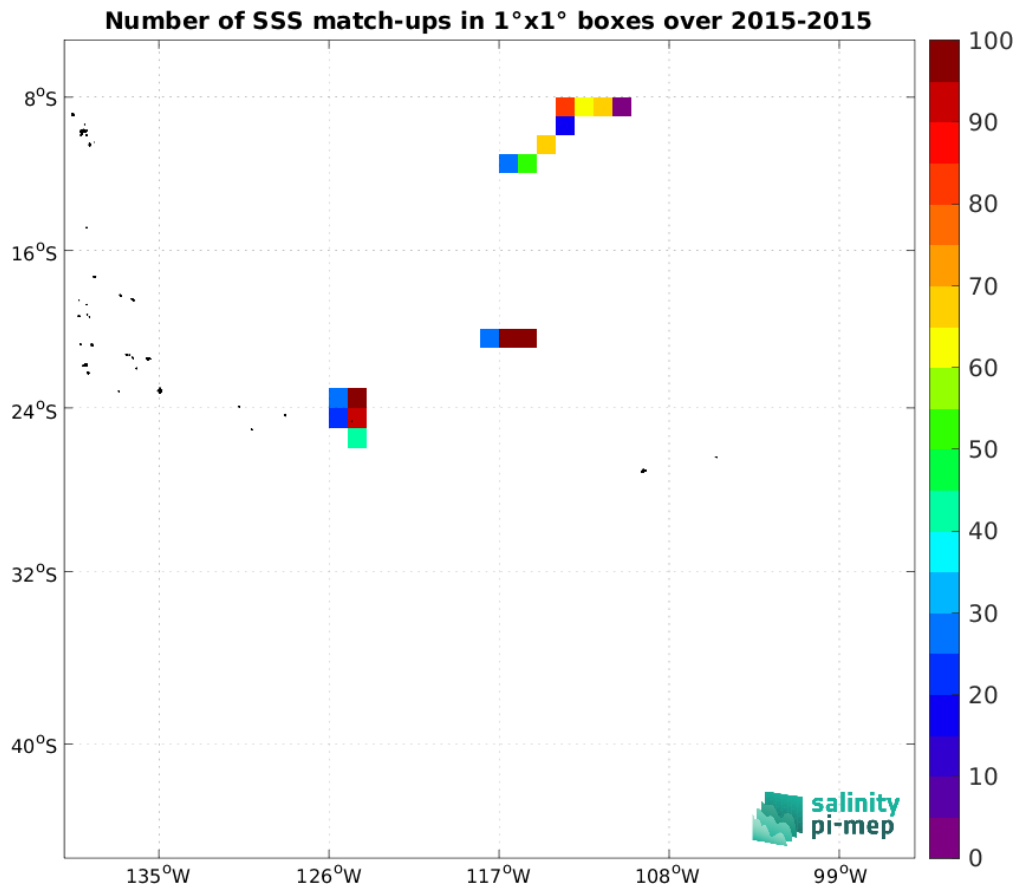
Figure 4: Number of SSS match-ups between Surface drifters SSS and the Aquarius SSS L3 OR v5 - Monthly - Rain mask (NASA-GSFC) SSS product for the OTT zone Pi-MEP region over 1°x1° boxes and for the full satellite product period.
