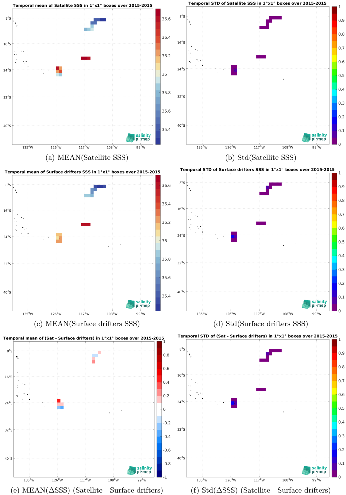
Figure 5: Temporal mean (left) and Std (right) of SSS from Aquarius SSS L3 OR v5 - Monthly - Rain mask (NASA-GSFC) (top), Surface drifters (middle), and of \Delta SSS (Satellite - Surface drifters). Only match-up pairs are used to generate these maps.
