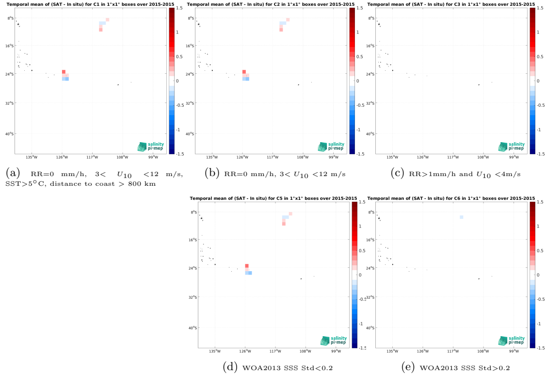
Figure 11: Temporal mean gridded over spatial boxes of size 1^{\circ}\times 1^{\circ} of \Delta\text{SSS} (Aquarius SSS L3 OR v5 - Monthly - Rain mask (NASA-GSFC) - Surface drifters) for 5 different subdatasets corresponding to:RR=0 mm/h, 3 < U_{10} < 12 m/s, SST >5^{\circ}\text{C} , distance to coast > 800 km (a), RR=0 mm/h, 3 < U_{10} < 12 m/s (b), RR >1 mm/h and U_{10} < 4 m/s (c), WOA2013 SSS Std <0.2 (d), WOA2013 SSS Std >0.2 (e).
