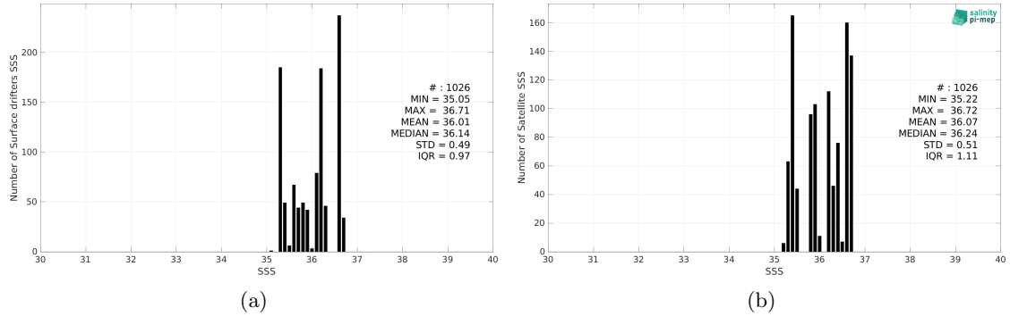
Figure 2: Histograms of SSS from Surface drifters (a) and Aquarius SSS L3 OR v5 - Monthly - Rain mask (NASA-GSFC) (b) considering all match-up pairs per bins of 0.1 over the OTT zone Pi-MEP region and for the full satellite product period.
