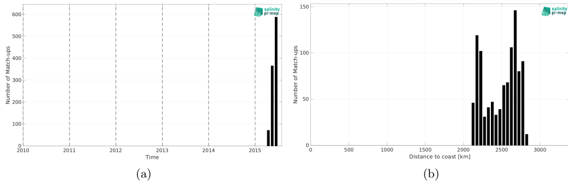
Figure 1: Number of match-ups between Surface drifters and Aquarius SSS L3 OR v5 - Monthly - Rain mask (NASA-GSFC) SSS as a function of time (a) and as function of the distance to coast (b) over the OTT zone Pi-MEP region and for the full satellite product period.
