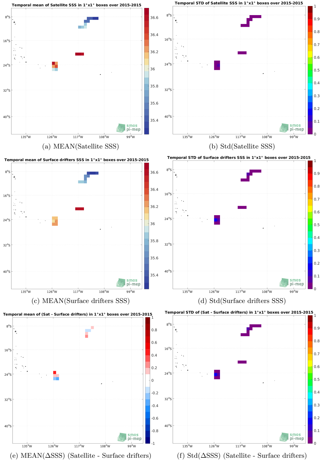
Figure 5: Temporal mean (left) and Std (right), of SSS from Aquarius SSS L3 OR v5 - Monthly - Rain mask (NASA-GSFC) (top), Surface drifters (middle), and of \Delta SSS (Satellite - Surface drifters). Only match-up pairs are used to generate these maps.
