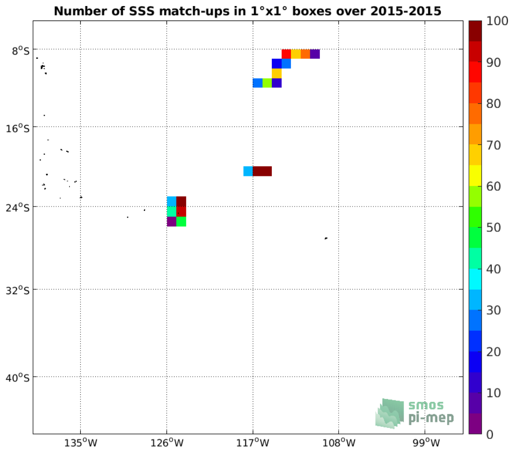
Figure 3: Number of SSS match-ups between Surface drifters SSS and the Aquarius SSS L3 OR v5 - Monthly - Rain mask (NASA-GSFC) SSS product for the OTT zone Pi-MEP region over 1^\circ \times 1^\circ boxes and for the full satellite product period.
