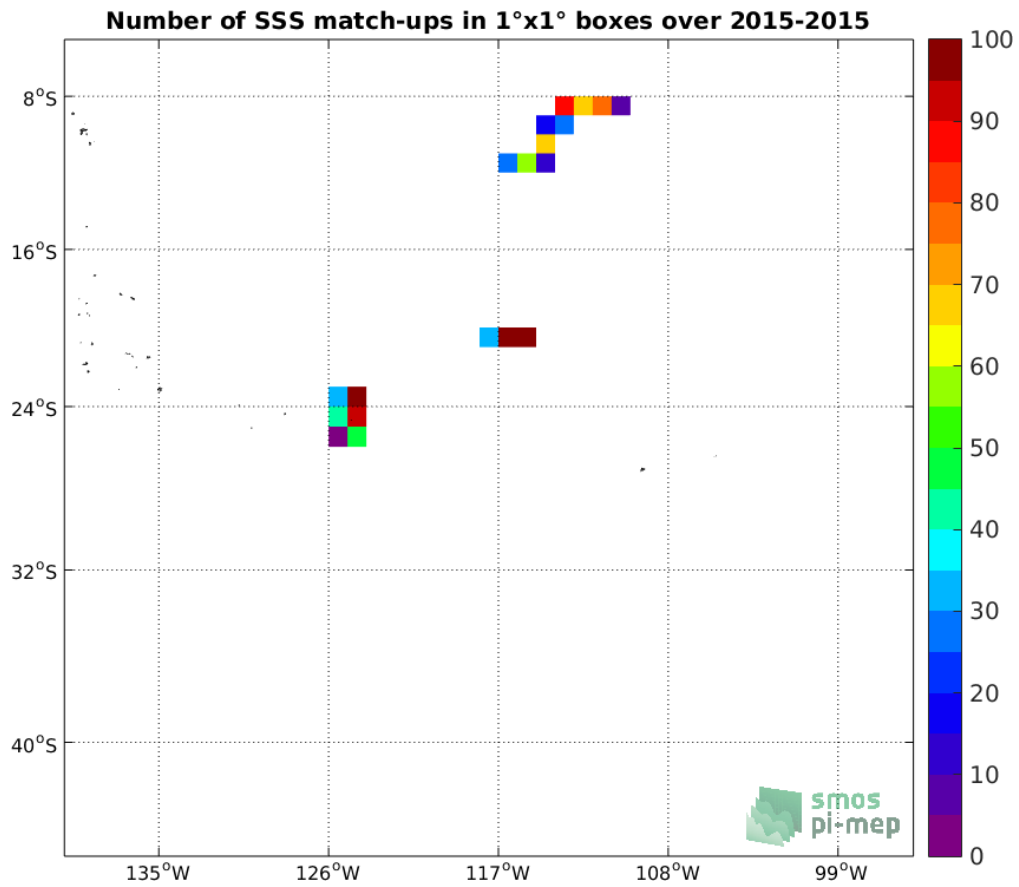
Figure 3: Number of SSS match-ups between Surface drifters SSS and the Aquarius-L3-OR-V5-MONTHLY-RAIN-MASK-1DEG SSS product for the OTT zone Pi-MEP region over 1°x1° boxes and for the full satellite product period.
