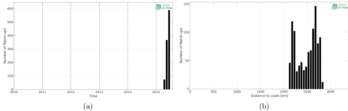
Figure 1: Number of match-ups between Surface drifters and Aquarius-L3-OR-V5-MONTHLY-RAIN-MASK-1DEG SSS as a function of time (a) and as function of the distance to coast (b) over the OTT zone Pi-MEP region and for the full satellite product period.
