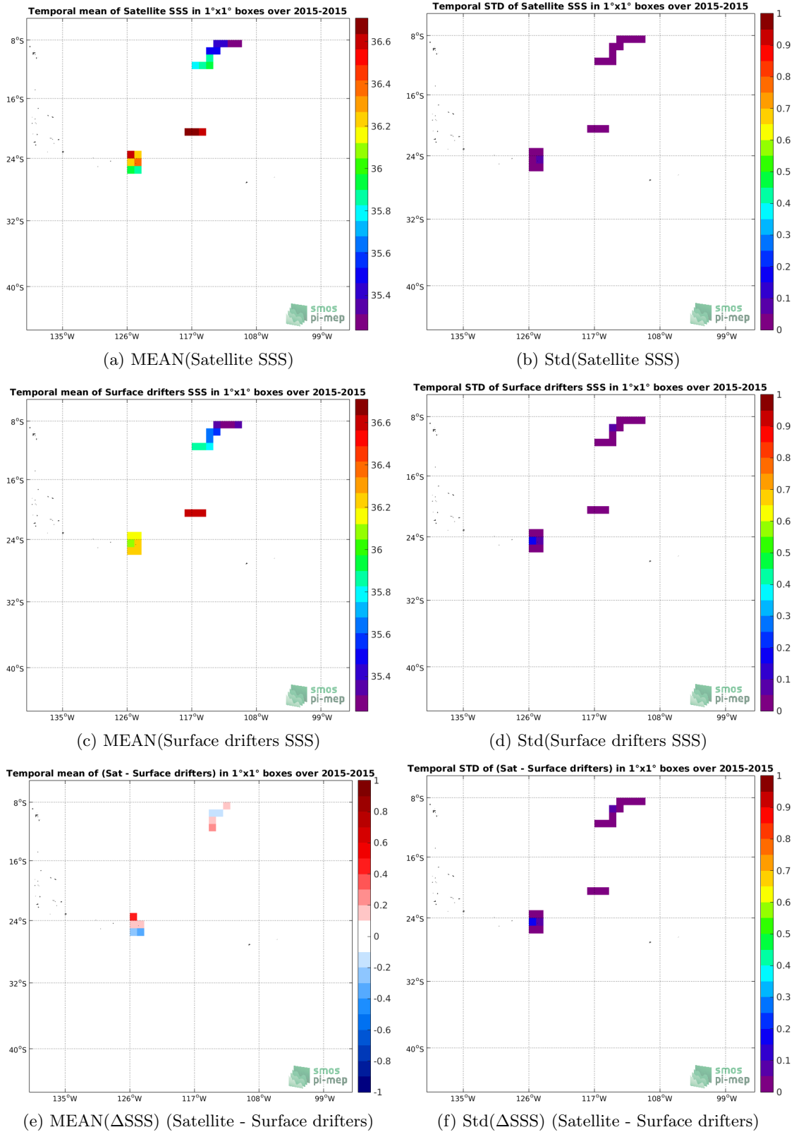
Figure 5: Temporal mean (left) and Std (right) of SSS from Aquarius-L3-OR-V5-MONTHLY-RAIN-MASK-1DEG (top), Surface drifters (middle), and of \Delta SSS (Satellite - Surface drifters). Only match-up pairs are used to generate these maps.
