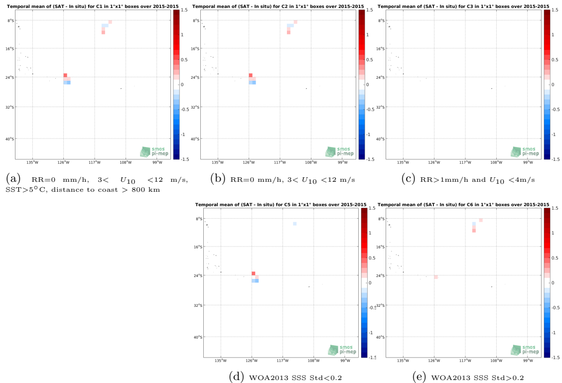
Figure 11: Temporal mean gridded over spatial boxes of size 1^\circ \times 1^\circ of \Delta SSS (Aquarius-L3-OR-V5-MONTHLY-RAIN-MASK-1DEG - Surface drifters) for 5 different subdatasets corresponding to: RR=0 mm/h, 3 < U_{10} < 12 m/s, SST > 5^\circ\text{C} , distance to coast > 800 km (a), RR=0 mm/h, 3 < U_{10} < 12 m/s (b), RR > 1 mm/h and U_{10} < 4 m/s (c), WOA2013 SSS Std < 0.2 (d), WOA2013 SSS Std > 0.2 (e).
