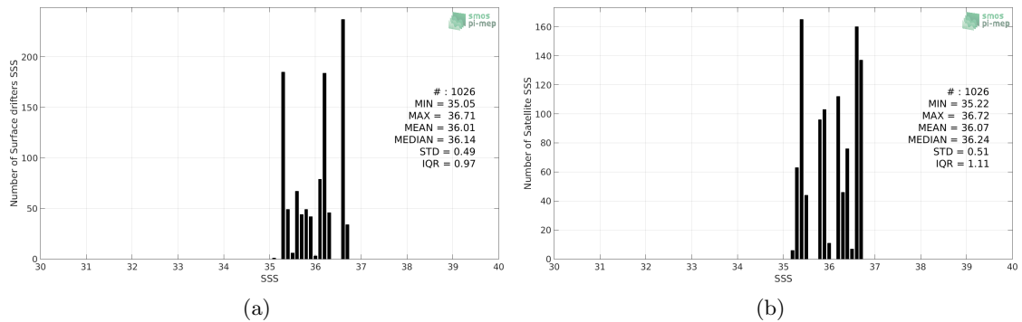
Figure 2: Histograms of SSS from Surface drifters (a) and Aquarius-L3-OR-V5-MONTHLY-RAIN-MASK-1DEG (b) considering all match-up pairs per bins of 0.1 over the OTT zone Pi-MEP region and for the full satellite product period.
