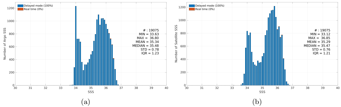
Figure 3: Histograms of SSS from Argo (a) and Aquarius SSS L3 OR v5 - Monthly - Rain mask (NASA-GSFC) (b) considering all match-up pairs per bins of 0.1 over the OTT zone Pi-MEP region and for the full satellite product period.
