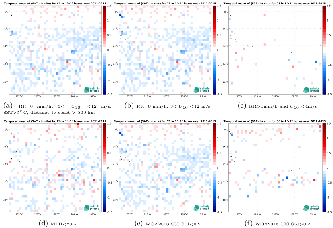
Figure 14: Temporal mean gridded over spatial boxes of size 1^\circ \times 1^\circ of \Delta SSS (Aquarius SSS L3 OR v5 - Monthly - Rain mask (NASA-GSFC) - Argo) for 6 different subdatasets corresponding to:RR=0 mm/h, 3 < U_{10} < 12 m/s, SST >5^\circ C, distance to coast > 800 km (a), RR=0 mm/h, 3 < U_{10} < 12 m/s (b), RR >1 mm/h and U_{10} < 4 m/s (c),MLD <20 m (d),WOA2013 SSS Std <0.2 (e),WOA2013 SSS Std >0.2 (f).
