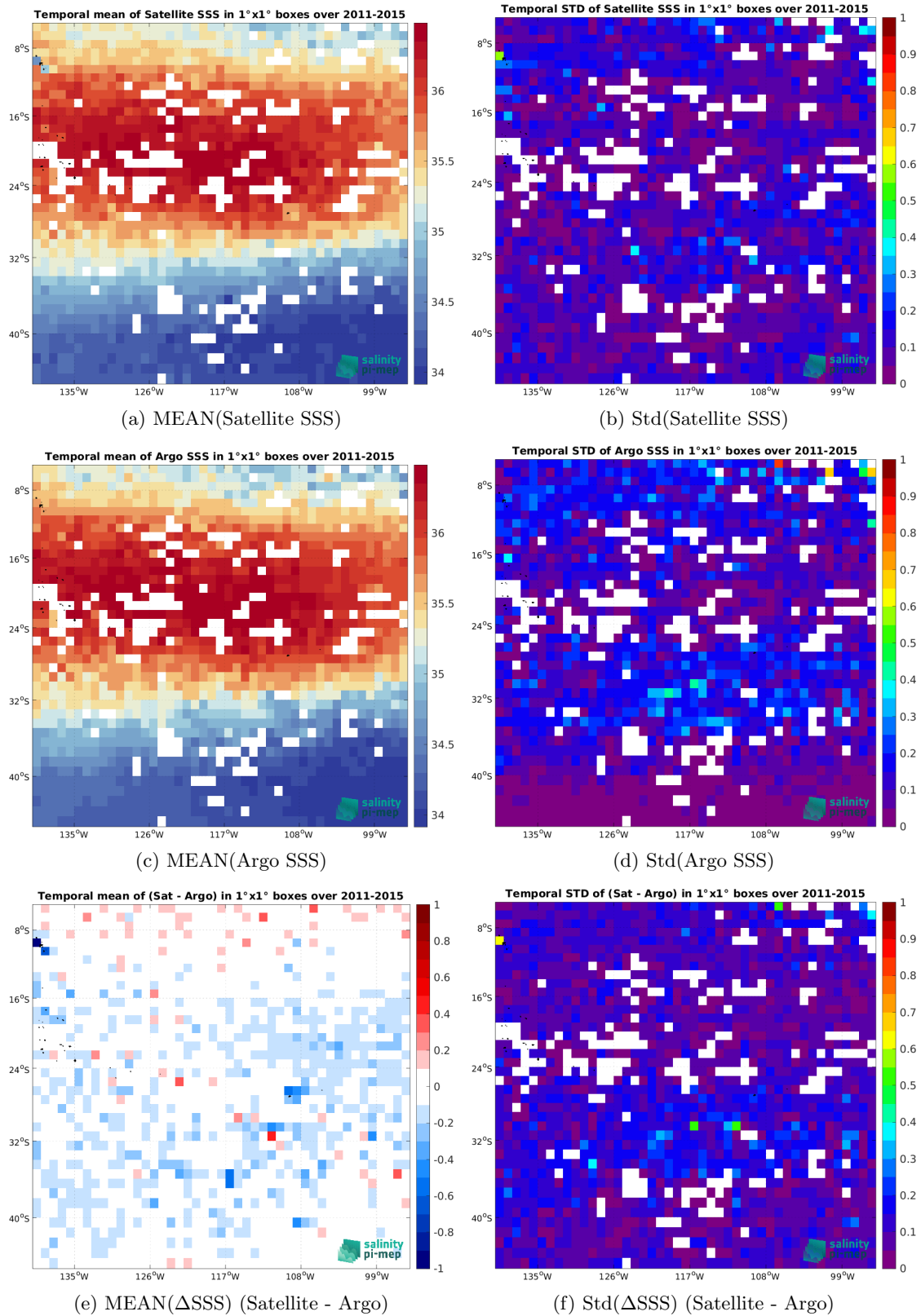
Figure 7: Temporal mean (left) and Std (right) of SSS from Aquarius SSS L3 OR v5 - Monthly - Rain mask (NASA-GSFC) (top), Argo (middle), and of \Delta SSS (Satellite - Argo). Only match-up pairs are used to generate these maps.
