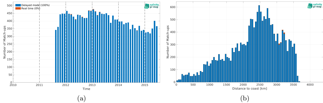
Figure 2: Number of match-ups between Argo and Aquarius SSS L3 OR v5 - Monthly - Rain mask (NASA-GSFC) SSS as a function of time (a) and as function of the distance to coast (b) over the OTT zone Pi-MEP region and for the full satellite product period.
