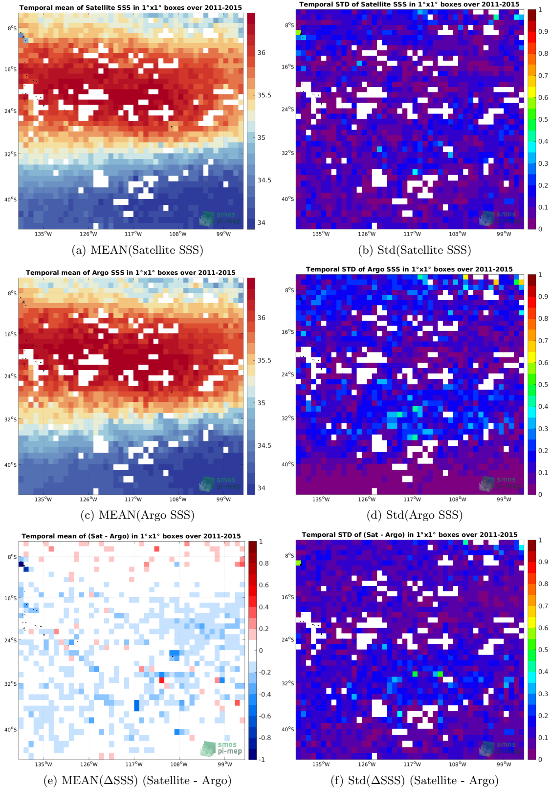
Figure 6: Temporal mean (left) and Std (right) of SSS from Aquarius SSS L3 OR v5 - Monthly - Rain mask (NASA-GSFC) (top), Argo (middle), and of \Delta SSS (Satellite - Argo). Only match-up pairs are used to generate these maps.
