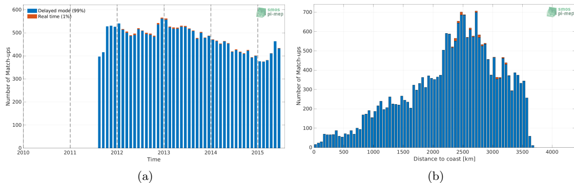
Figure 1: Number of match-ups between Argo and Aquarius SSS L3 OR v5 - Monthly - Rain mask (NASA-GSFC) SSS as a function of time (a) and as function of the distance to coast (b) over the OTT zone Pi-MEP region and for the full satellite product period.
