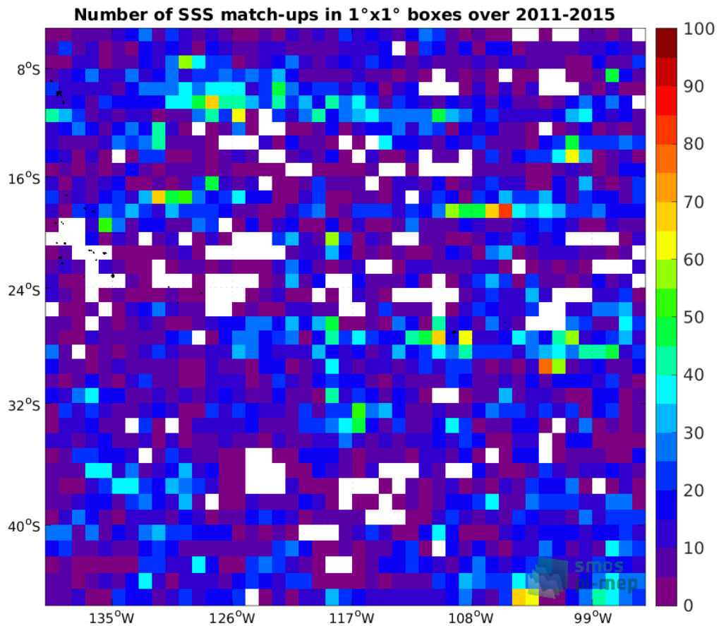
Figure 4: Number of SSS match-ups between Argo SSS and the Aquarius SSS L3 OR v5 - Monthly - Rain mask (NASA-GSFC) SSS product for the OTT zone Pi-MEP region over 1°x1° boxes and for the full satellite product period.
