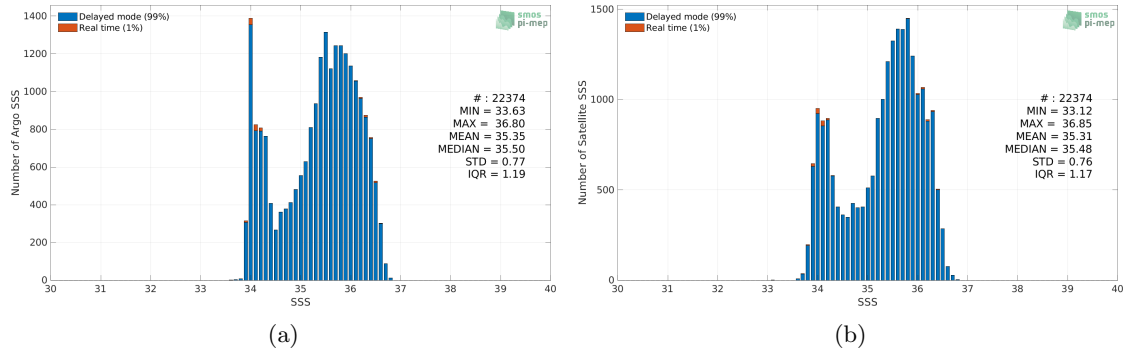
Figure 2: Histograms of SSS from Argo (a) and Aquarius SSS L3 OR v5 - Monthly - Rain mask (NASA-GSFC) (b) considering all match-up pairs per bins of 0.1 over the OTT zone Pi-MEP region and for the full satellite product period.
