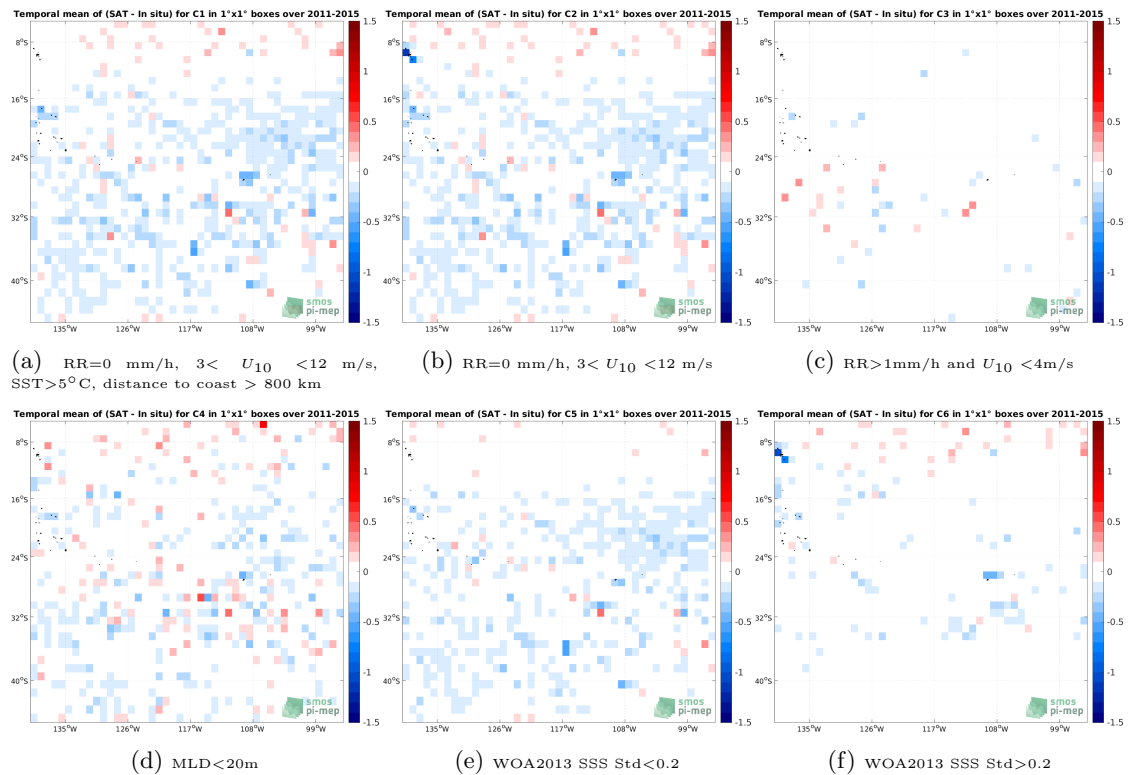
Figure 12: Temporal mean gridded over spatial boxes of size 1^\circ \times 1^\circ of \Delta SSS (Aquarius SSS L3 OR v5 - Monthly - Rain mask (NASA-GSFC) - Argo) for 6 different subdatasets corresponding to:RR=0 mm/h, 3 < U_{10} < 12 m/s, SST >5^\circ C, distance to coast > 800 km (a), RR=0 mm/h, 3 < U_{10} < 12 m/s (b), RR >1 mm/h and U_{10} < 4 m/s (c),MLD <20 m (d),WOA2013 SSS Std <0.2 (e),WOA2013 SSS Std >0.2 (f).
