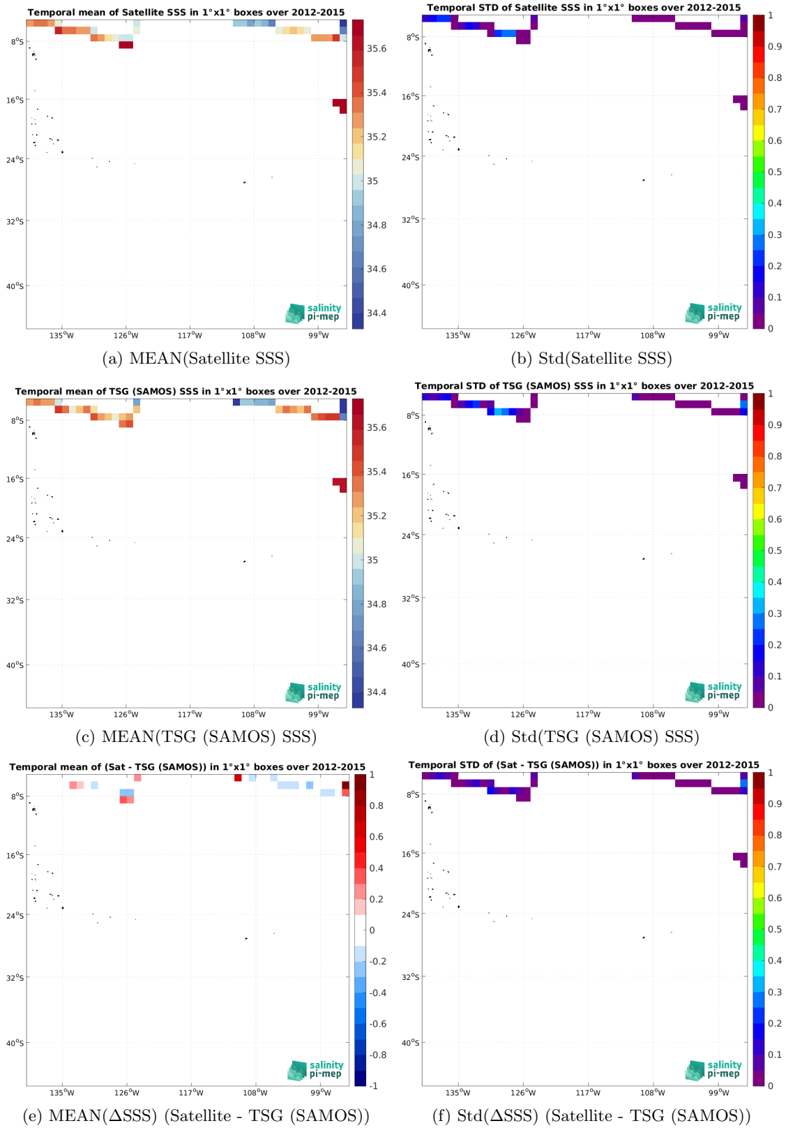
Figure 7: Temporal mean (left) and Std (right) of SSS from Aquarius SSS L3 CAP v5 - 7-Day running (JPL) (top), TSG (SAMOS) (middle), and of \Delta SSS (Satellite - TSG (SAMOS)). Only match-up pairs are used to generate these maps.
