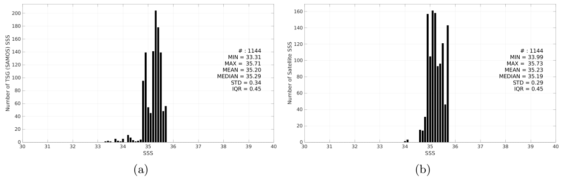
Figure 3: Histograms of SSS from TSG (SAMOS) (a) and Aquarius SSS L3 CAP v5 - 7-Day running (JPL) (b) considering all match-up pairs per bins of 0.1 over the OTT zone Pi-MEP region and for the full satellite product period.
