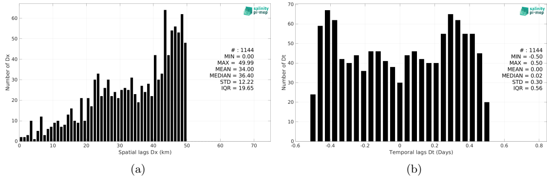
Figure 6: Histograms of the spatial (a) and temporal (b) lags between the location/time of the TSG (SAMOS) measurement and the date of the corresponding Aquarius SSS L3 CAP v5 - 7-Day running (JPL) SSS pixel.
