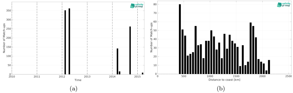
Figure 2: Number of match-ups between TSG (SAMOS) and Aquarius SSS L3 CAP v5 - 7-Day running (JPL) SSS as a function of time (a) and as function of the distance to coast (b) over the OTT zone Pi-MEP region and for the full satellite product period.
