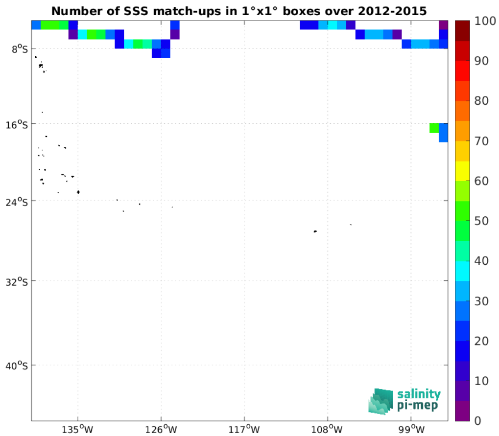
Figure 5: Number of SSS match-ups between TSG (SAMOS) SSS and the Aquarius SSS L3 CAP v5 - 7-Day running (JPL) SSS product for the OTT zone Pi-MEP region over 1^\circ \times 1^\circ boxes and for the full satellite product period.
