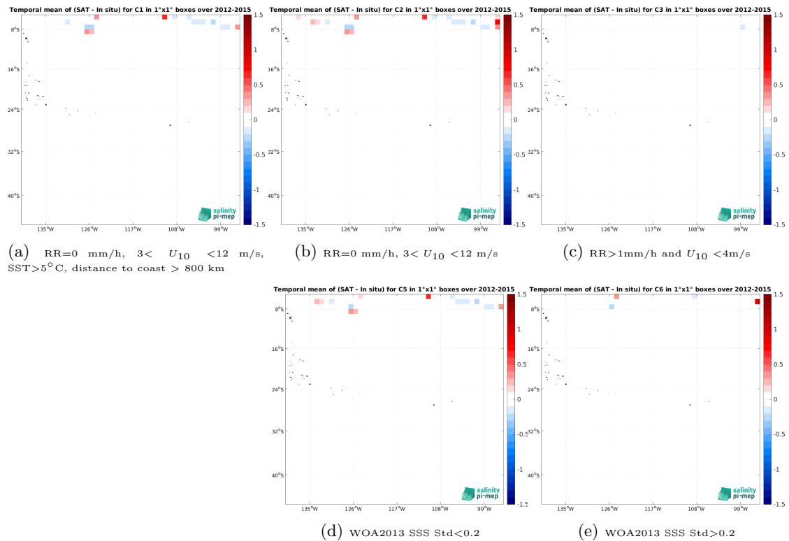
Figure 14: Temporal mean gridded over spatial boxes of size 1^\circ \times 1^\circ of \Delta SSS (Aquarius SSS L3 CAP v5 - 7-Day running (JPL) - TSG (SAMOS)) for 5 different subdatasets corresponding to: RR=0 mm/h, 3 < U_{10} < 12 m/s, SST > 5°C, distance to coast > 800 km (a), RR=0 mm/h, 3 < U_{10} < 12 m/s (b), RR > 1mm/h and U_{10} < 4 m/s (c), WOA2013 SSS Std < 0.2 (d), WOA2013 SSS Std > 0.2 (e).
