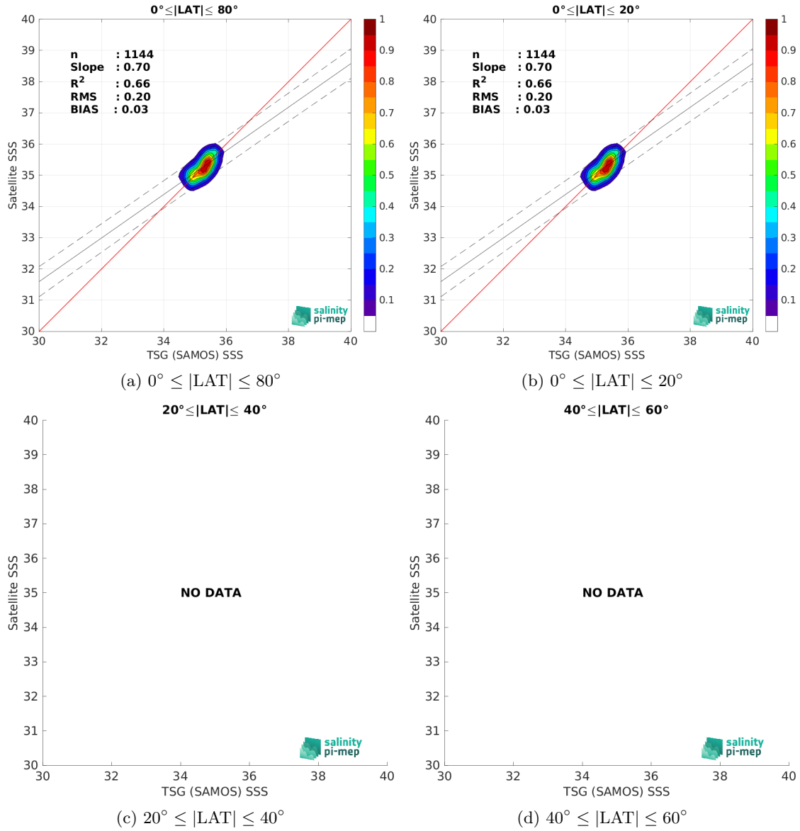
Figure 10: Contour maps of the concentration of Aquarius SSS L3 CAP v5 - 7-Day running (JPL) SSS ( y -axis) versus TSG (SAMOS) SSS ( x -axis) at match-up pairs for different latitude bands. For each plot, the red line shows x=y . The black thin and dashed lines indicate a linear fit through the data cloud and the \pm 95\% confidence levels, respectively. The number match-up pairs n , the slope and R^2 coefficient of the linear fit, the root mean square (RMS) and the mean bias between satellite and in situ data are indicated for each latitude band in each plots.
