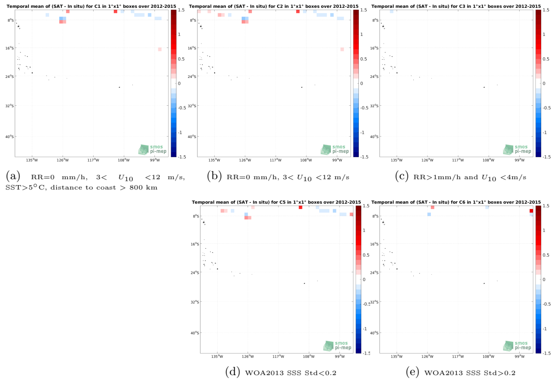
Figure 12: Temporal mean gridded over spatial boxes of size 1^\circ \times 1^\circ of \Delta\text{SSS} (Aquarius SSS L3 CAP v5 - 7-Day running (JPL) - TSG (SAMOS)) for 5 different subdatasets corresponding to:RR=0 mm/h, 3 < U_{10} < 12 m/s, SST >5^\circ\text{C} , distance to coast > 800 km (a), RR=0 mm/h, 3 < U_{10} < 12 m/s (b), RR >1 mm/h and U_{10} < 4 m/s (c), WOA2013 SSS Std <0.2 (d), WOA2013 SSS Std >0.2 (e).
