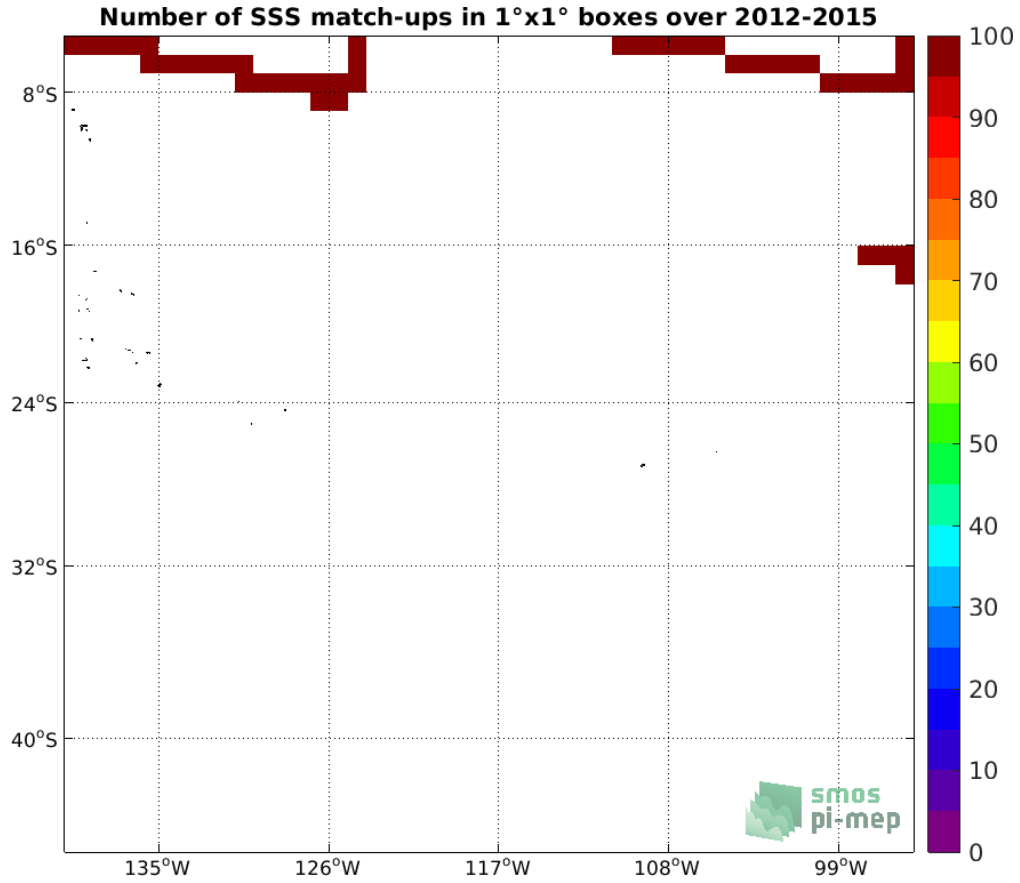
Figure 4: Number of SSS match-ups between TSG (SAMOS) SSS and the Aquarius SSS L3 CAP v5 - 7-Day running (JPL) SSS product for the OTT zone Pi-MEP region over 1°x1° boxes and for the full satellite product period.
