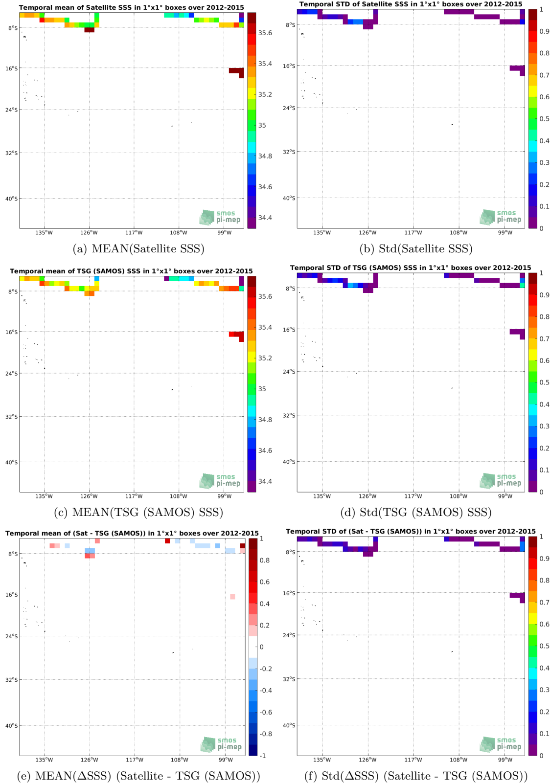
Figure 6: Temporal mean (left) and Std (right) of SSS from Aquarius SSS L3 CAP v5 - 7-Day running (JPL) (top), TSG (SAMOS) (middle), and of \Delta SSS (Satellite - TSG (SAMOS)). Only match-up pairs are used to generate these maps.
