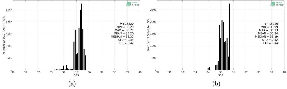
Figure 2: Histograms of SSS from TSG (SAMOS) (a) and Aquarius SSS L3 CAP v5 - 7-Day running (JPL) (b) considering all match-up pairs per bins of 0.1 over the OTT zone Pi-MEP region and for the full satellite product period.
