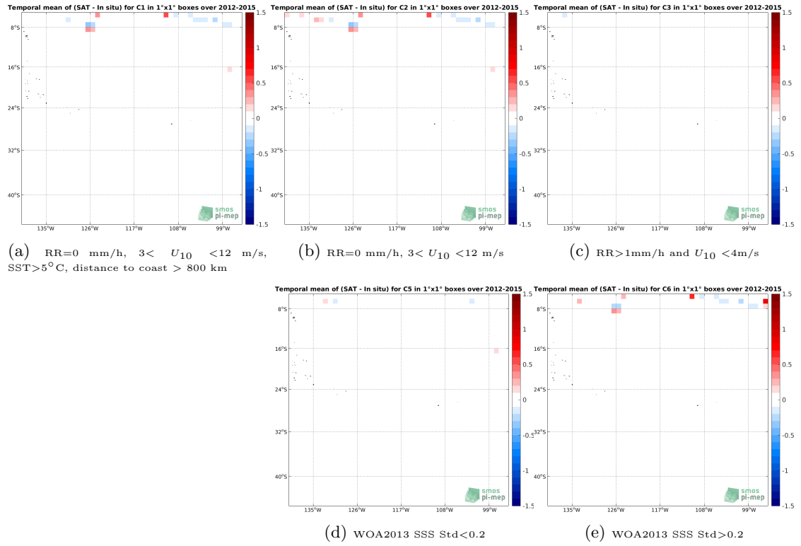
Figure 12: Temporal mean gridded over spatial boxes of size 1^\circ \times 1^\circ of \Delta SSS (Aquarius SSS L3 CAP v5 - 7-Day running (JPL) - TSG (SAMOS)) for 5 different subdatasets corresponding to: RR=0 mm/h, 3 < U_{10} < 12 m/s, SST>5°C, distance to coast > 800 km (a), RR=0 mm/h, 3 < U_{10} < 12 m/s (b), RR>1mm/h and U_{10} < 4 m/s (c), WOA2013 SSS Std<0.2 (d), WOA2013 SSS Std>0.2 (e).
