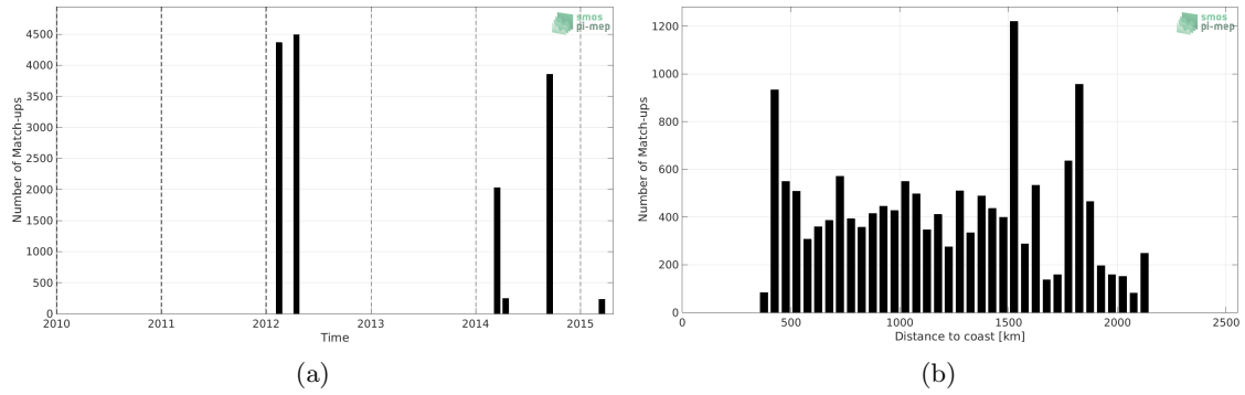
Figure 1: Number of match-ups between TSG (SAMOS) and Aquarius SSS L3 CAP v5 - 7-Day running (JPL) SSS as a function of time (a) and as function of the distance to coast (b) over the OTT zone Pi-MEP region and for the full satellite product period.
