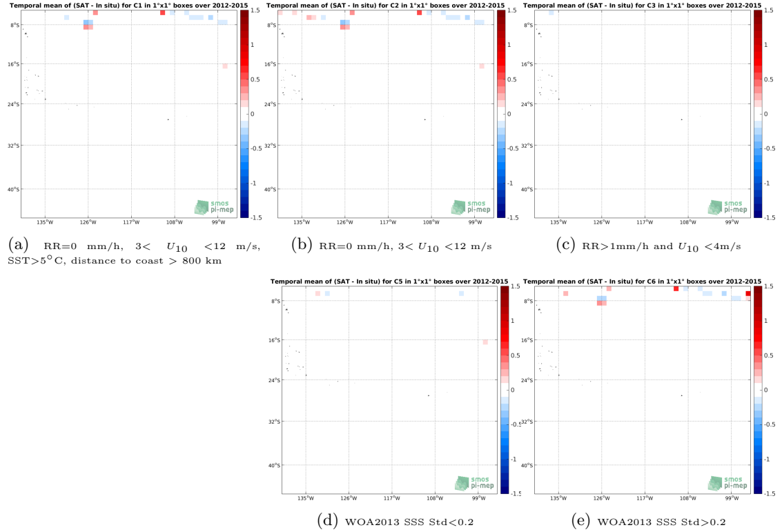
Figure 12: Temporal mean gridded over spatial boxes of size 1^\circ \times 1^\circ of \Delta SSS (Aquarius-L3-JPL-V5-7DAY-RUNNING - TSG-SAMOS) for 5 different subdatasets corresponding to: RR=0 mm/h, 3 < U_{10} < 12 m/s, SST > 5^\circ\text{C} , distance to coast > 800 km (a), RR=0 mm/h, 3 < U_{10} < 12 m/s (b), RR > 1 mm/h and U_{10} < 4 m/s (c), WOA2013 SSS Std < 0.2 (d), WOA2013 SSS Std > 0.2 (e).
