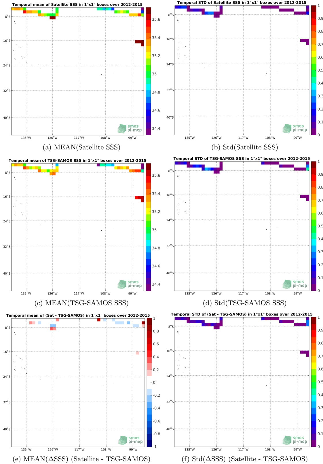
Figure 6: Temporal mean (left) and Std (right) of SSS from Aquarius-L3-JPL-V5-7DAY-RUNNING (top), TSG-SAMOS (middle), and of \Delta SSS (Satellite - TSG-SAMOS). Only match-up pairs are used to generate these maps.
