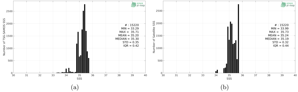
Figure 2: Histograms of SSS from TSG-SAMOS (a) and Aquarius-L3-JPL-V5-7DAY-RUNNING (b) considering all match-up pairs per bins of 0.1 over the OTT zone Pi-MEP region and for the full satellite product period.
