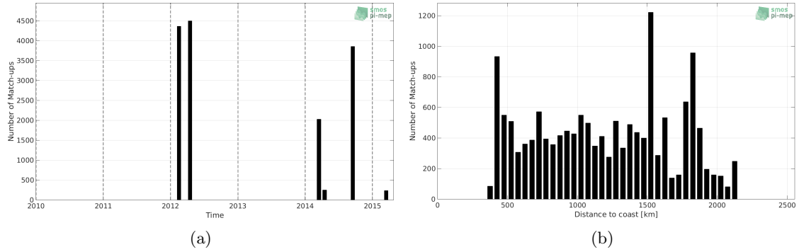
Figure 1: Number of match-ups between TSG-SAMOS and Aquarius-L3-JPL-V5-7DAY-RUNNING SSS as a function of time (a) and as function of the distance to coast (b) over the OTT zone Pi-MEP region and for the full satellite product period.
