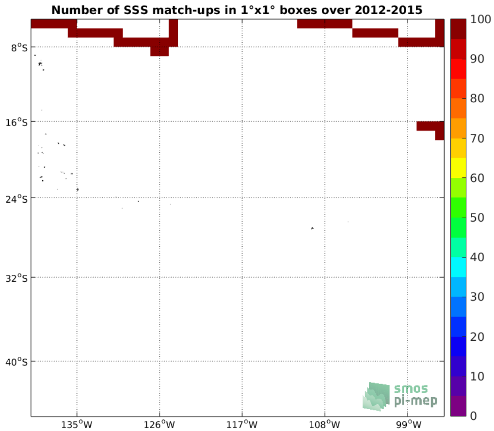
Figure 4: Number of SSS match-ups between TSG-SAMOS SSS and the Aquarius-L3-JPL-V5-7DAY-RUNNING SSS product for the OTT zone Pi-MEP region over 1°x1° boxes and for the full satellite product period.
