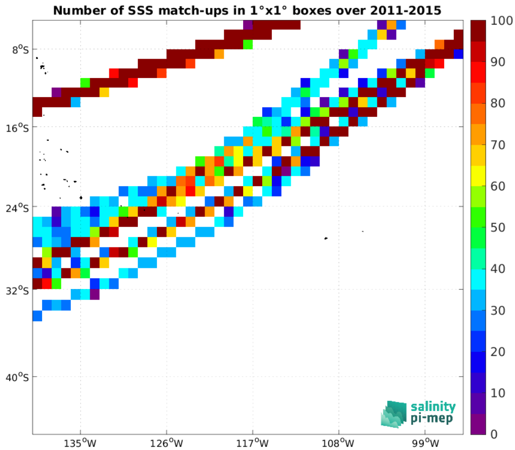
Figure 4: Number of SSS match-ups between TSG (LEGOS-DM) SSS and the Aquarius SSS L3 CAP v5 - 7-Day running (JPL) SSS product for the OTT zone Pi-MEP region over 1^\circ \times 1^\circ boxes and for the full satellite product period.
