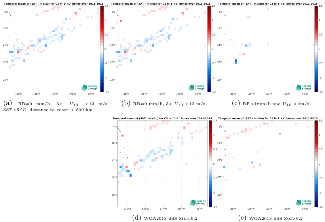
Figure 12: Temporal mean gridded over spatial boxes of size 1^\circ \times 1^\circ of \Delta\text{SSS} (Aquarius SSS L3 CAP v5 - 7-Day running (JPL) - TSG (LEGOS-DM)) for 5 different subdatasets corresponding to:RR=0 mm/h, 3 < U_{10} < 12 m/s, SST >5^\circ\text{C} , distance to coast > 800 km (a), RR=0 mm/h, 3 < U_{10} < 12 m/s (b), RR >1 mm/h and U_{10} < 4 m/s (c), WOA2013 SSS Std <0.2 (d), WOA2013 SSS Std >0.2 (e).
