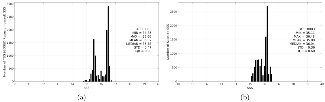
Figure 3: Histograms of SSS from TSG (GOSUD-Research-vessel) (a) and Aquarius SSS L3 CAP v5 - 7-Day running (JPL) (b) considering all match-up pairs per bins of 0.1 over the OTT zone Pi-MEP region and for the full satellite product period.
