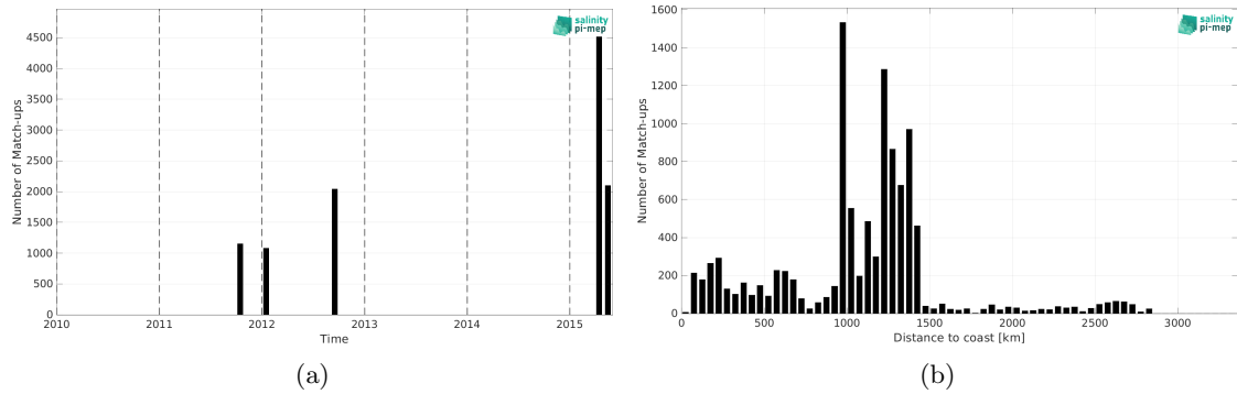
Figure 2: Number of match-ups between TSG (GOSUD-Research-vessel) and Aquarius SSS L3 CAP v5 - 7-Day running (JPL) SSS as a function of time (a) and as function of the distance to coast (b) over the OTT zone Pi-MEP region and for the full satellite product period.
