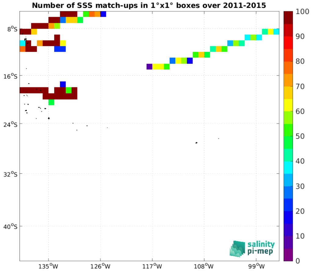
Figure 5: Number of SSS match-ups between TSG (GOSUD-Research-vessel) SSS and the Aquarius SSS L3 CAP v5 - 7-Day running (JPL) SSS product for the OTT zone Pi-MEP region over 1°x1° boxes and for the full satellite product period.
