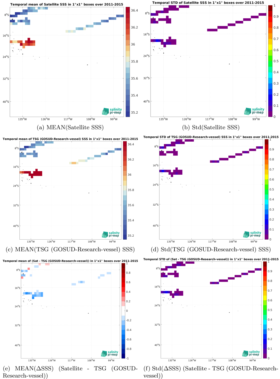
Figure 7: Temporal mean (left) and Std (right) of SSS from Aquarius SSS L3 CAP v5 - 7-Day running (JPL) (top), TSG (GOSUD-Research-vessel) (middle), and of \Delta SSS (Satellite - TSG (GOSUD-Research-vessel)). Only match-up pairs are used to generate these maps.
