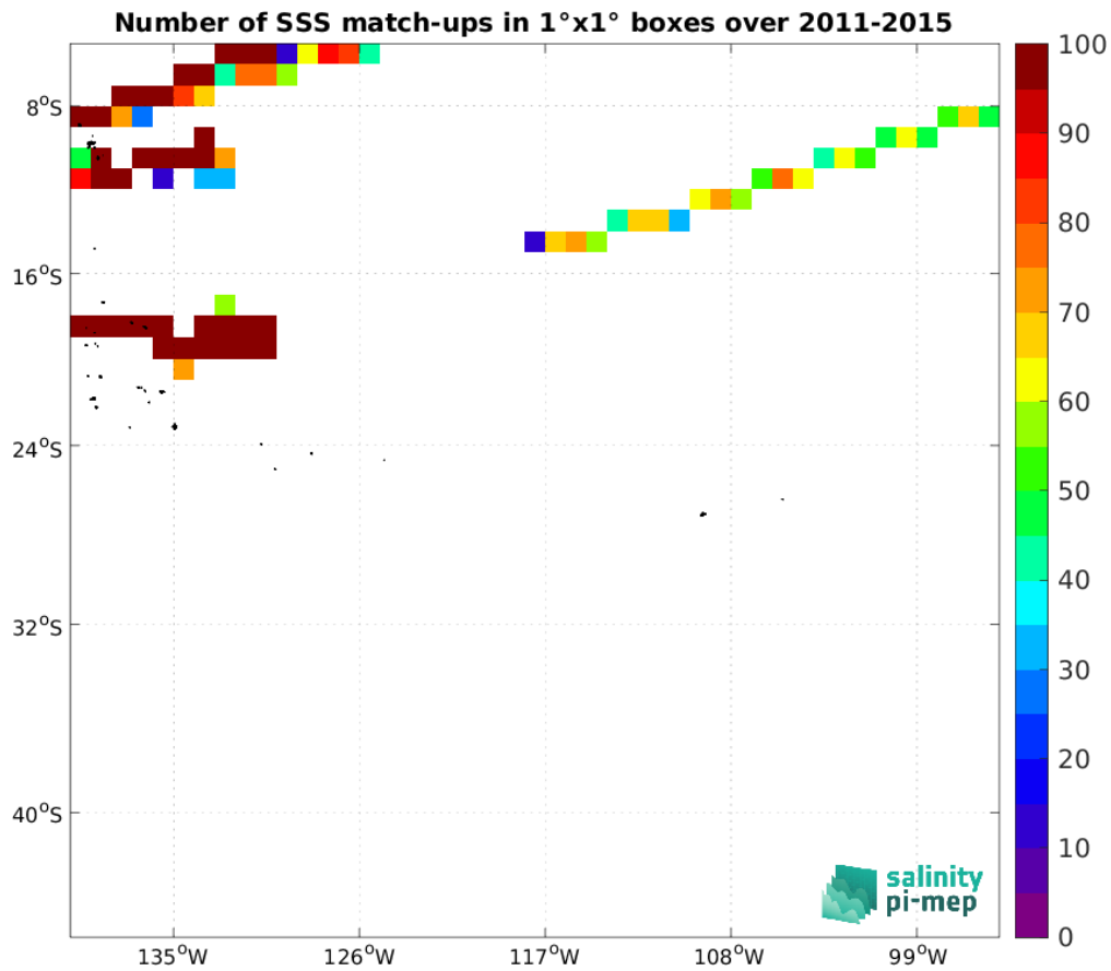
Figure 4: Number of SSS match-ups between TSG (GOSUD-Research-vessel) SSS and the Aquarius SSS L3 CAP v5 - 7-Day running (JPL) SSS product for the OTT zone Pi-MEP region over 1^\circ \times 1^\circ boxes and for the full satellite product period.
