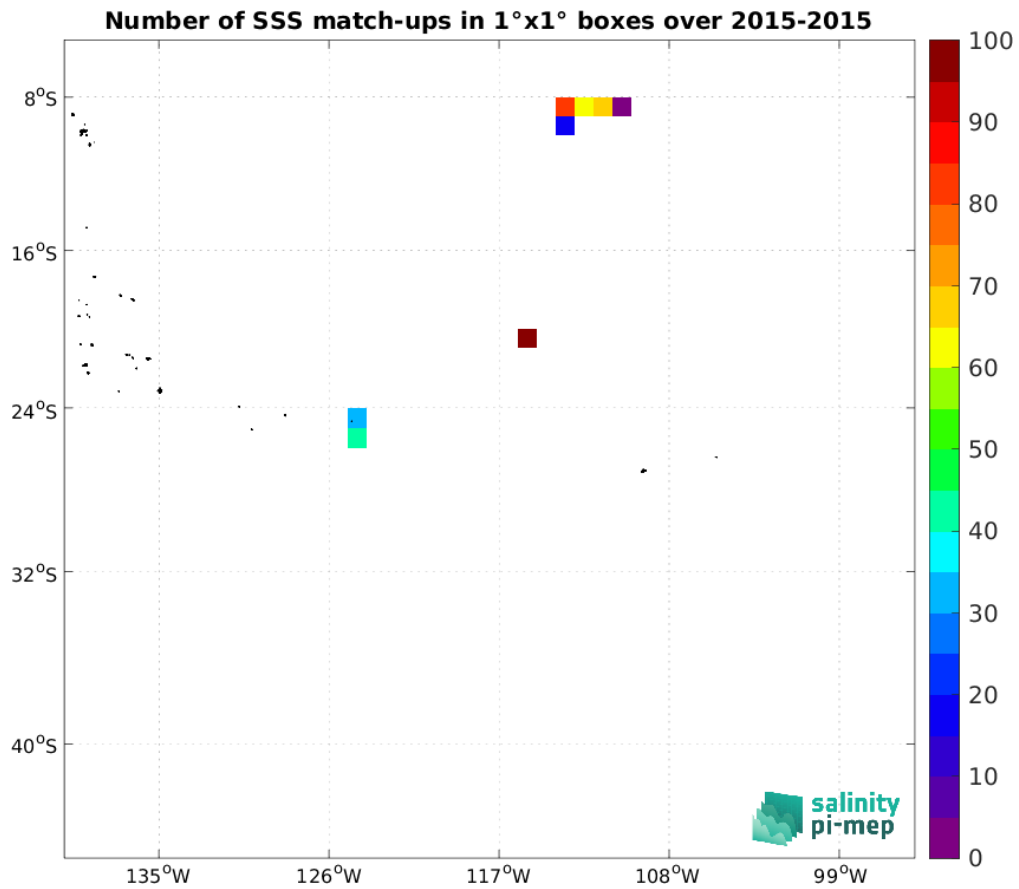
Figure 4: Number of SSS match-ups between Surface drifters SSS and the Aquarius SSS L3 CAP v5 - 7-Day running (JPL) SSS product for the OTT zone Pi-MEP region over 1°x1° boxes and for the full satellite product period.
