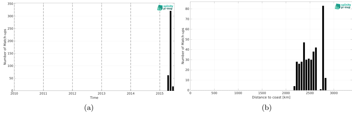
Figure 2: Number of match-ups between Surface drifters and Aquarius SSS L3 CAP v5 - 7-Day running (JPL) SSS as a function of time (a) and as function of the distance to coast (b) over the OTT zone Pi-MEP region and for the full satellite product period.
