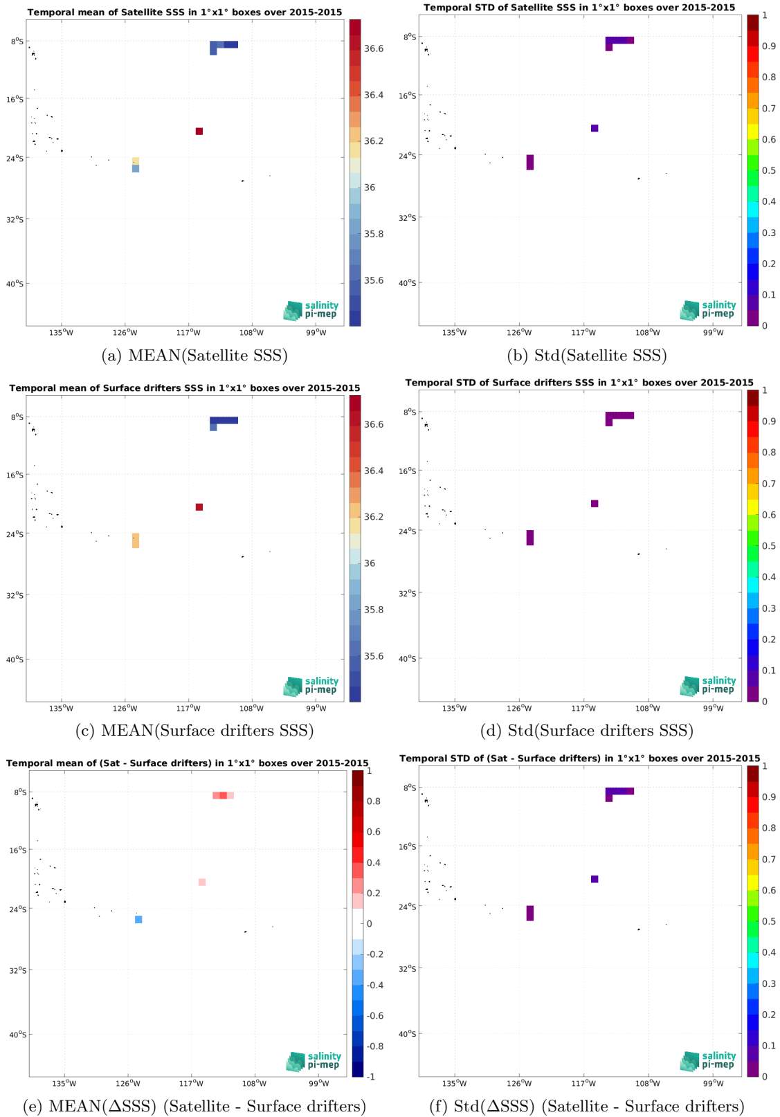
Figure 6: Temporal mean (left) and Std (right) of SSS from Aquarius SSS L3 CAP v5 - 7-Day running (JPL) (top), Surface drifters (middle), and of \Delta SSS (Satellite - Surface drifters). Only match-up pairs are used to generate these maps.
