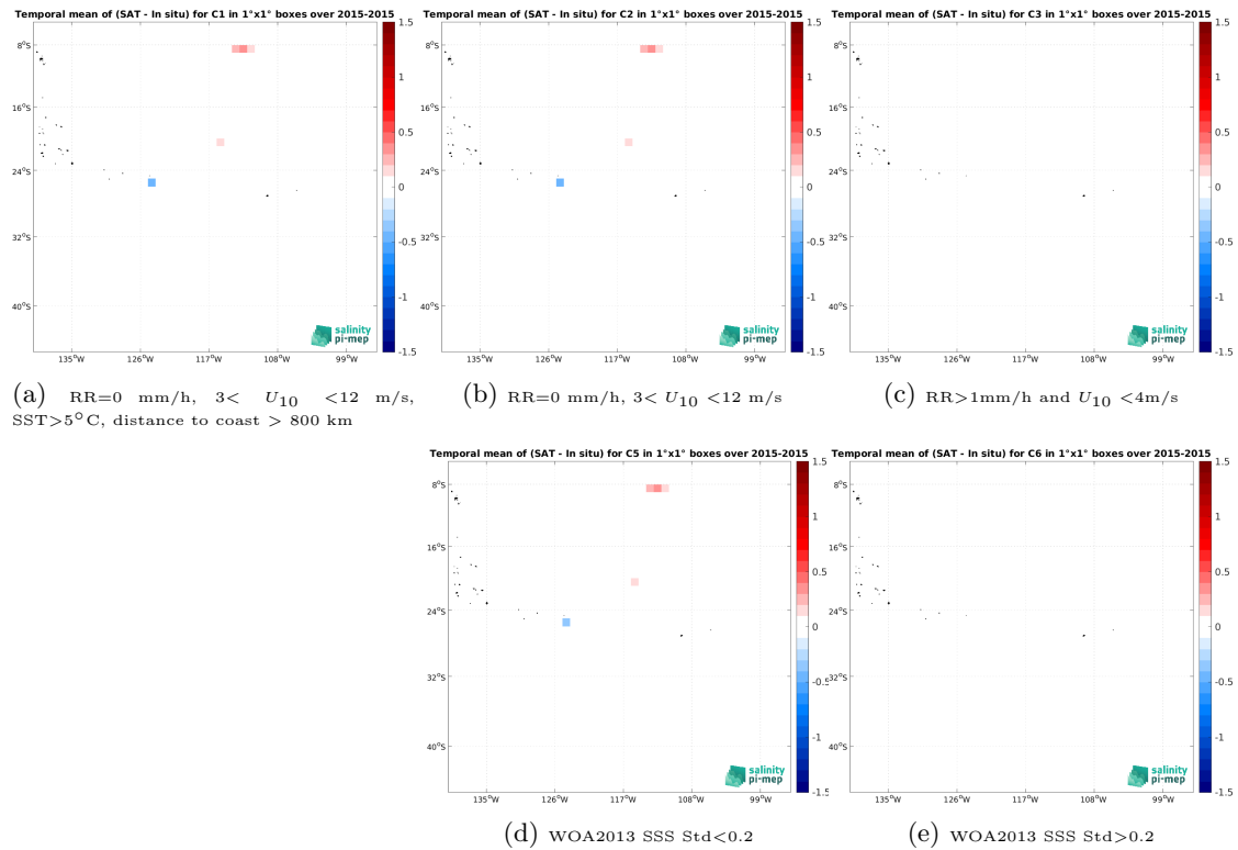
Figure 13: Temporal mean gridded over spatial boxes of size 1^\circ \times 1^\circ of \Delta SSS (Aquarius SSS L3 CAP v5 - 7-Day running (JPL) - Surface drifters) for 5 different subdatasets corresponding to: RR=0 mm/h, 3 < U_{10} < 12 m/s, SST >5^\circ C, distance to coast > 800 km (a), RR=0 mm/h, 3 < U_{10} < 12 m/s (b), RR >1 mm/h and U_{10} < 4 m/s (c), WOA2013 SSS Std <0.2 (d), WOA2013 SSS Std >0.2 (e).
