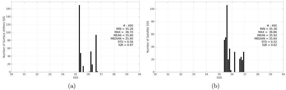
Figure 3: Histograms of SSS from Surface drifters (a) and Aquarius SSS L3 CAP v5 - 7-Day running (JPL) (b) considering all match-up pairs per bins of 0.1 over the OTT zone Pi-MEP region and for the full satellite product period.
