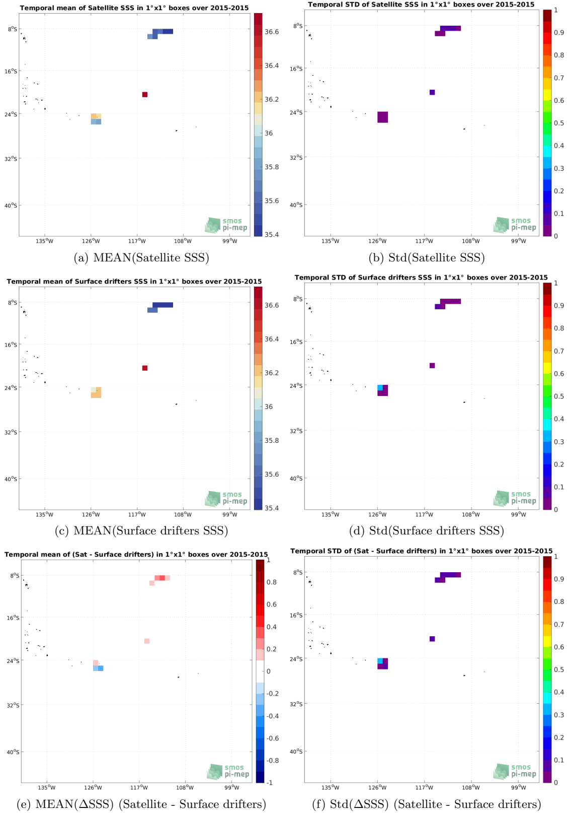
Figure 5: Temporal mean (left) and Std (right) of SSS from Aquarius SSS L3 CAP v5 - 7-Day running (JPL) (top), Surface drifters (middle), and of \Delta SSS (Satellite - Surface drifters). Only match-up pairs are used to generate these maps.
