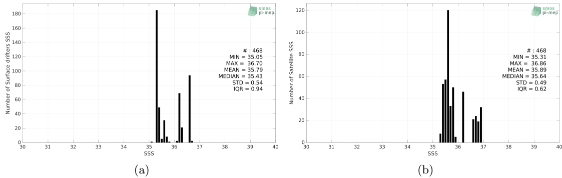
Figure 2: Histograms of SSS from Surface drifters (a) and Aquarius SSS L3 CAP v5 - 7-Day running (JPL) (b) considering all match-up pairs per bins of 0.1 over the OTT zone Pi-MEP region and for the full satellite product period.
