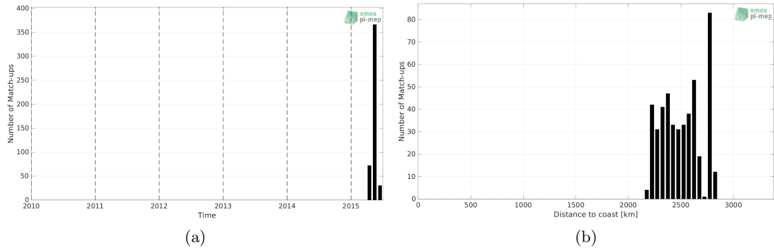
Figure 1: Number of match-ups between Surface drifters and Aquarius SSS L3 CAP v5 - 7-Day running (JPL) SSS as a function of time (a) and as function of the distance to coast (b) over the OTT zone Pi-MEP region and for the full satellite product period.
