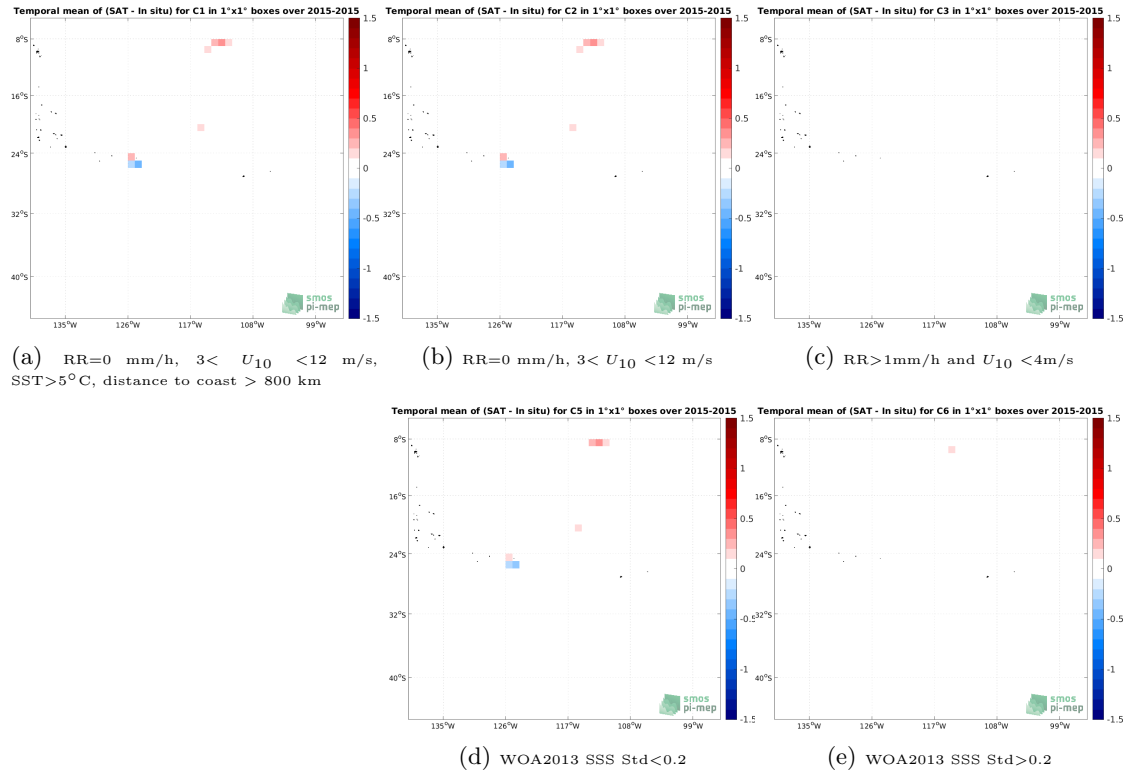
Figure 11: Temporal mean gridded over spatial boxes of size 1^\circ \times 1^\circ of \Delta\text{SSS} (Aquarius SSS L3 CAP v5 - 7-Day running (JPL) - Surface drifters) for 5 different subdatasets corresponding to:RR=0 mm/h, 3 < U_{10} < 12 m/s, SST >5^\circ\text{C} , distance to coast > 800 km (a), RR=0 mm/h, 3 < U_{10} < 12 m/s (b), RR >1 mm/h and U_{10} < 4 m/s (c), WOA2013 SSS Std <0.2 (d), WOA2013 SSS Std >0.2 (e).
