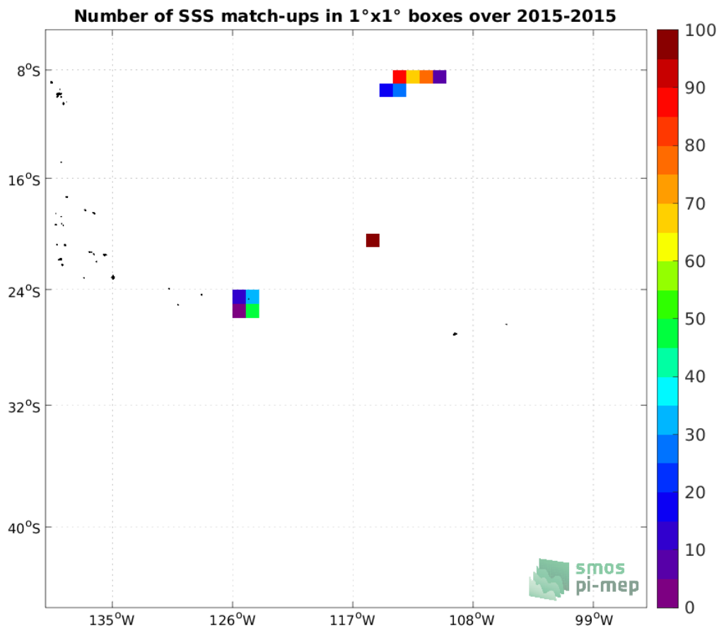
Figure 3: Number of SSS match-ups between Surface drifters SSS and the Aquarius SSS L3 CAP v5 - 7-Day running (JPL) SSS product for the OTT zone Pi-MEP region over 1^\circ \times 1^\circ boxes and for the full satellite product period.
