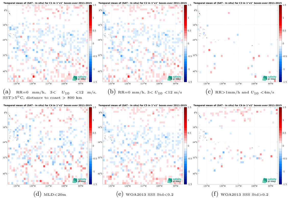
Figure 14: Temporal mean gridded over spatial boxes of size 1^\circ \times 1^\circ of \Delta SSS (Aquarius SSS L3 CAP v5 - 7-Day running (JPL) - Argo) for 6 different subdatasets corresponding to: RR=0 mm/h, 3 < U_{10} < 12 m/s, SST > 5^\circ C , distance to coast > 800 km (a), RR=0 mm/h, 3 < U_{10} < 12 m/s (b), RR > 1 mm/h and U_{10} < 4 m/s (c), MLD < 20 m (d), WOA2013 SSS Std < 0.2 (e), WOA2013 SSS Std > 0.2 (f).
