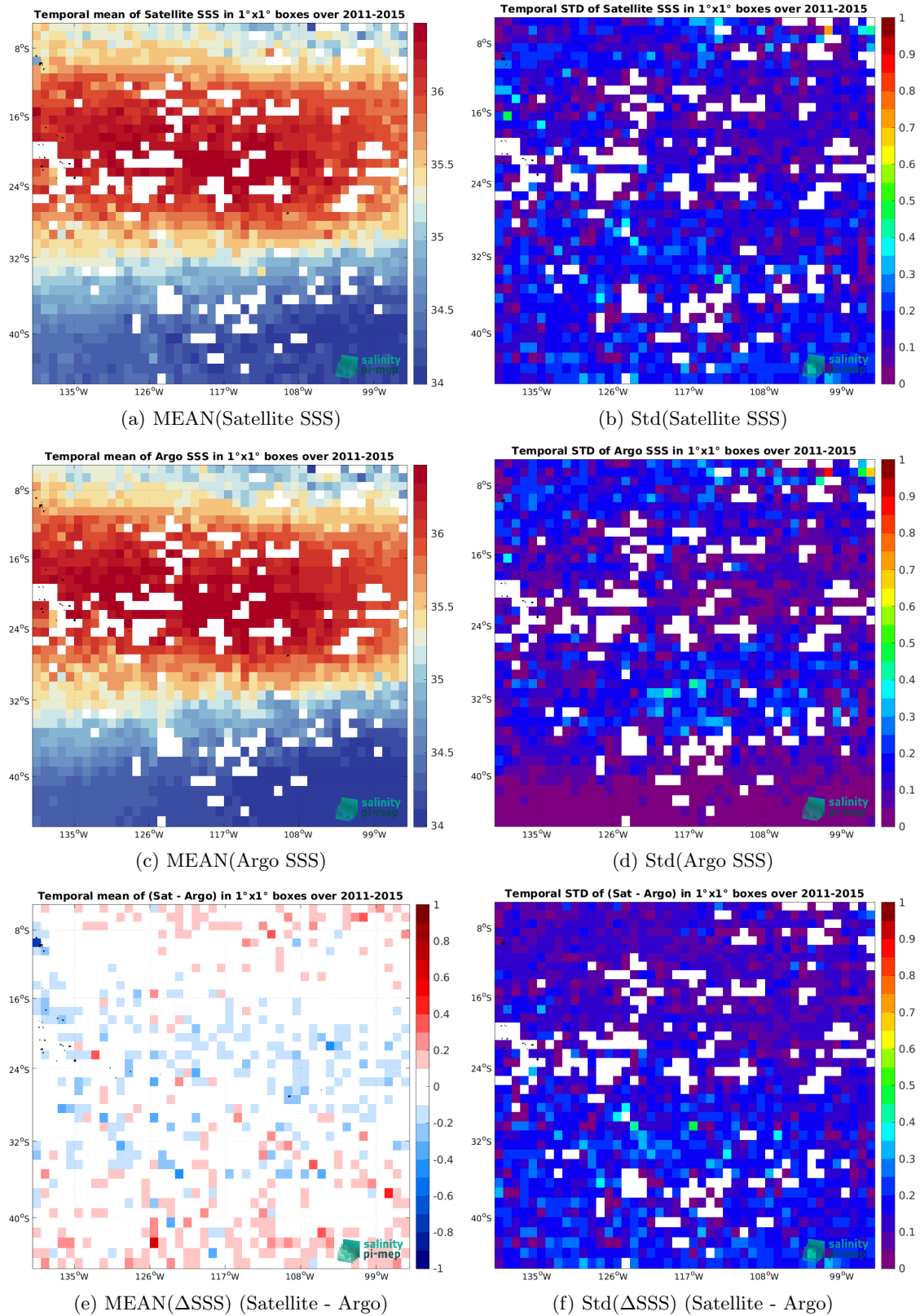
Figure 7: Temporal mean (left) and Std (right) of SSS from Aquarius SSS L3 CAP v5 - 7-Day running (JPL) (top), Argo (middle), and of \Delta SSS (Satellite - Argo). Only match-up pairs are used to generate these maps.
