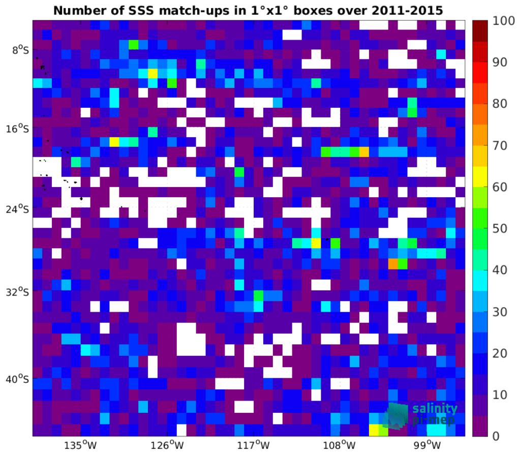
Figure 5: Number of SSS match-ups between Argo SSS and the Aquarius SSS L3 CAP v5 - 7-Day running (JPL) SSS product for the OTT zone Pi-MEP region over 1°x1° boxes and for the full satellite product period.
