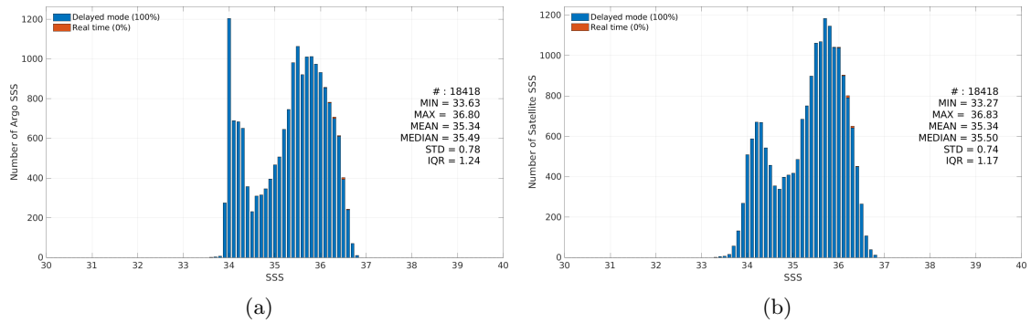
Figure 3: Histograms of SSS from Argo (a) and Aquarius SSS L3 CAP v5 - 7-Day running (JPL) (b) considering all match-up pairs per bins of 0.1 over the OTT zone Pi-MEP region and for the full satellite product period.
