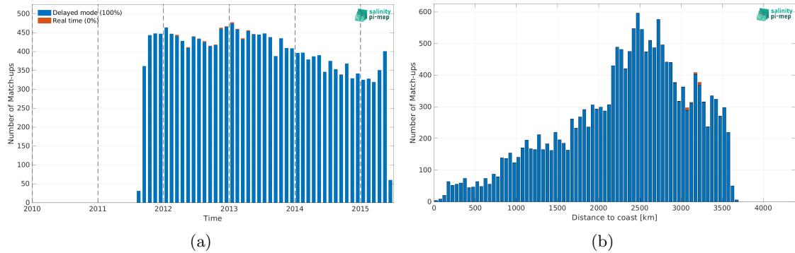
Figure 2: Number of match-ups between Argo and Aquarius SSS L3 CAP v5 - 7-Day running (JPL) SSS as a function of time (a) and as function of the distance to coast (b) over the OTT zone Pi-MEP region and for the full satellite product period.
