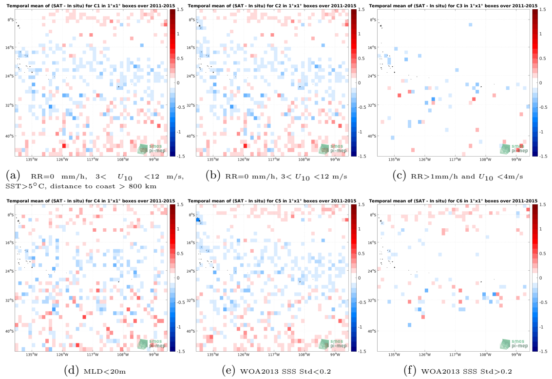
Figure 12: Temporal mean gridded over spatial boxes of size 1^\circ \times 1^\circ of \Delta SSS (Aquarius SSS L3 CAP v5 - 7-Day running (JPL) - Argo) for 6 different subdatasets corresponding to:RR=0 mm/h, 3 < U_{10} < 12 m/s, SST > 5^\circ\text{C} , distance to coast > 800 km (a), RR=0 mm/h, 3 < U_{10} < 12 m/s (b), RR > 1 mm/h and U_{10} < 4 m/s (c),MLD < 20 m (d),WOA2013 SSS Std < 0.2 (e),WOA2013 SSS Std > 0.2 (f).
