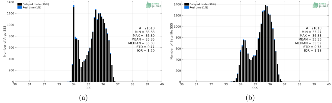
Figure 2: Histograms of SSS from Argo (a) and Aquarius SSS L3 CAP v5 - 7-Day running (JPL) (b) considering all match-up pairs per bins of 0.1 over the OTT zone Pi-MEP region and for the full satellite product period.
