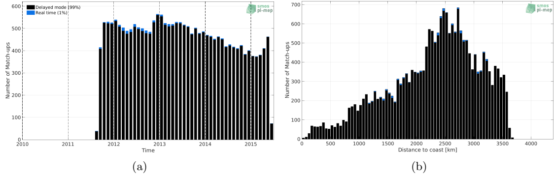
Figure 1: Number of match-ups between Argo and Aquarius SSS L3 CAP v5 - 7-Day running (JPL) SSS as a function of time (a) and as function of the distance to coast (b) over the OTT zone Pi-MEP region and for the full satellite product period.
