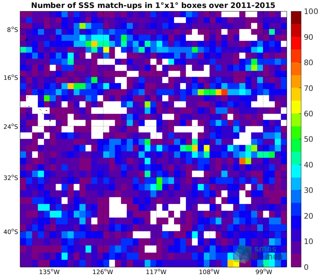
Figure 4: Number of SSS match-ups between Argo SSS and the Aquarius SSS L3 CAP v5 - 7-Day running (JPL) SSS product for the OTT zone Pi-MEP region over 1°x1° boxes and for the full satellite product period.
