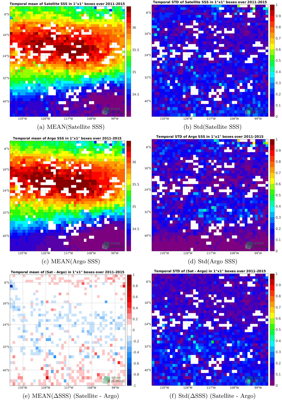
Figure 6: Temporal mean (left) and Std (right) of SSS from Aquarius SSS L3 CAP v5 - 7-Day running (JPL) (top), Argo (middle), and of \Delta SSS (Satellite - Argo). Only match-up pairs are used to generate these maps.
