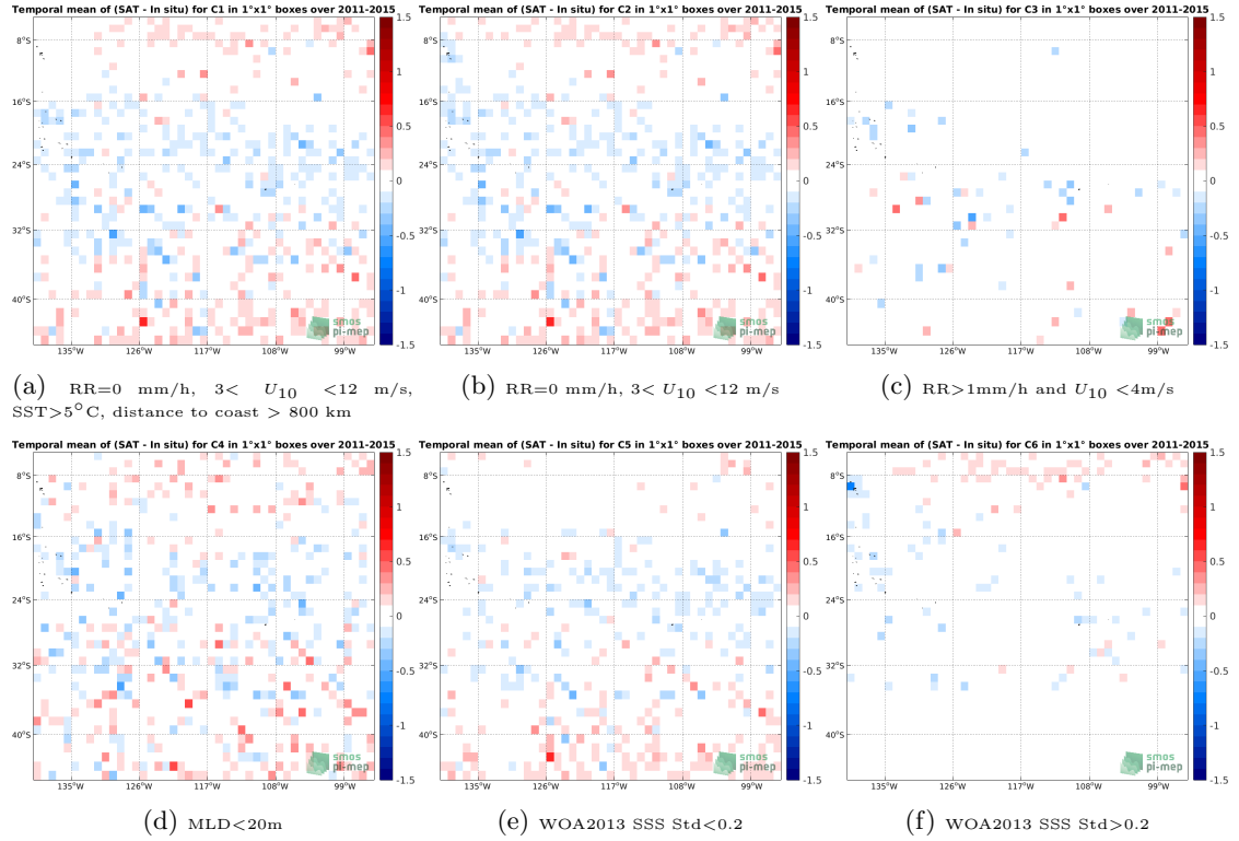
Figure 12: Temporal mean gridded over spatial boxes of size 1^\circ \times 1^\circ of \Delta SSS (Aquarius SSS L3 CAP v5 - 7-Day running (JPL) - Argo) for 6 different subdatasets corresponding to: RR=0 mm/h, 3 < U_{10} < 12 m/s, SST >5^\circ C, distance to coast > 800 km (a), RR=0 mm/h, 3 < U_{10} < 12 m/s (b), RR >1 mm/h and U_{10} < 4 m/s (c), MLD <20 m (d), WOA2013 SSS Std <0.2 (e), WOA2013 SSS Std >0.2 (f).
