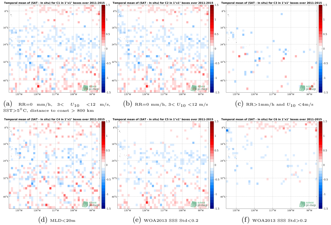
Figure 12: Temporal mean gridded over spatial boxes of size 1^\circ \times 1^\circ of \Delta SSS (Aquarius-L3-JPL-V5-7DAY-RUNNING - Argo) for 6 different subdatasets corresponding to: RR=0 mm/h, 3 < U_{10} < 12 m/s, SST >5^\circ C, distance to coast > 800 km (a), RR=0 mm/h, 3 < U_{10} < 12 m/s (b), RR >1 mm/h and U_{10} < 4 m/s (c), MLD <20 m (d), WOA2013 SSS Std <0.2 (e), WOA2013 SSS Std >0.2 (f).
