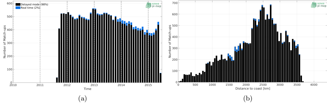
Figure 1: Number of match-ups between Argo and Aquarius-L3-JPL-V5-7DAY-RUNNING SSS as a function of time (a) and as function of the distance to coast (b) over the OTT zone Pi-MEP region and for the full satellite product period.
