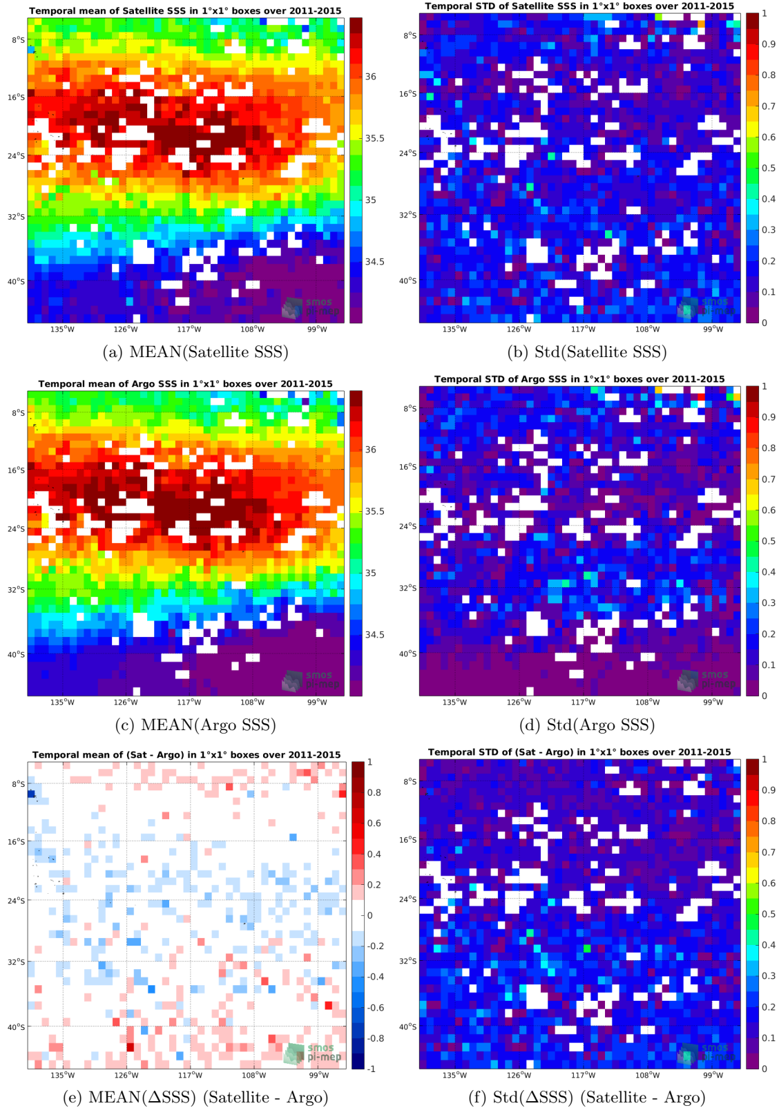
Figure 6: Temporal mean (left) and Std (right) of SSS from Aquarius-L3-JPL-V5-7DAY-RUNNING (top), Argo (middle), and of \Delta SSS (Satellite - Argo). Only match-up pairs are used to generate these maps.
