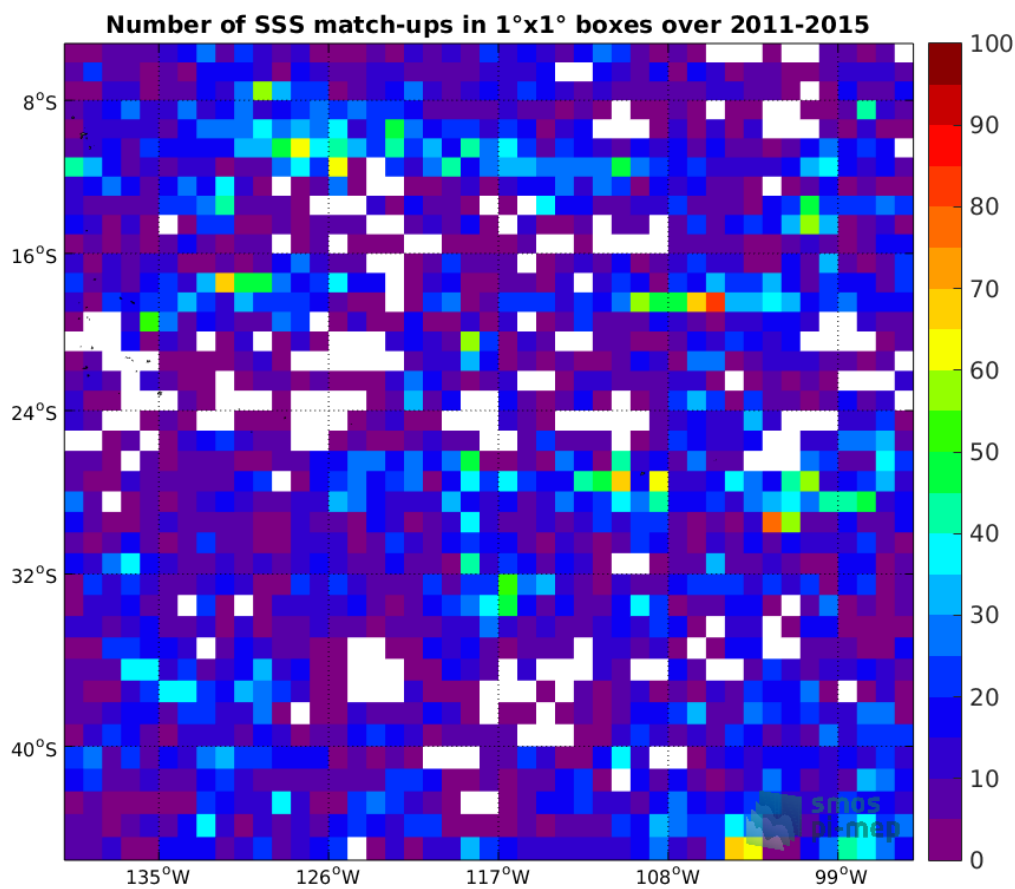
Figure 4: Number of SSS match-ups between Argo SSS and the Aquarius-L3-JPL-V5-7DAY-RUNNING SSS product for the OTT zone Pi-MEP region over 1°x1° boxes and for the full satellite product period.
