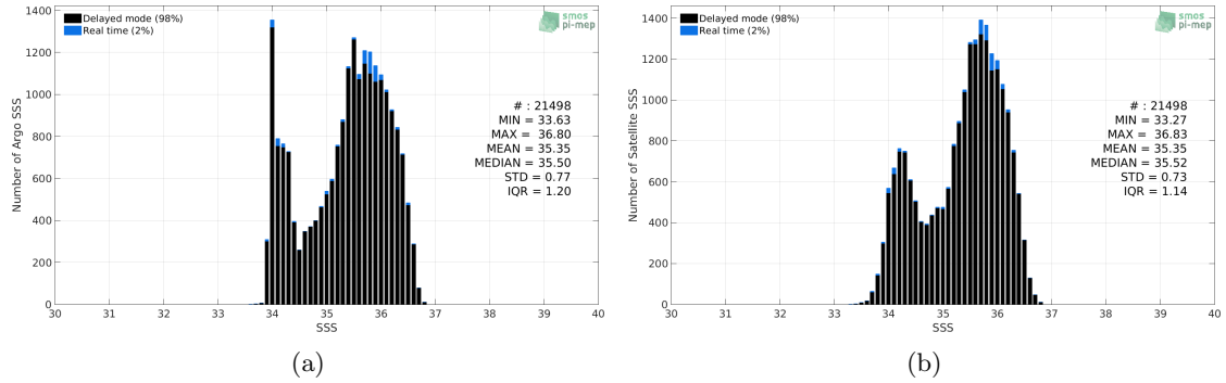
Figure 2: Histograms of SSS from Argo (a) and Aquarius-L3-JPL-V5-7DAY-RUNNING (b) considering all match-up pairs per bins of 0.1 over the OTT zone Pi-MEP region and for the full satellite product period.
