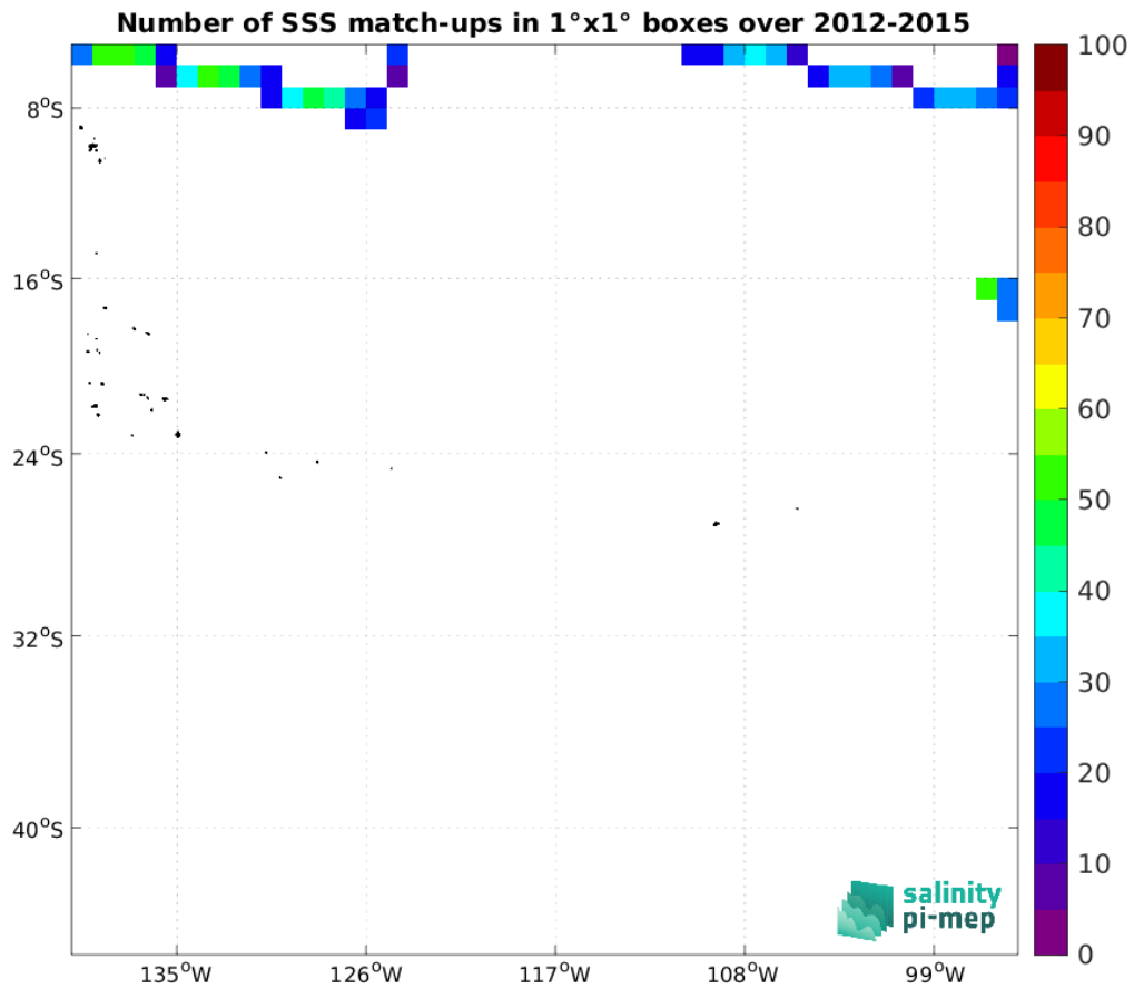
Figure 5: Number of SSS match-ups between TSG (SAMOS) SSS and the Aquarius SSS L3 CAP v5 - Monthly (JPL) SSS product for the OTT zone Pi-MEP region over 1^\circ \times 1^\circ boxes and for the full satellite product period.
