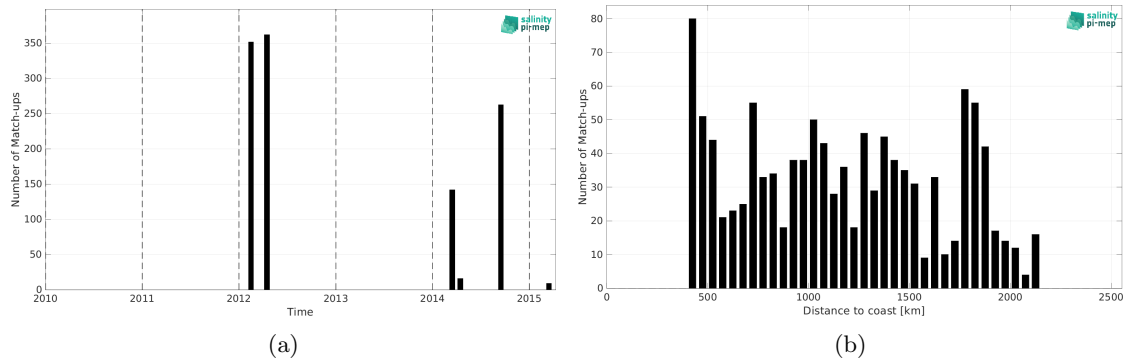
Figure 2: Number of match-ups between TSG (SAMOS) and Aquarius SSS L3 CAP v5 - Monthly (JPL) SSS as a function of time (a) and as function of the distance to coast (b) over the OTT zone Pi-MEP region and for the full satellite product period.
