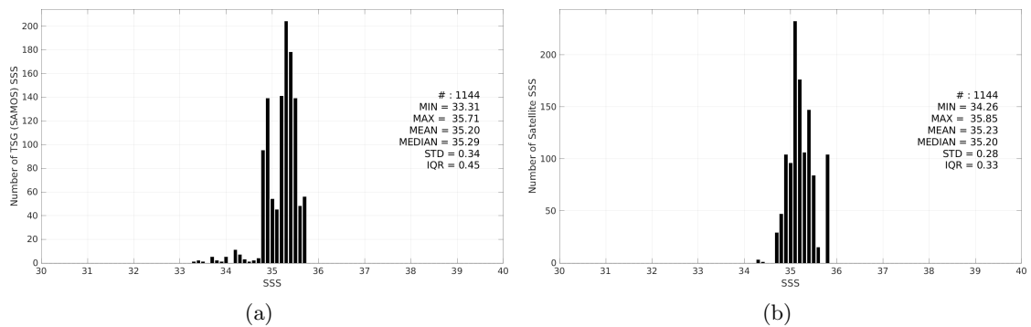
Figure 3: Histograms of SSS from TSG (SAMOS) (a) and Aquarius SSS L3 CAP v5 - Monthly (JPL) (b) considering all match-up pairs per bins of 0.1 over the OTT zone Pi-MEP region and for the full satellite product period.
