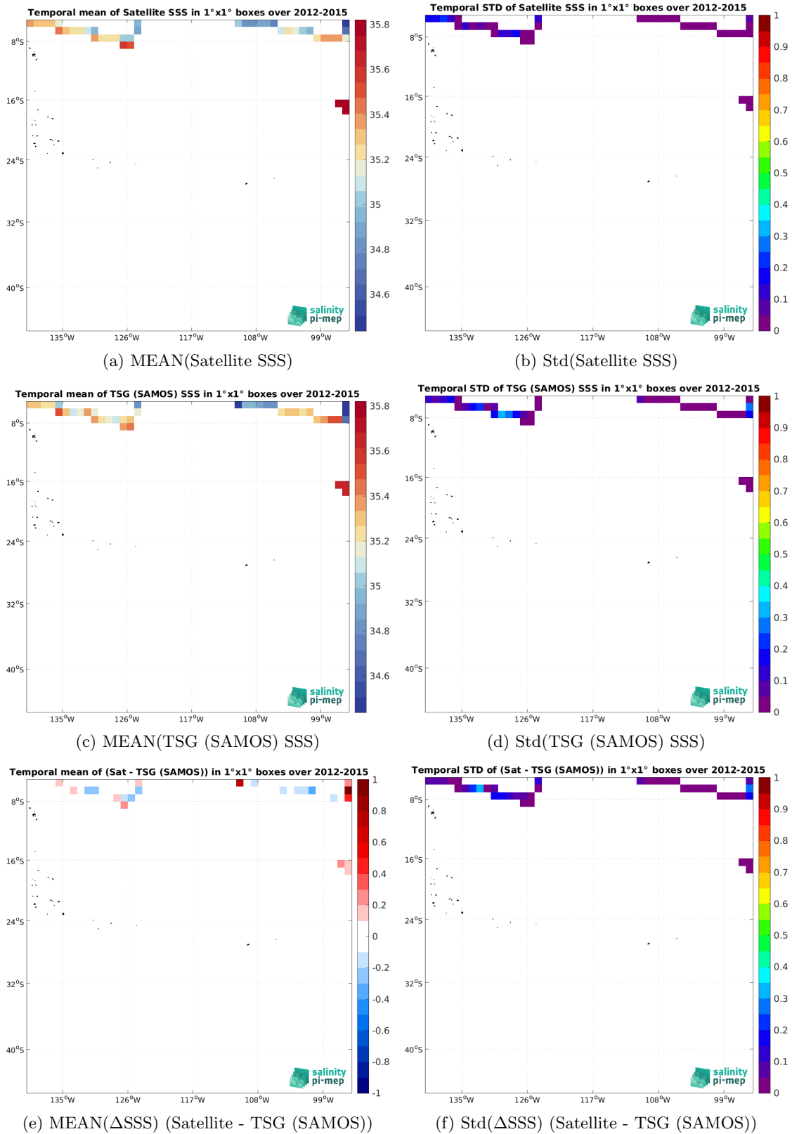
Figure 7: Temporal mean (left) and Std (right) of SSS from Aquarius SSS L3 CAP v5 - Monthly (JPL) (top), TSG (SAMOS) (middle), and of \Delta SSS (Satellite - TSG (SAMOS)). Only match-up pairs are used to generate these maps.
