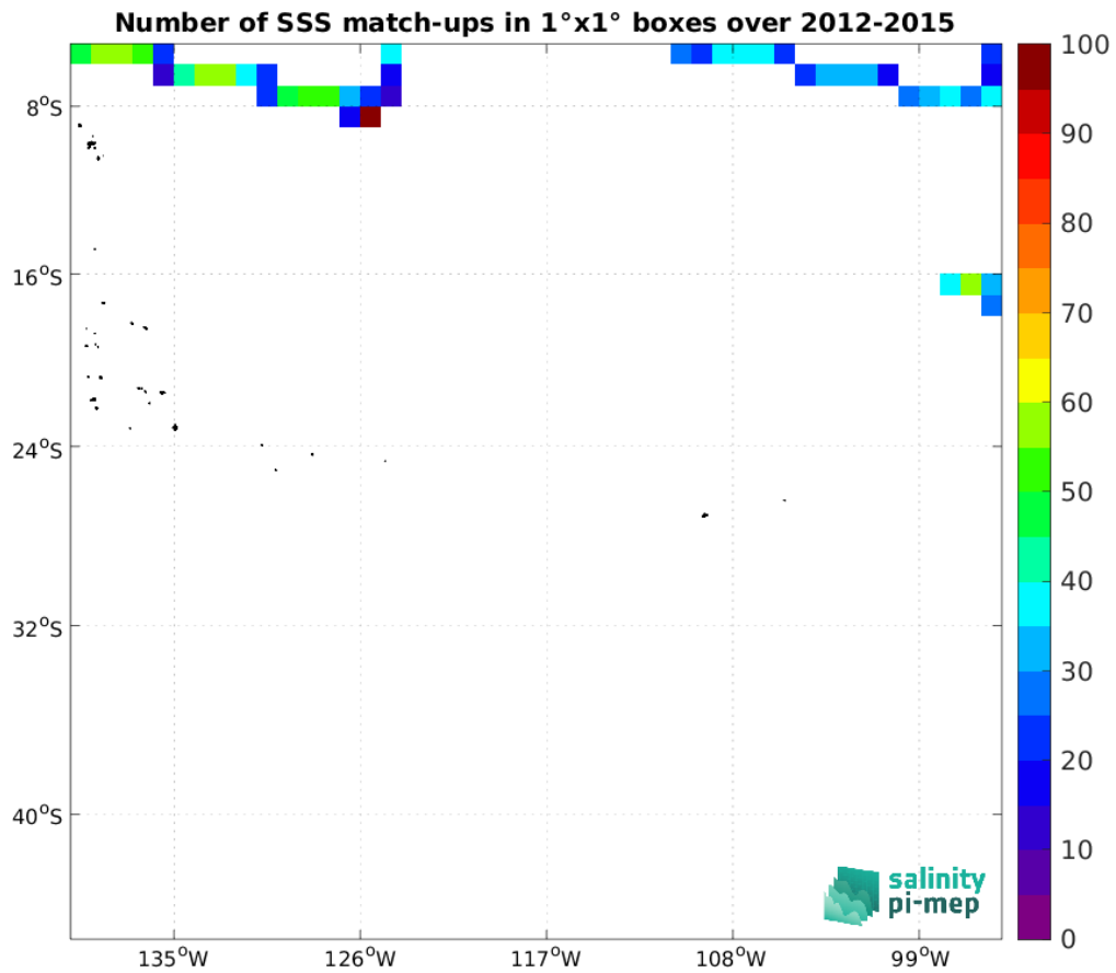
Figure 4: Number of SSS match-ups between TSG (SAMOS) SSS and the Aquarius SSS L3 CAP v5 - Monthly (JPL) SSS product for the OTT zone Pi-MEP region over 1^\circ \times 1^\circ boxes and for the full satellite product period.
