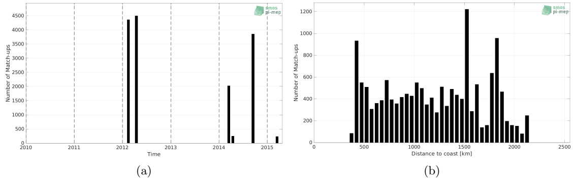
Figure 1: Number of match-ups between TSG (SAMOS) and Aquarius SSS L3 CAP v5 - Monthly (JPL) SSS as a function of time (a) and as function of the distance to coast (b) over the OTT zone Pi-MEP region and for the full satellite product period.
