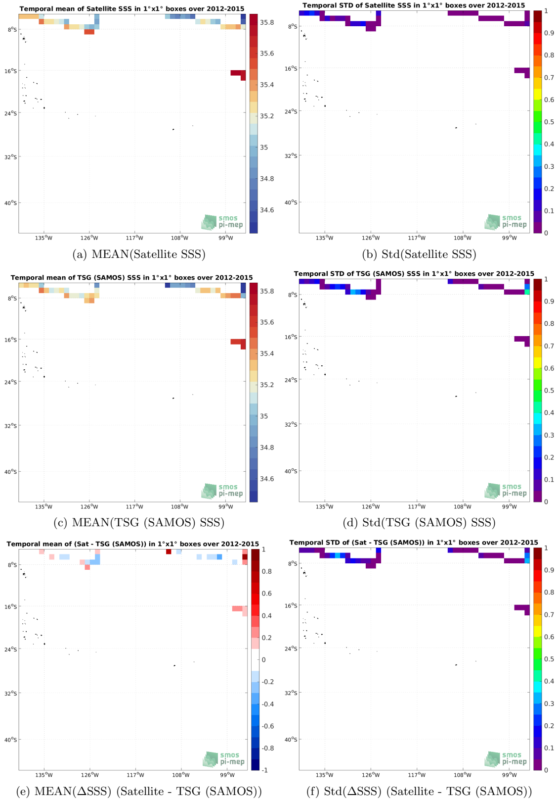
Figure 6: Temporal mean (left) and Std (right) of SSS from Aquarius SSS L3 CAP v5 - Monthly (JPL) (top), TSG (SAMOS) (middle), and of \Delta SSS (Satellite - TSG (SAMOS)). Only match-up pairs are used to generate these maps.
