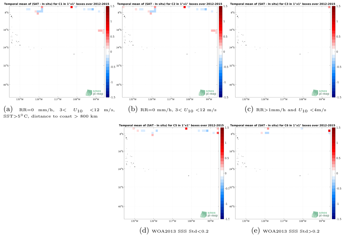
Figure 12: Temporal mean gridded over spatial boxes of size 1^\circ \times 1^\circ of \Delta SSS (Aquarius SSS L3 CAP v5 - Monthly (JPL) - TSG (SAMOS)) for 5 different subdatasets corresponding to: RR=0 mm/h, 3 < U_{10} < 12 m/s, SST > 5^\circ C , distance to coast > 800 km (a), RR=0 mm/h, 3 < U_{10} < 12 m/s (b), RR > 1 mm/h and U_{10} < 4 m/s (c), WOA2013 SSS Std < 0.2 (d), WOA2013 SSS Std > 0.2 (e).
