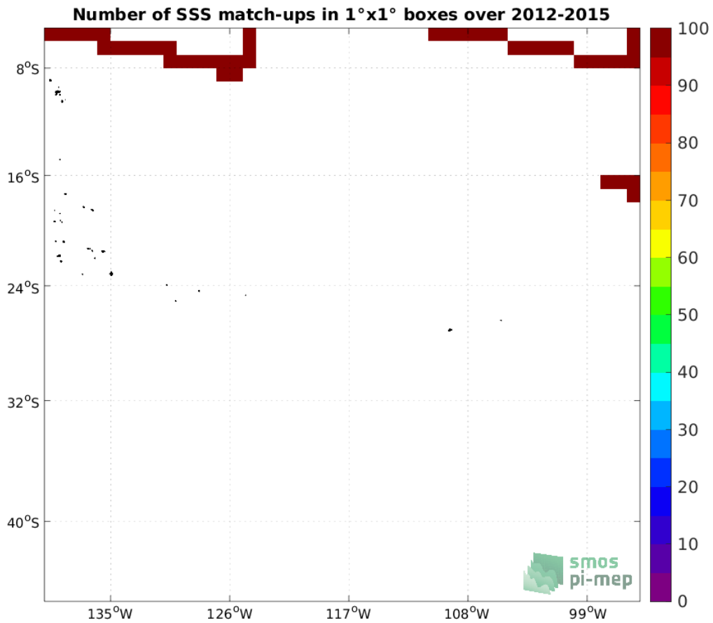
Figure 4: Number of SSS match-ups between TSG (SAMOS) SSS and the Aquarius SSS L3 CAP v5 - Monthly (JPL) SSS product for the OTT zone Pi-MEP region over 1°×1° boxes and for the full satellite product period.
