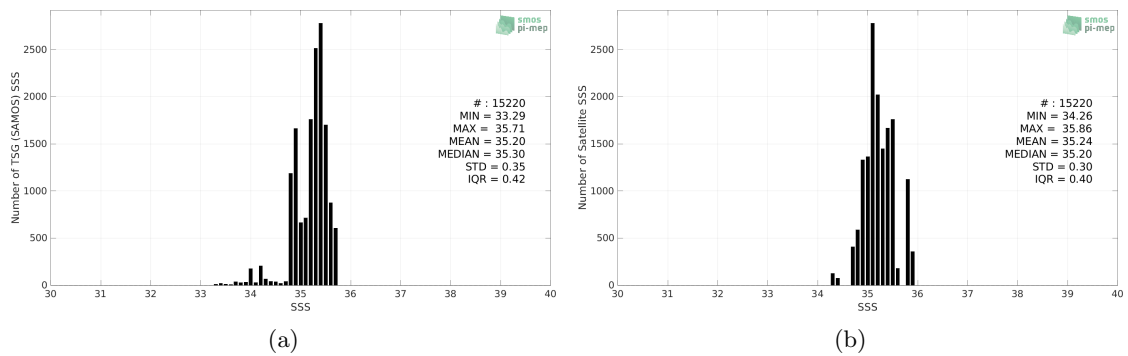
Figure 2: Histograms of SSS from TSG (SAMOS) (a) and Aquarius SSS L3 CAP v5 - Monthly (JPL) (b) considering all match-up pairs per bins of 0.1 over the OTT zone Pi-MEP region and for the full satellite product period.
