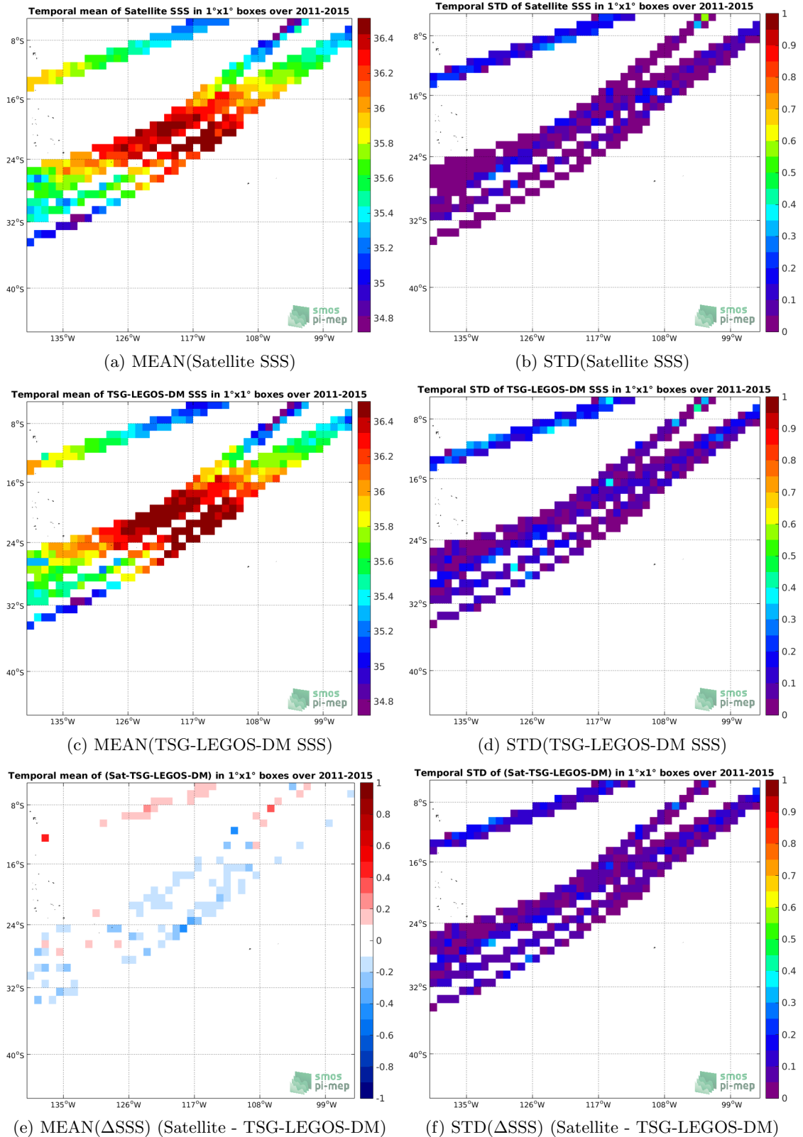
Figure 6: Temporal mean (left) and STD (right) of SSS from Aquarius-L3-JPL-V5-MONTHLY (top), TSG-LEGOS-DM (middle), and of \Delta SSS 8 (Satellite - TSG-LEGOS-DM). Only match-up pairs are used to generate these maps.
