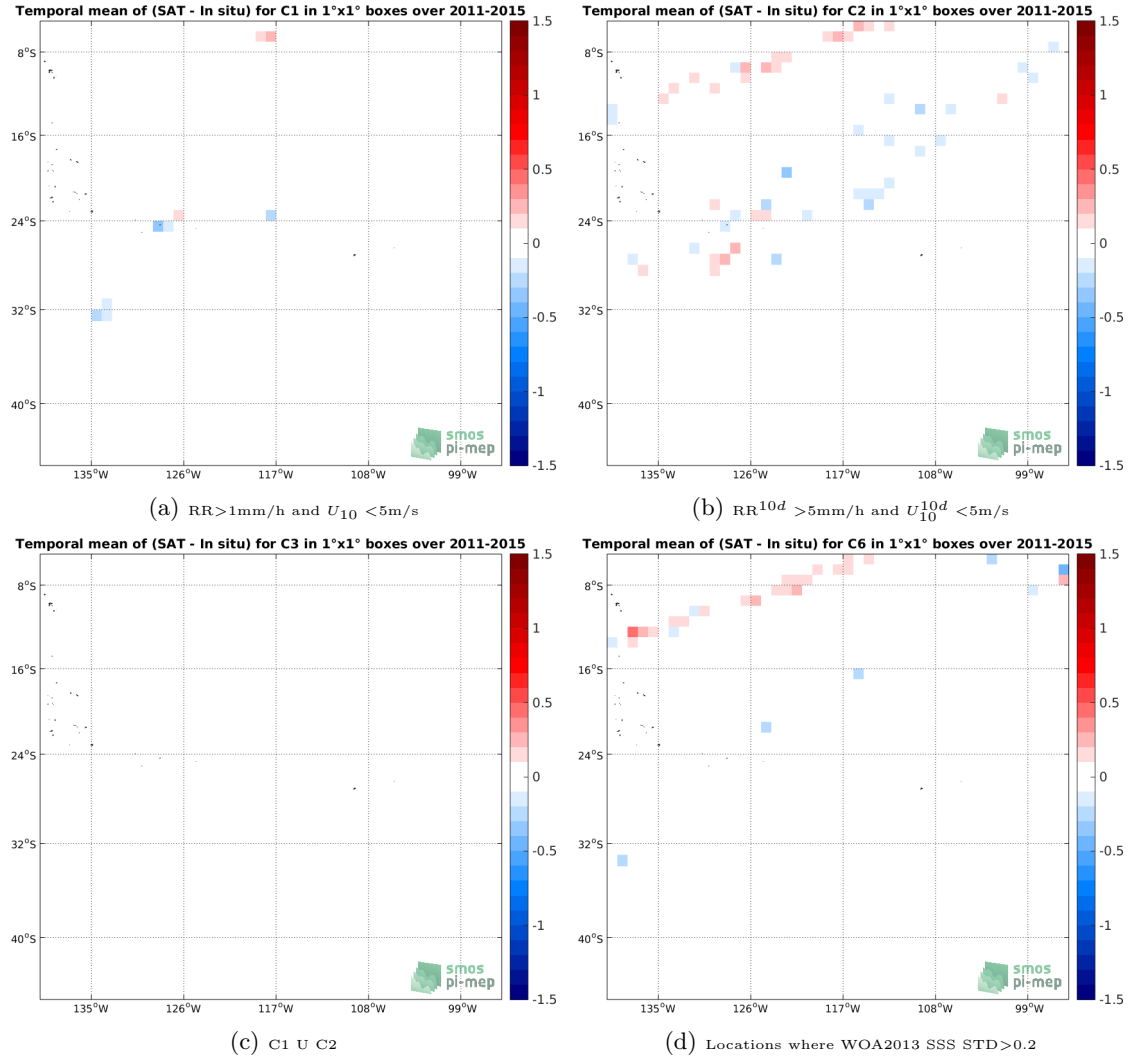
Figure 12: Temporal mean gridded over spatial boxes of size 1^\circ \times 1^\circ of \Delta SSS (Aquarius-L3-JPL-V5-MONTHLY - TSG-LEGOS-DM) for 4 different subdatasets corresponding to: RR > 1mm/h and U_{10} < 5m/s (a), RR^{10d} > 5mm/h and U_{10}^{10d} < 5m/s (b), C1 U C2 (c), Locations where WOA2013 SSS STD > 0.2 (d).
