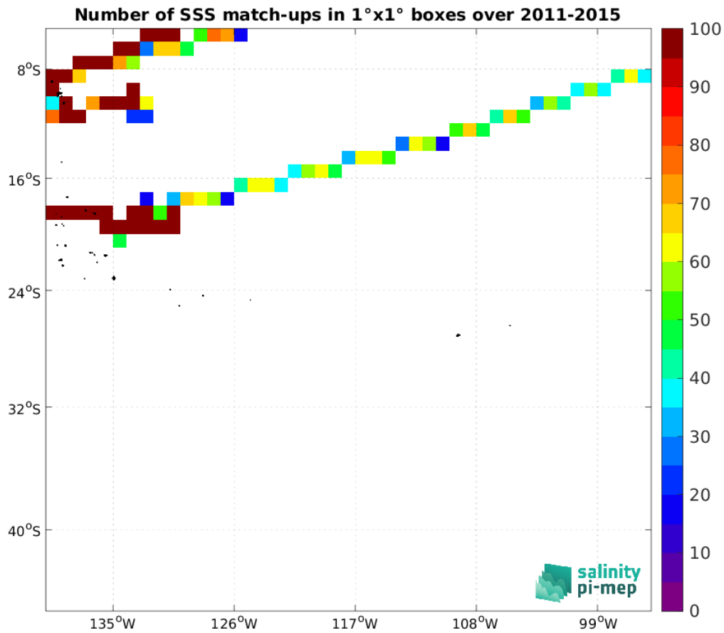
Figure 5: Number of SSS match-ups between TSG (GOSUD-Research-vessel) SSS and the Aquarius SSS L3 CAP v5 - Monthly (JPL) SSS product for the OTT zone Pi-MEP region over 1^\circ \times 1^\circ boxes and for the full satellite product period.
