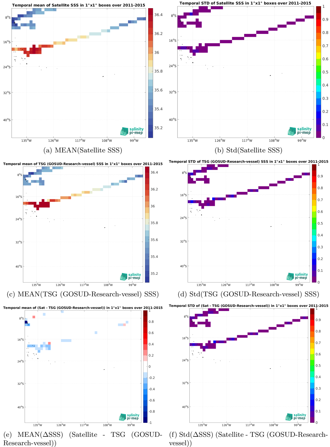
Figure 7: Temporal mean (left) and Std (right) of SSS from Aquarius SSS L3 CAP v5 - Monthly (JPL) (top), TSG (GOSUD-Research-vessel) (middle), and of \Delta SSS (Satellite - TSG (GOSUD-Research-vessel)). Only match-up pairs are used to generate these maps.
