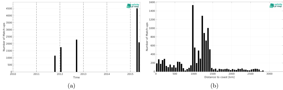
Figure 2: Number of match-ups between TSG (GOSUD-Research-vessel) and Aquarius SSS L3 CAP v5 - Monthly (JPL) SSS as a function of time (a) and as function of the distance to coast (b) over the OTT zone Pi-MEP region and for the full satellite product period.
