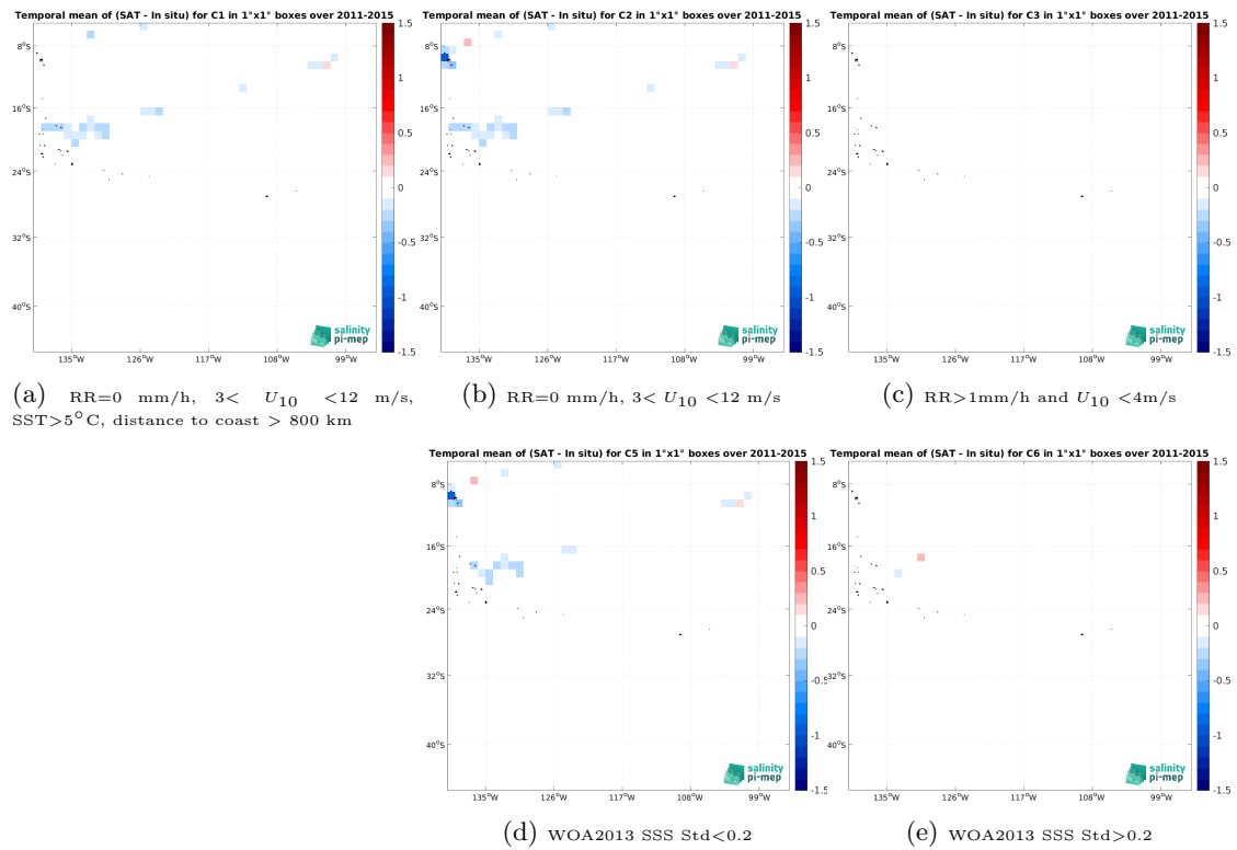
Figure 14: Temporal mean gridded over spatial boxes of size 1^\circ \times 1^\circ of \Delta SSS (Aquarius SSS L3 CAP v5 - Monthly (JPL) - TSG (GOSUD-Research-vessel)) for 5 different subdatasets corresponding to:RR=0 mm/h, 3 < U_{10} < 12 m/s, SST >5^\circ\text{C} , distance to coast > 800 km (a), RR=0 mm/h, 3 < U_{10} < 12 m/s (b), RR >1 mm/h and U_{10} < 4 m/s (c), WOA2013 SSS Std <0.2 (d), WOA2013 SSS Std >0.2 (e).
