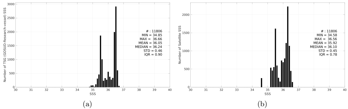
Figure 3: Histograms of SSS from TSG (GOSUD-Research-vessel) (a) and Aquarius SSS L3 CAP v5 - Monthly (JPL) (b) considering all match-up pairs per bins of 0.1 over the OTT zone Pi-MEP region and for the full satellite product period.
