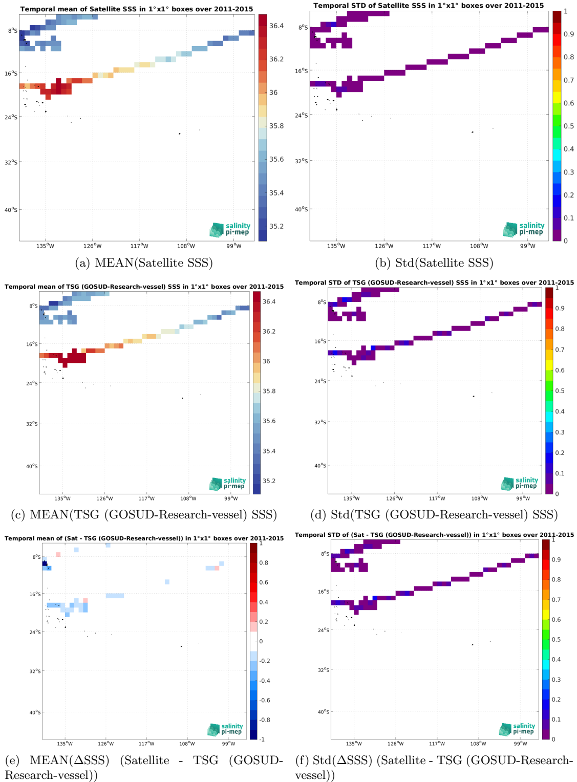
Figure 6: Temporal mean (left) and Std (right) of SSS from Aquarius SSS L3 CAP v5 - Monthly (JPL) (top), TSG (GOSUD-Research-vessel) (middle), and of \Delta SSS (Satellite - TSG (GOSUD-Research-vessel)). Only match-up pairs are used to generate these maps.
