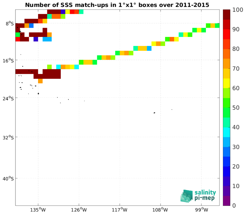
Figure 4: Number of SSS match-ups between TSG (GOSUD-Research-vessel) SSS and the Aquarius SSS L3 CAP v5 - Monthly (JPL) SSS product for the OTT zone Pi-MEP region over 1^{\circ} \times 1^{\circ} boxes and for the full satellite product period.
